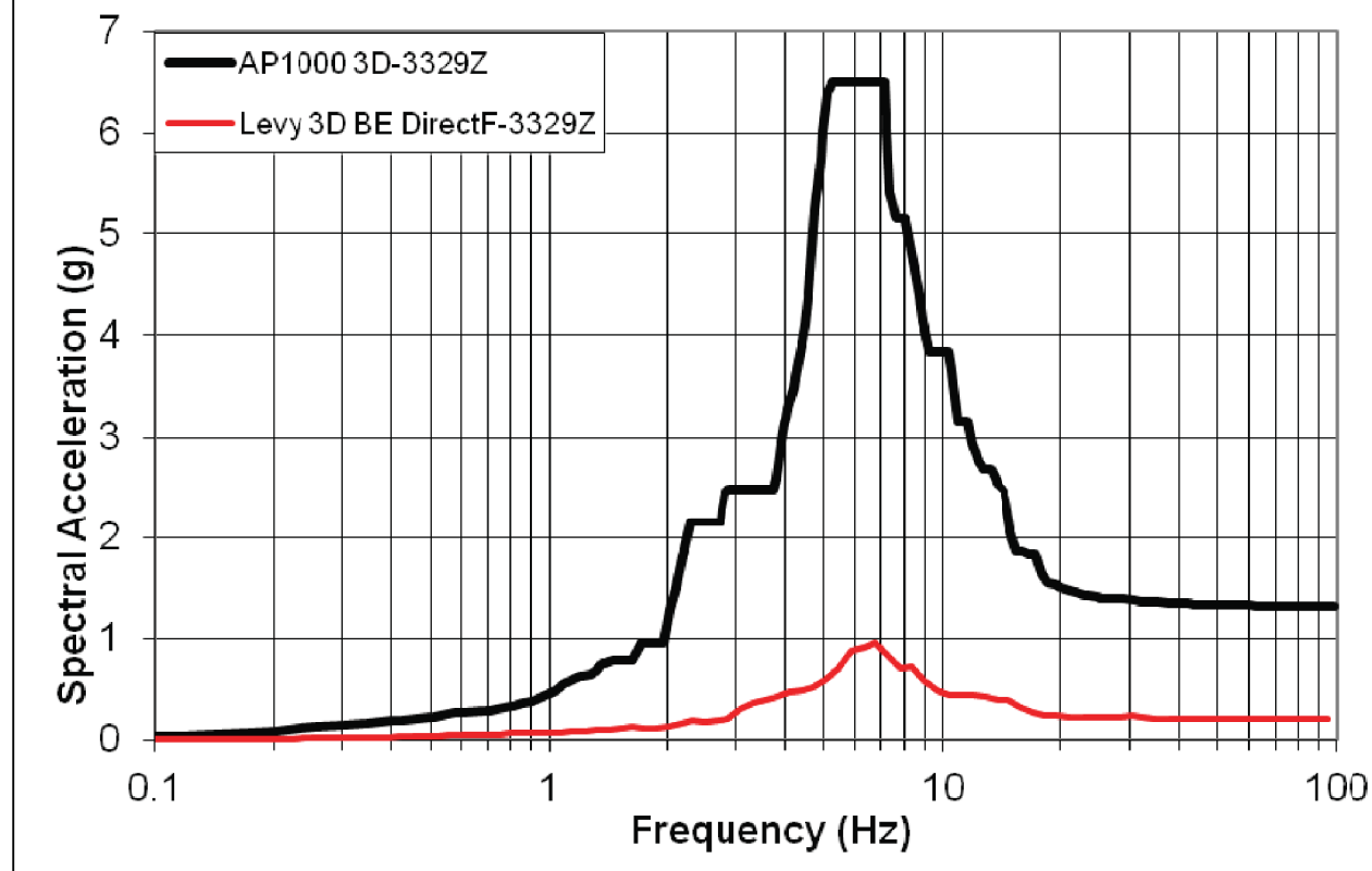
LEVY 3D SSI DIRECT FACTORED Z BE (3329)
