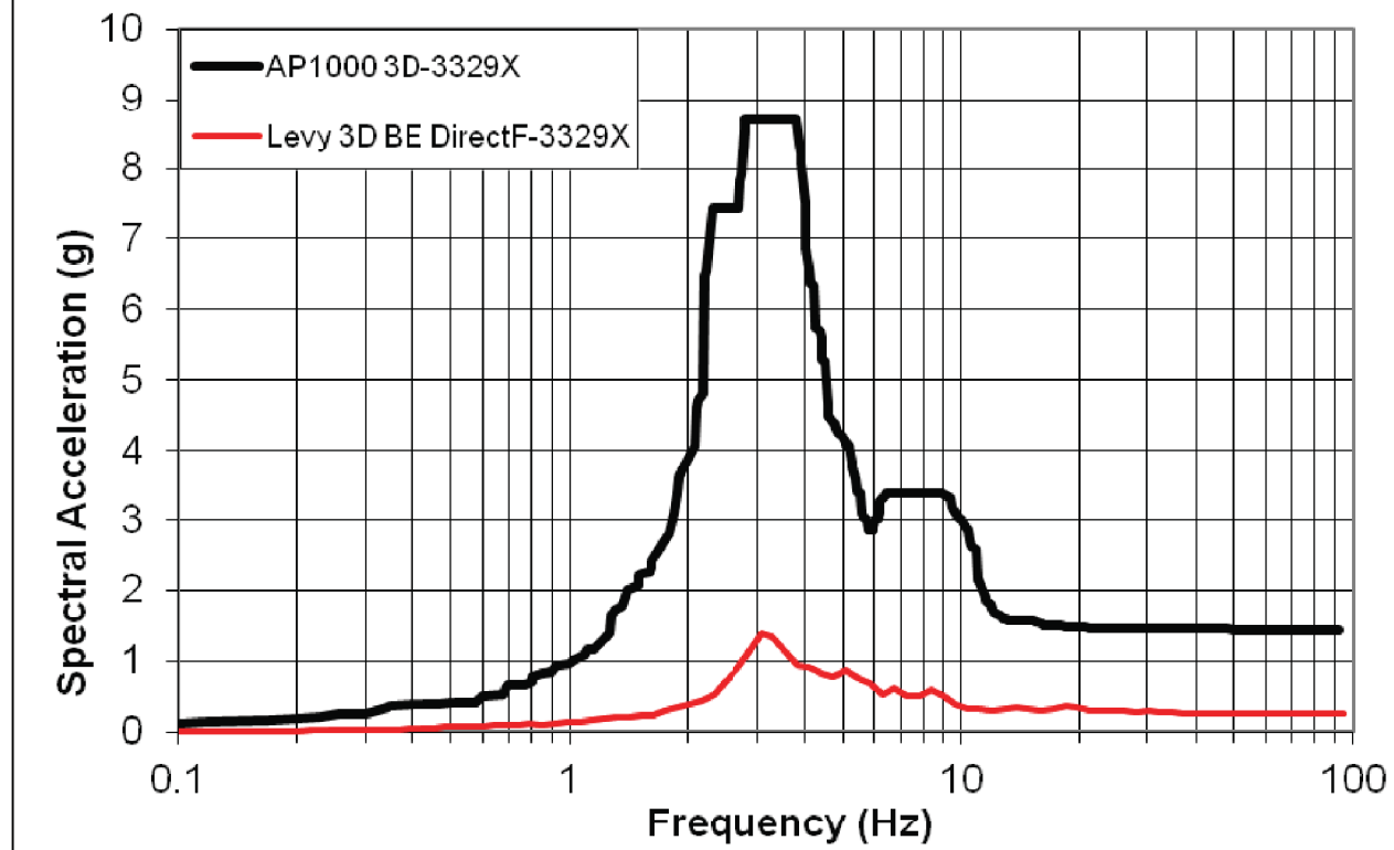
LEVY 3D SSI DIRECT FACTORED X BE (3329)
