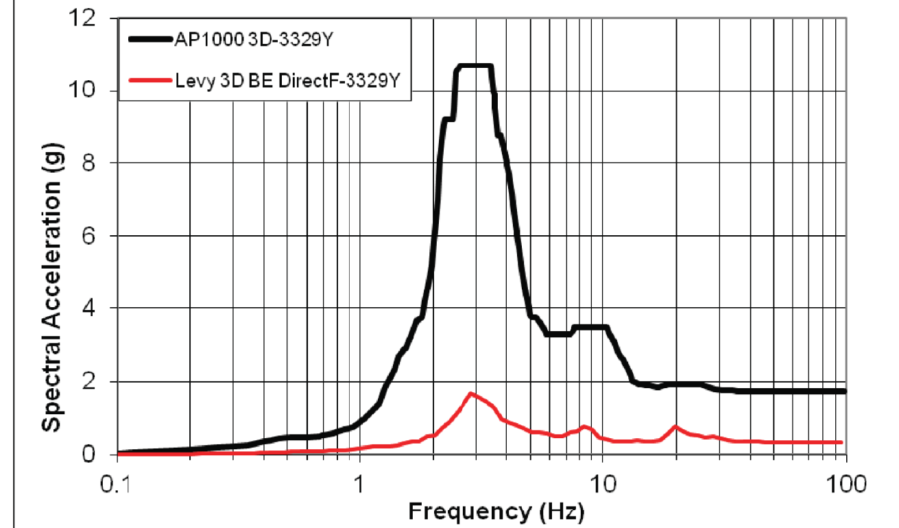
LEVY 3D SSI DIRECT FACTORED Y BE (3329)
