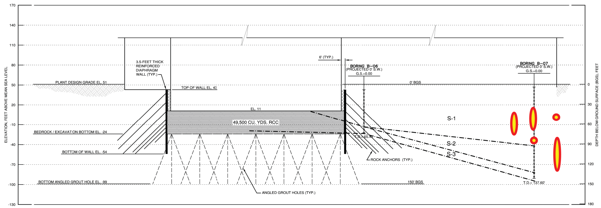
SECTION A
