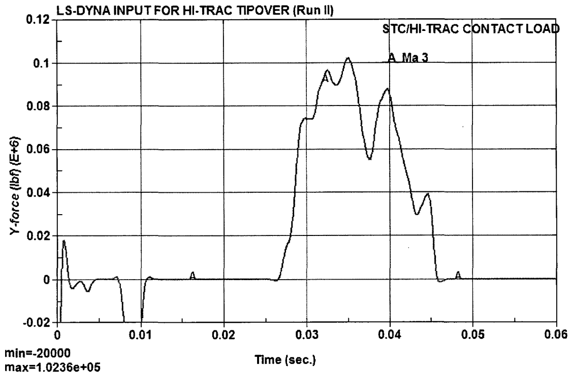
Figure 6.2.13 Contact Force on the HI-TRAC (Governing Case)
