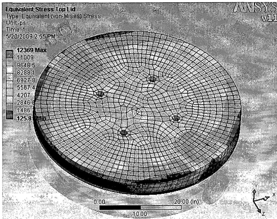
Figure 6.2.2 Resulting Stress from STC Lifting
