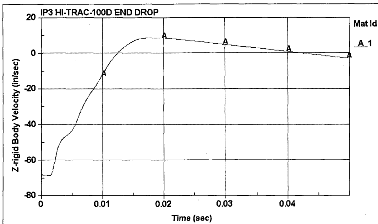
Figure 6.2.4 HI-TRAC 100D Transfer Cask Impact Velocity Time History
