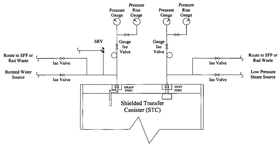
Figure 10.1: Example P&I Diagram for Pressure Monitoring System
