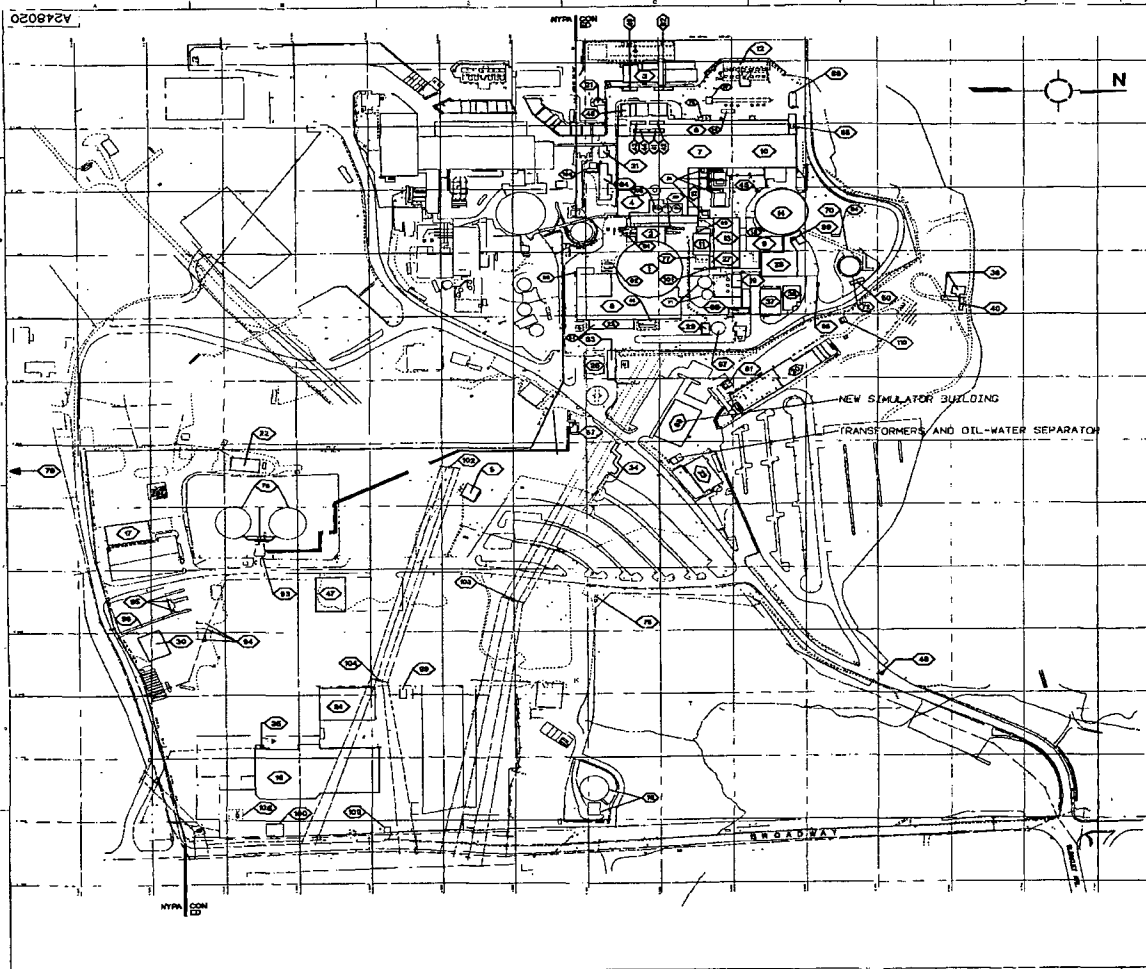
FIGURE 7.4.3 SITE MAP (BUILDING IDENTIFICATION PLAN) SHOWING TRUE NORTH
