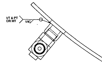
DETAIL P
