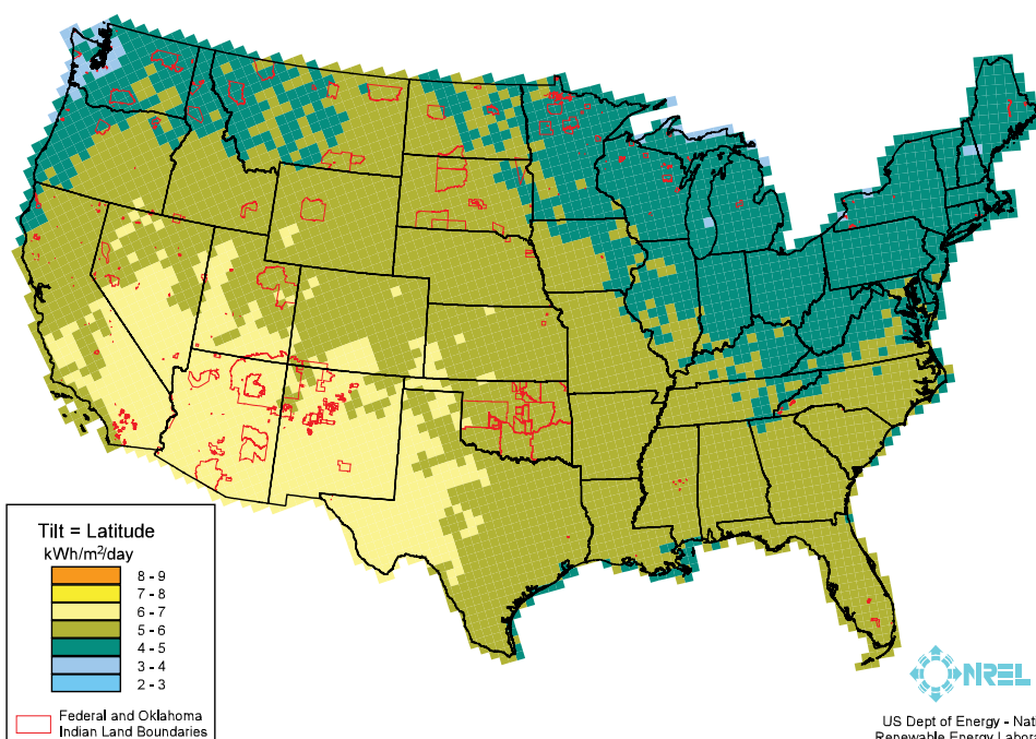
Figure 5: Solar photovoltaic resource potential. 11
