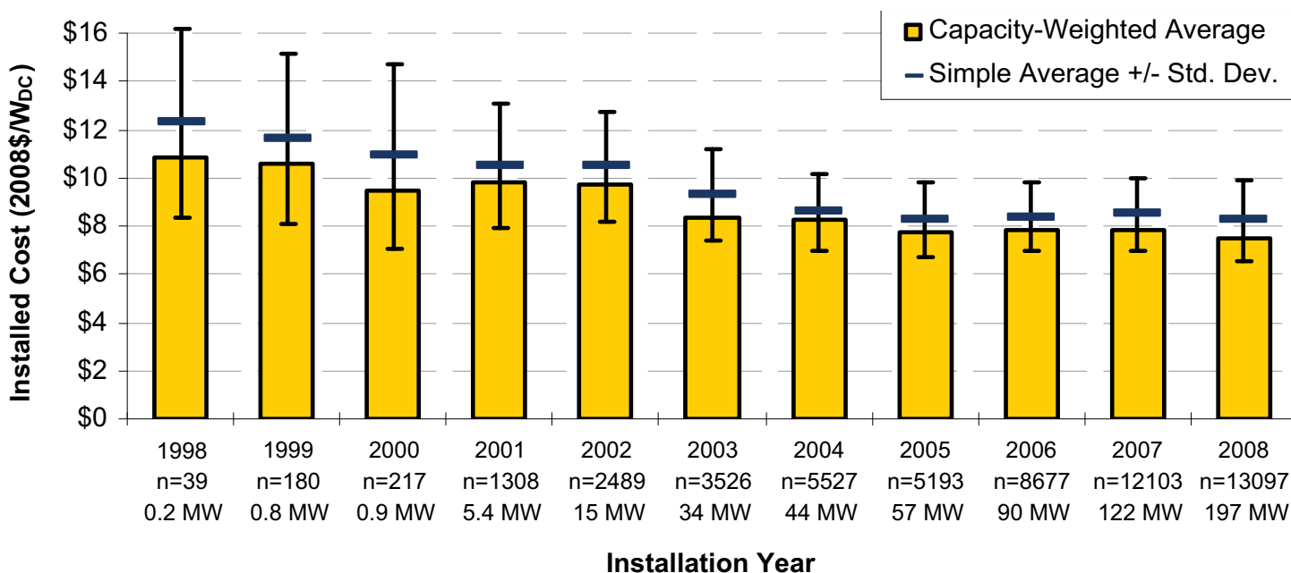
Figure 2: Falling installed cost for solar PV, 1998–2008 (Wiser, 2009).
