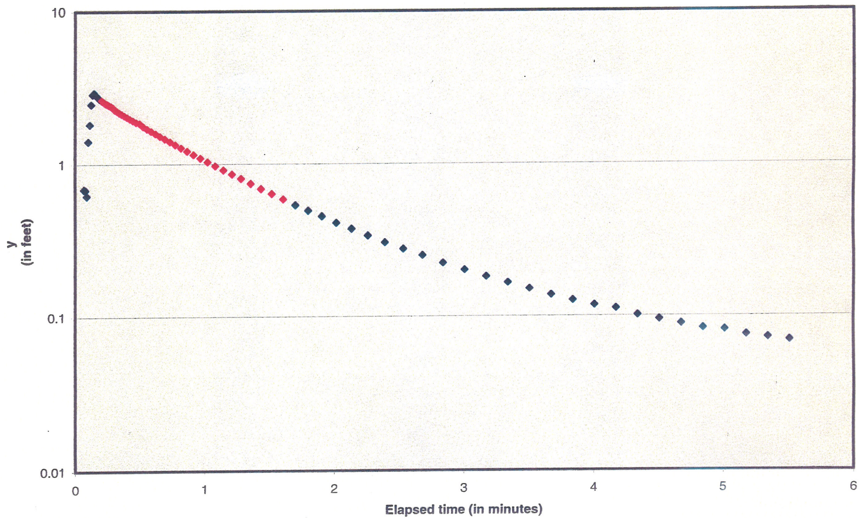
OW-946 (slug-out2) Recovery vs. Time
