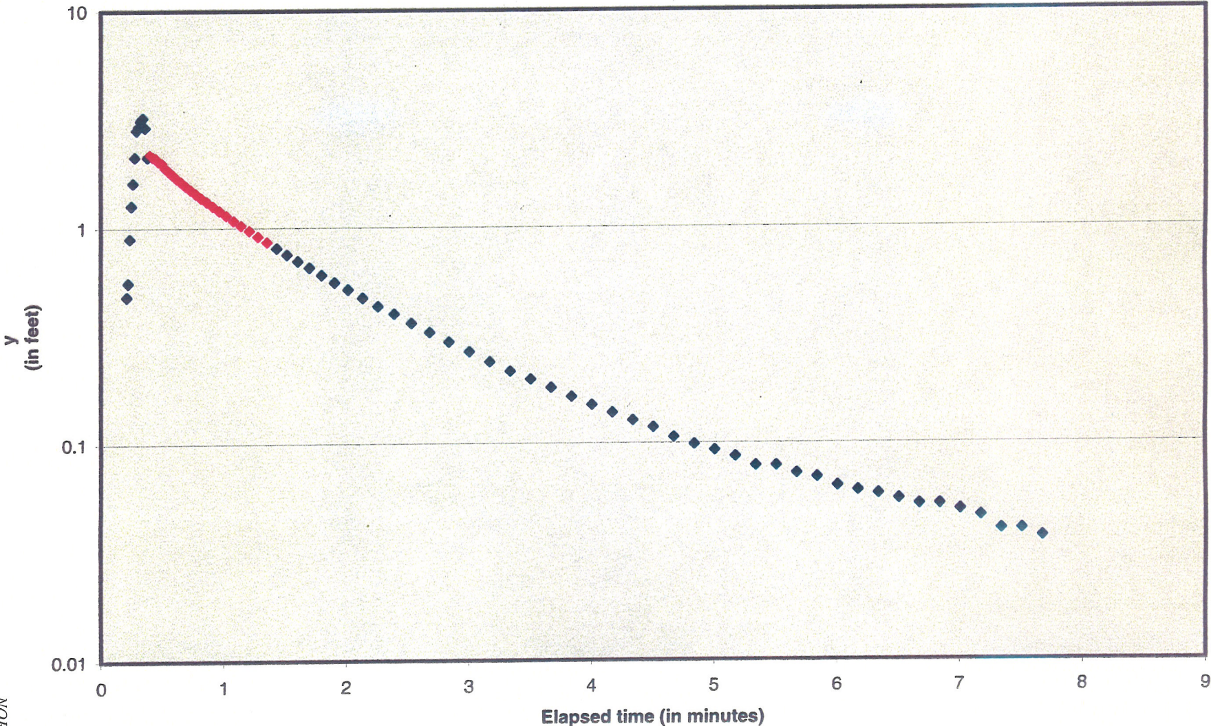
OW-946 (slug-in2) Recovery vs. Time
