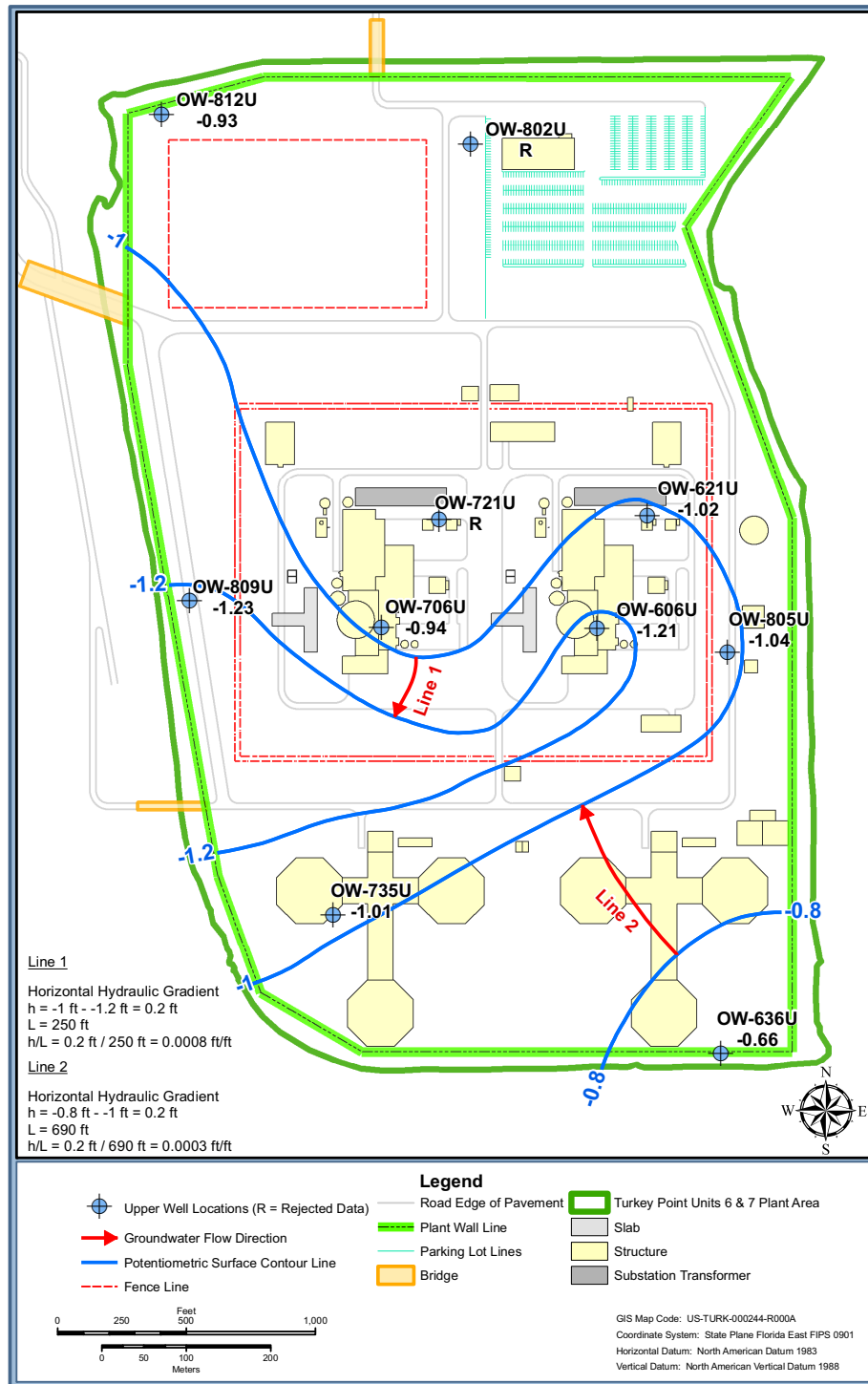
Figure 2.4.12-248 Biscayne Aquifer Potentiometric Surface Map, Upper Monitoring Interval, July 15, 2009 (Sheet 1 of 2) High Tide
