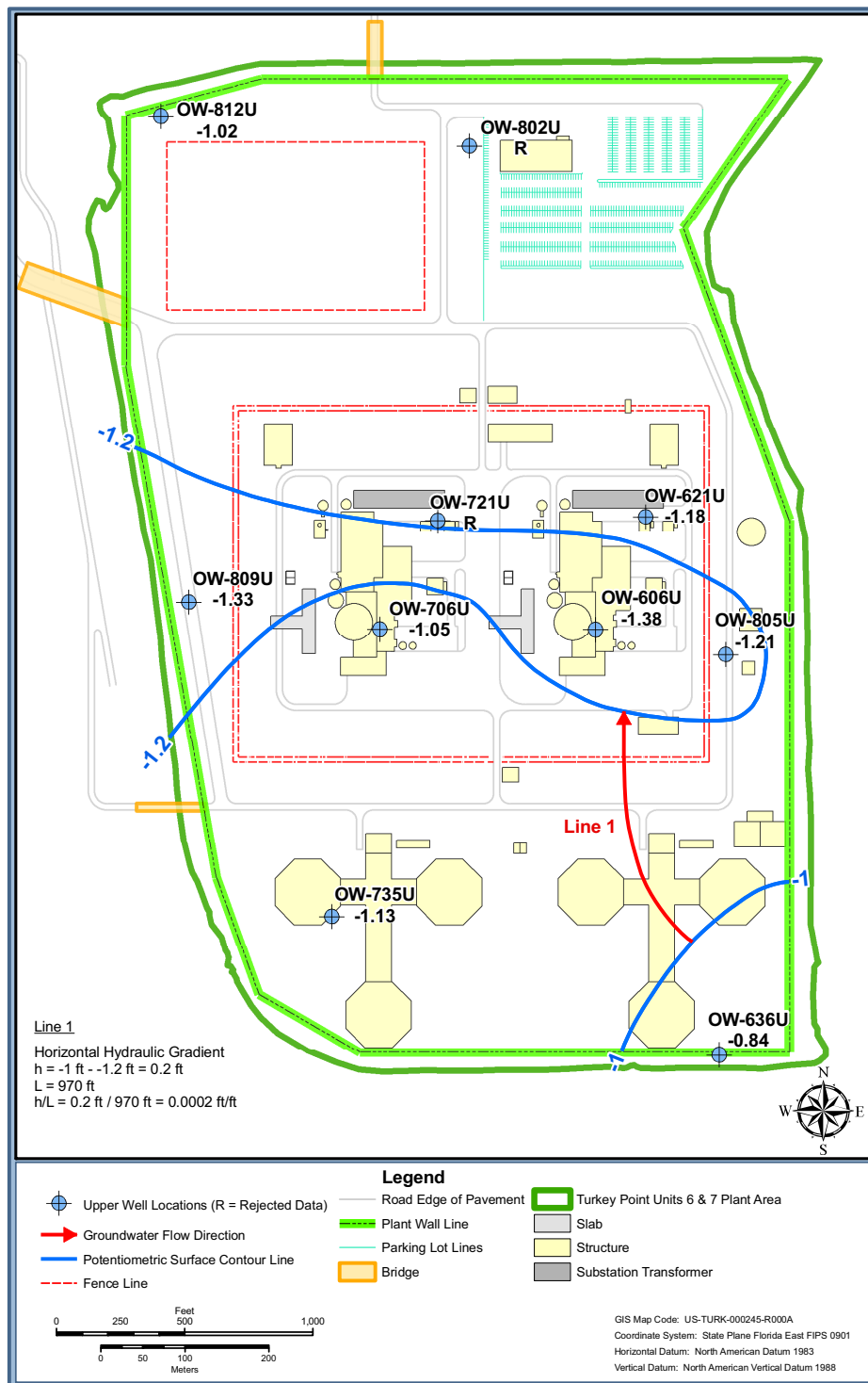
Figure 2.4.12-248 Biscayne Aquifer Potentiometric Surface Map, Upper Monitoring Interval, July 15, 2009 (Sheet 2 of 2) Low Tide
