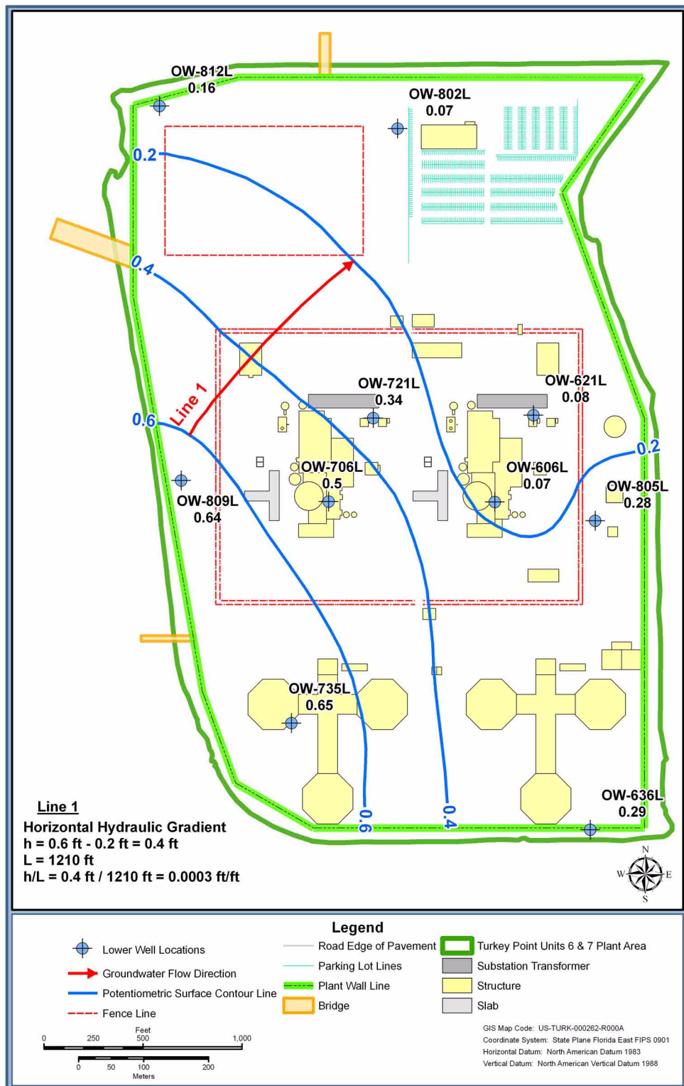
Figure 2.4.12-253 Biscayne Aquifer Potentiometric Surface Map, Lower Monitoring Interval, June 15, 2010 (Sheet 2 of 2) Low Tide
