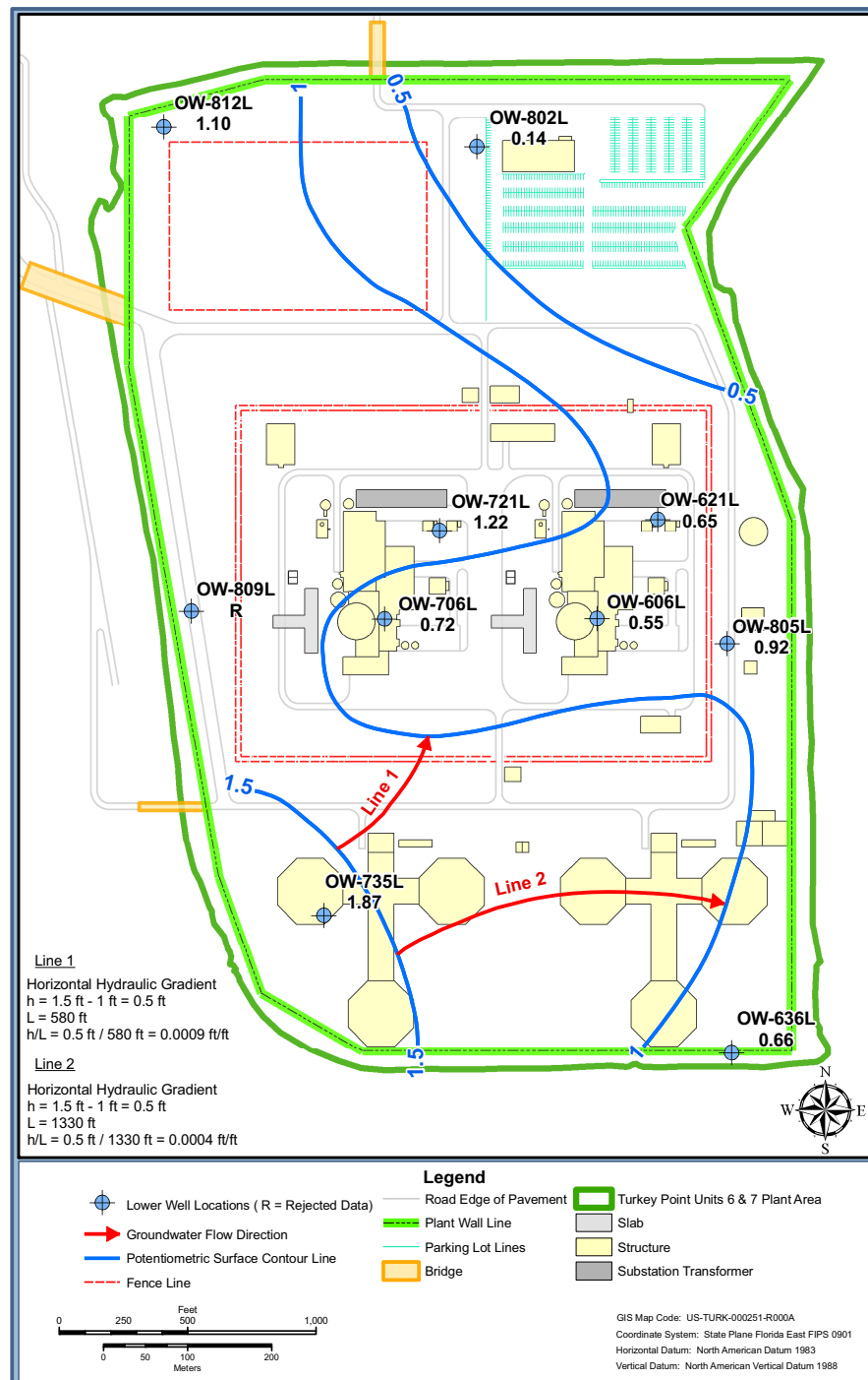
Figure 2.4.12-251 Biscayne Aquifer Potentiometric Surface Map, Lower Monitoring Interval, January 15, 2010 (Sheet 2 of 2) Low Tide
