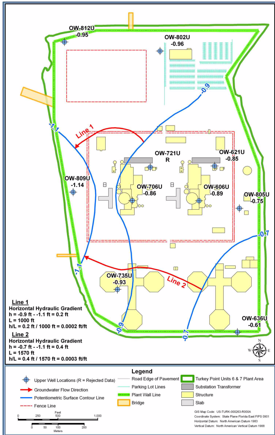
Figure 2.4.12-252 Biscayne Aquifer Potentiometric Surface Map, Upper Monitoring Interval, June 15, 2010 (Sheet 1 of 2) High Tide
