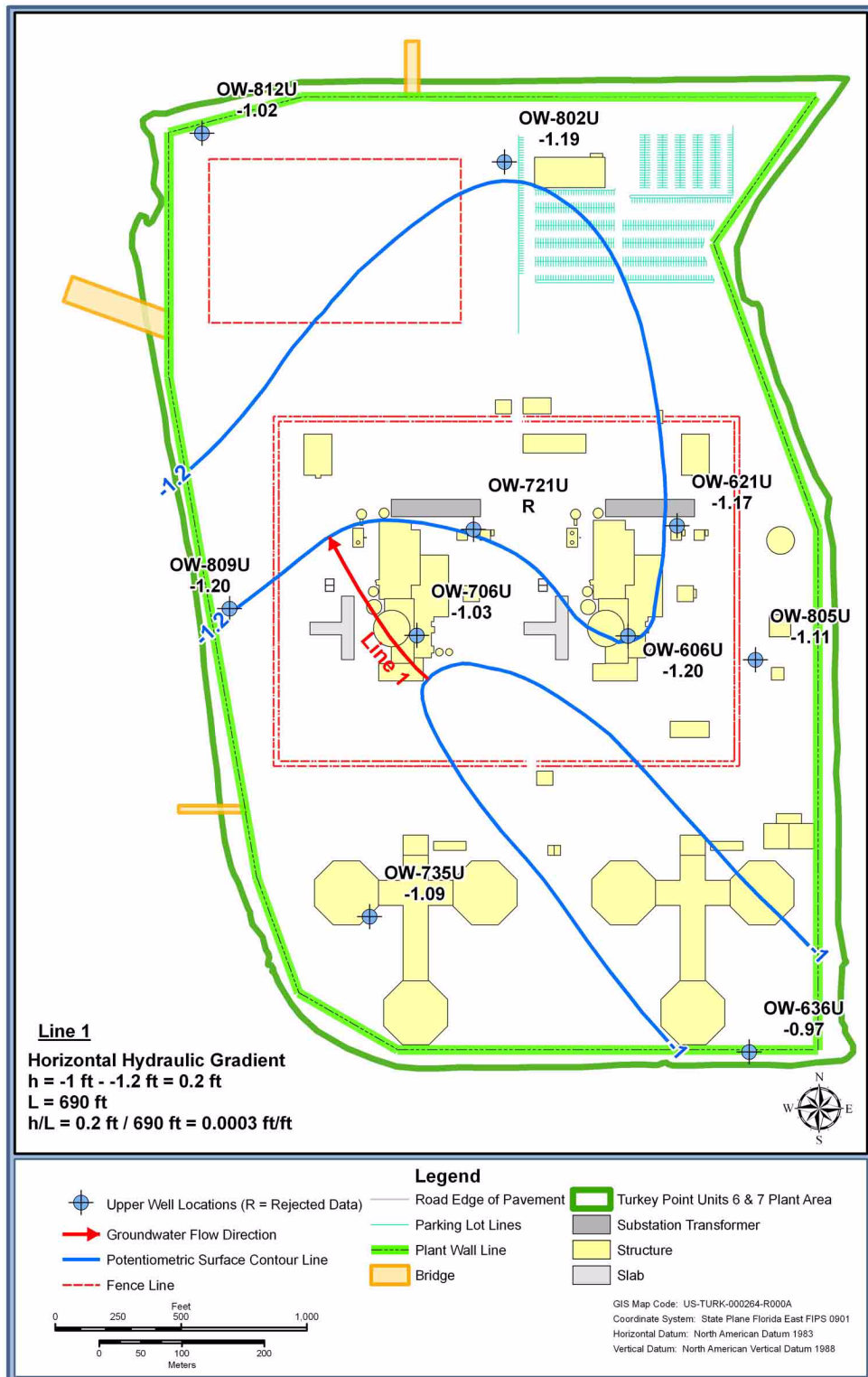
Figure 2.4.12-252 Biscayne Aquifer Potentiometric Surface Map, Upper Monitoring Interval, June 15, 2010 (Sheet 2 of 2) Low Tide
