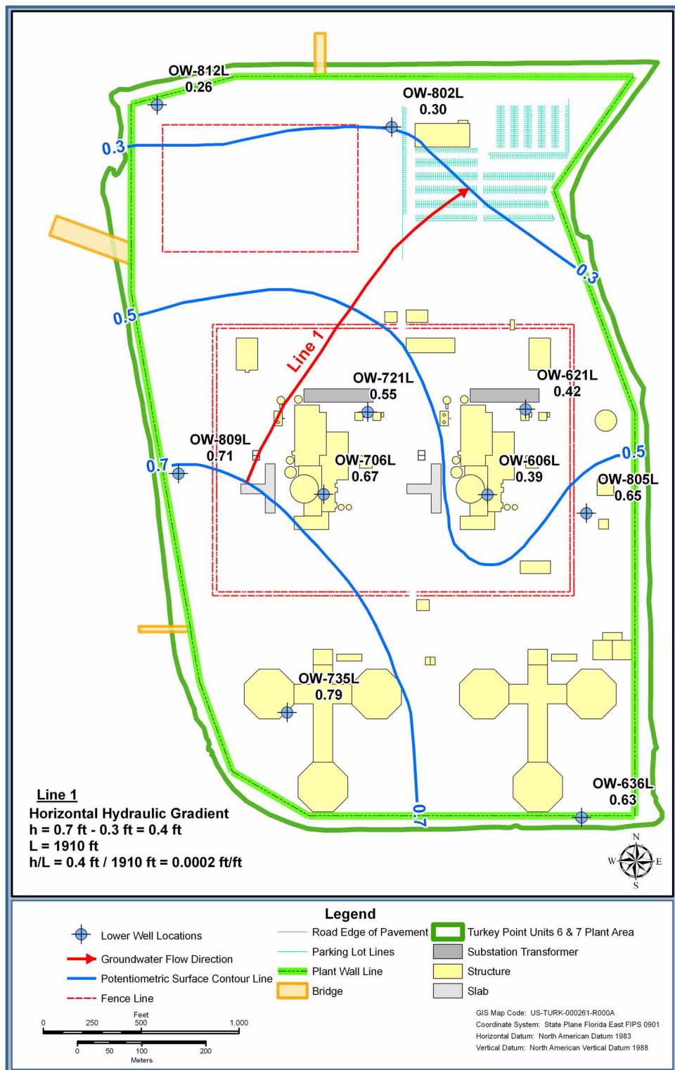
Figure 2.4.12-253 Biscayne Aquifer Potentiometric Surface Map, Lower Monitoring Interval, June 15, 2010 (Sheet 1 of 2) High Tide
