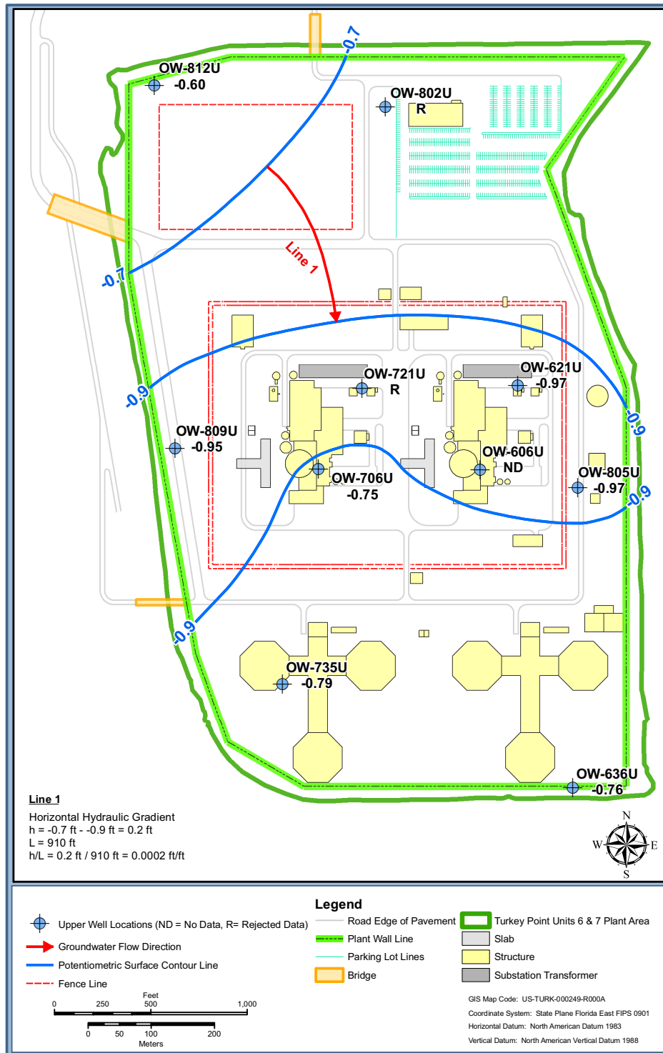
Figure 2.4.12-250 Biscayne Aquifer Potentiometric Surface Map, Upper Monitoring Interval, January 15, 2010 (Sheet 2 of 2) Low Tide
