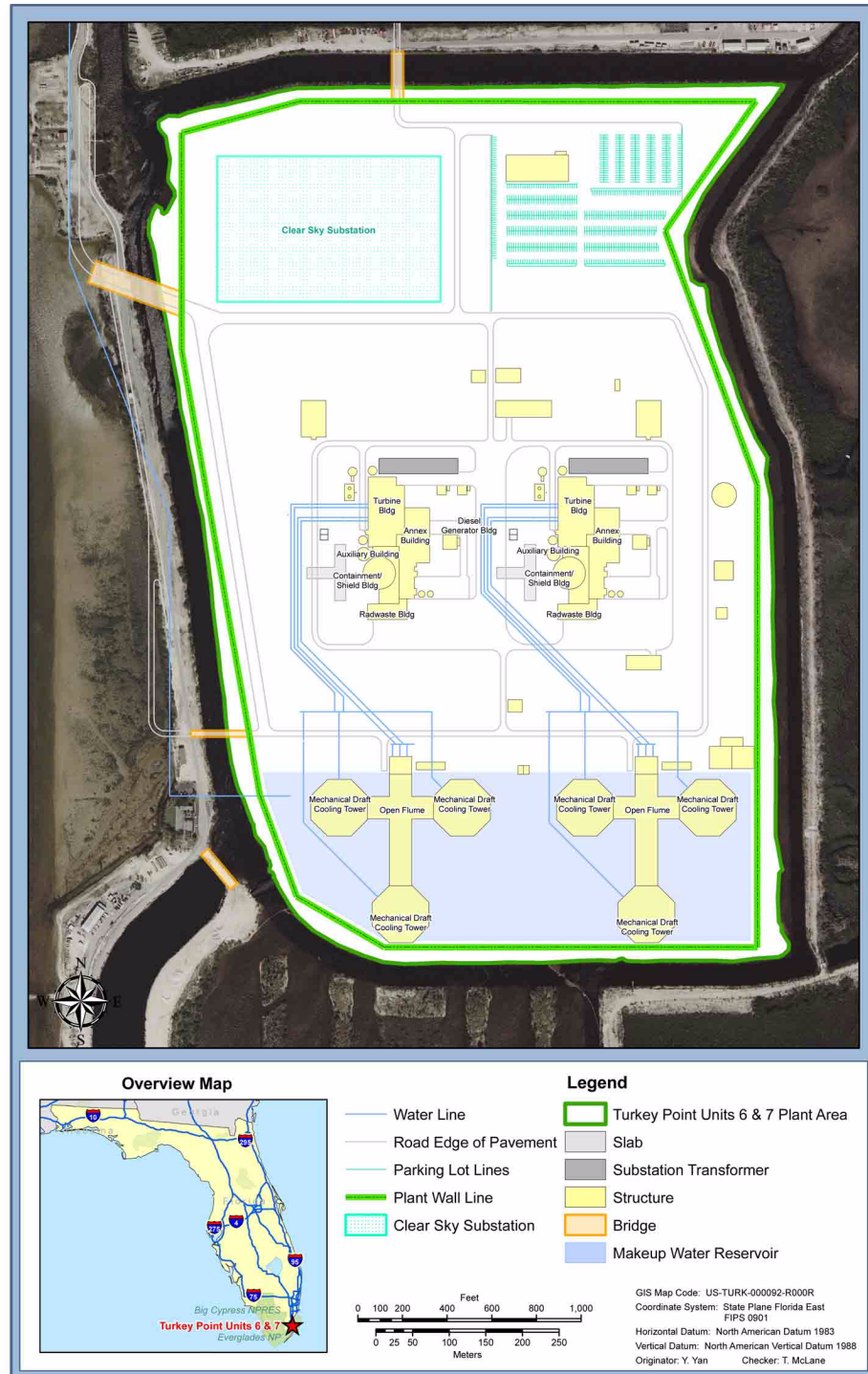
Figure 2.1-205 Principal Plant Structures within the Site Area
