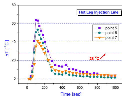
Fig. 11. Temperature changes with time at points 5, 6 and 7.
