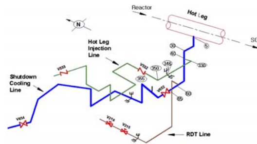
Fig. 1. Schematic diagram of the branch lines connected to the RCS piping.
