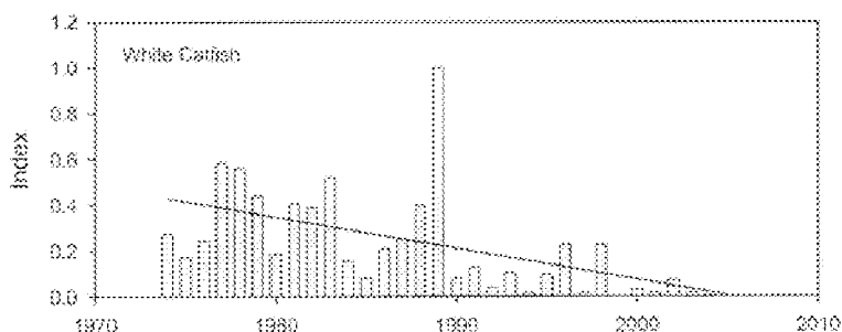
Figure 2: The standardised juvenile index for white catfish in the Hudson, showing a decreasing trend though time. The trend is significant ( a = -0.0136 , b = 27.216 , F = 14.0414 , p = 0.0008 ) (Seaby and Henderson, 2007)
