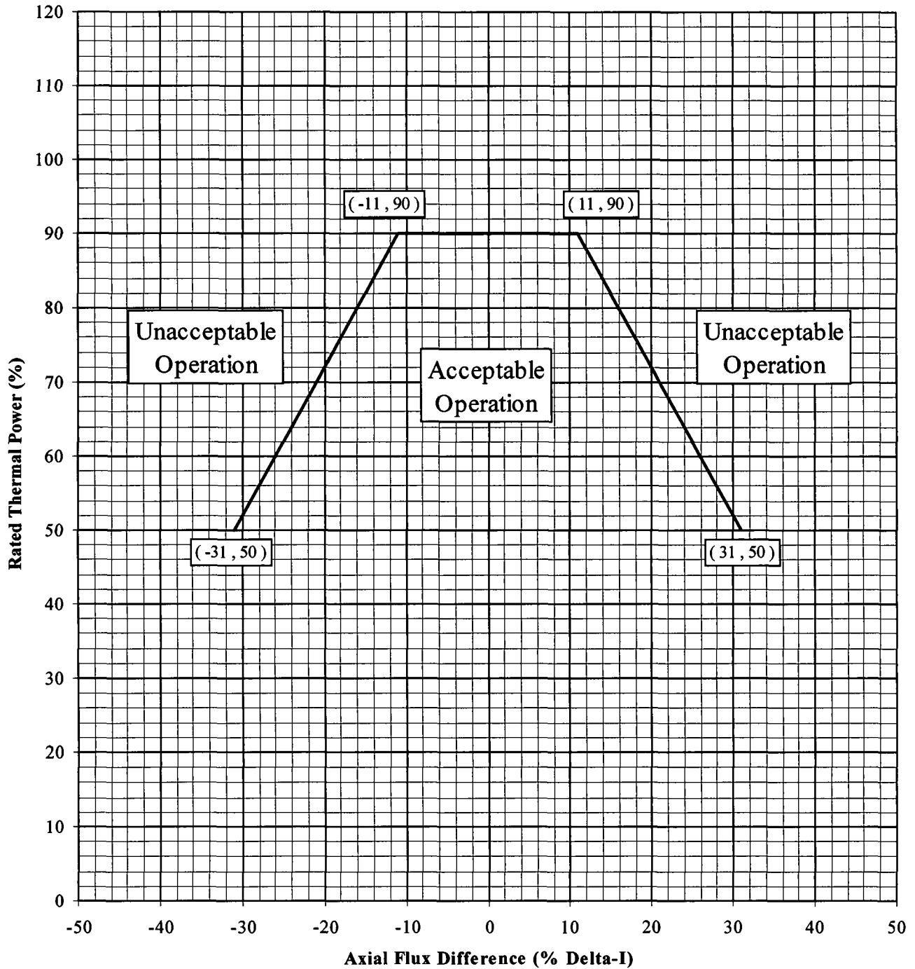
AFD Limits versus Power Level
