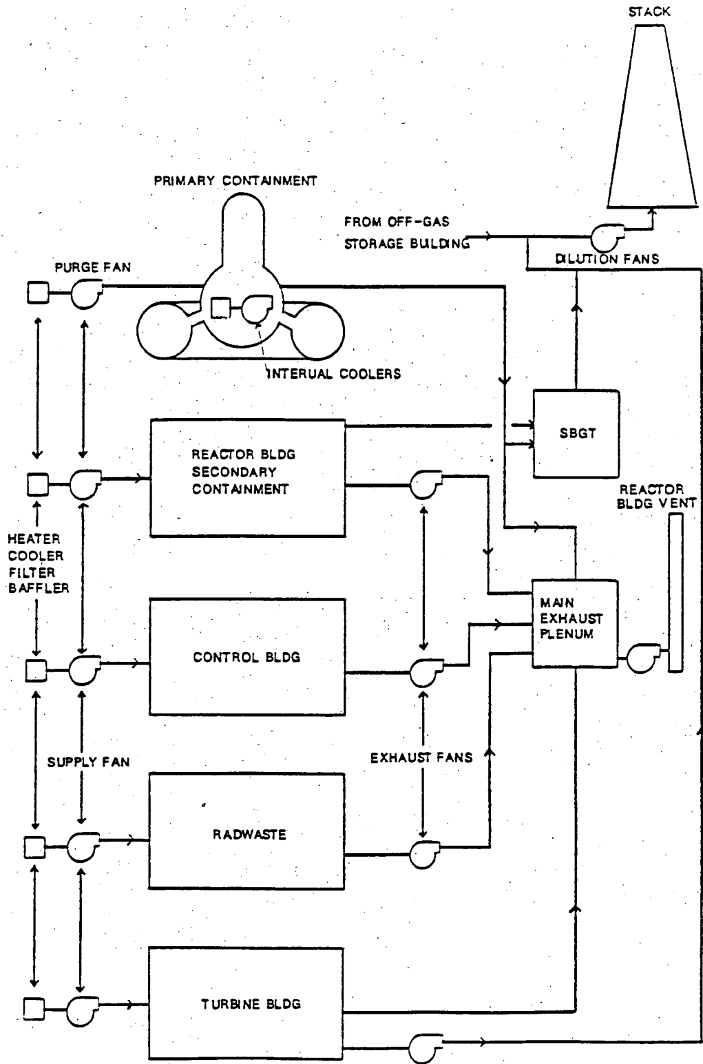
VENTILATION SYSTEM
