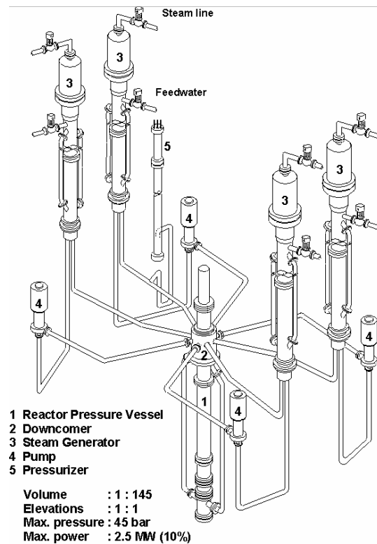
Figure 1: PKL facility
