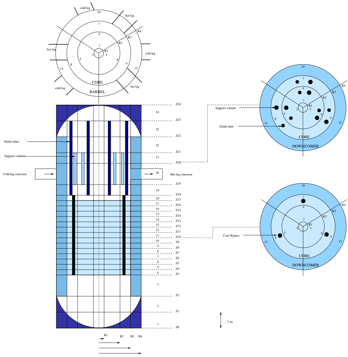
Figure 16: Nodalization of the TRACE model of 3D VESSEL
