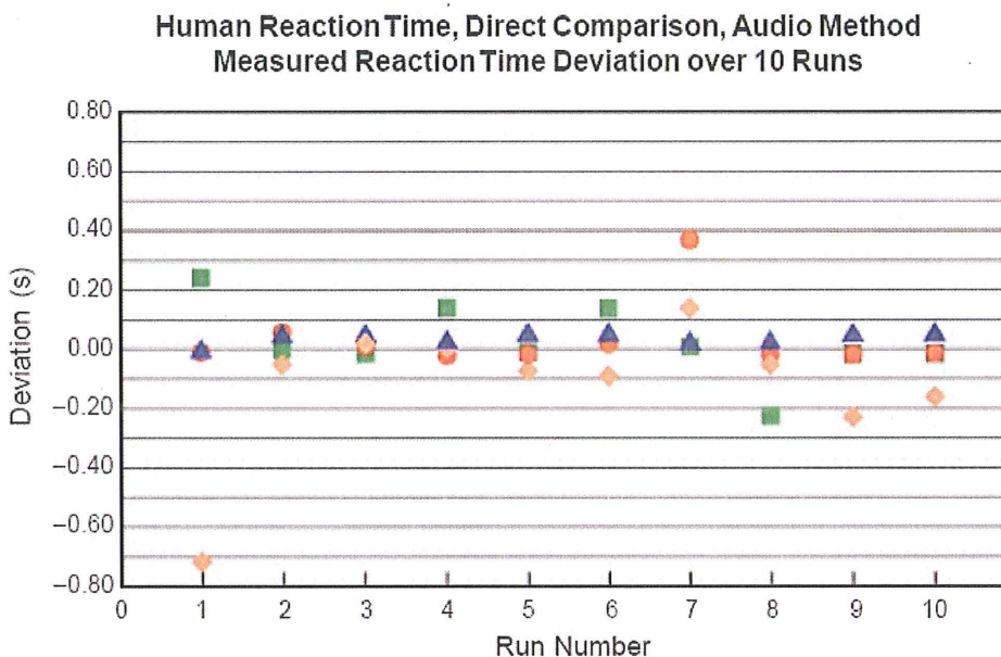
Figure 14. Reaction time measurements (four operators, ten runs each) for the Direct Comparison Method.
