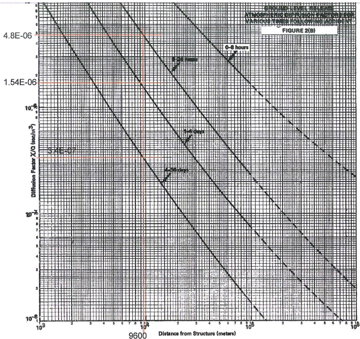
Figure 5.4: Detail from Regulatory Guide 1.4 (Reference 12.a.9) showing development of X/Q = 4.8E-06 sec/m 3 at a distance of 6 miles (9600 m) for the 8 to 24 hour line, of X/Q = 1.54E-06 sec/m 3 at a distance of 6 miles for the 1 to 4 day line, and of X/Q = 3.4E-07 sec/m 3 at a distance of 6 miles for the 4 to 30 day line.
