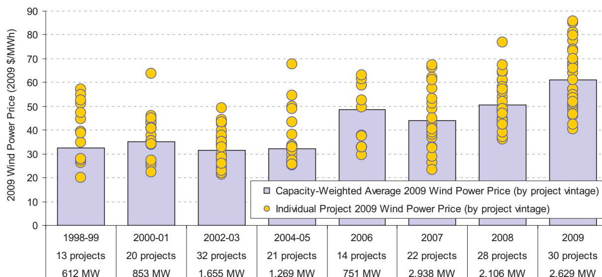
Figure 20. 2009 Wind Power Prices by Project Vintage
