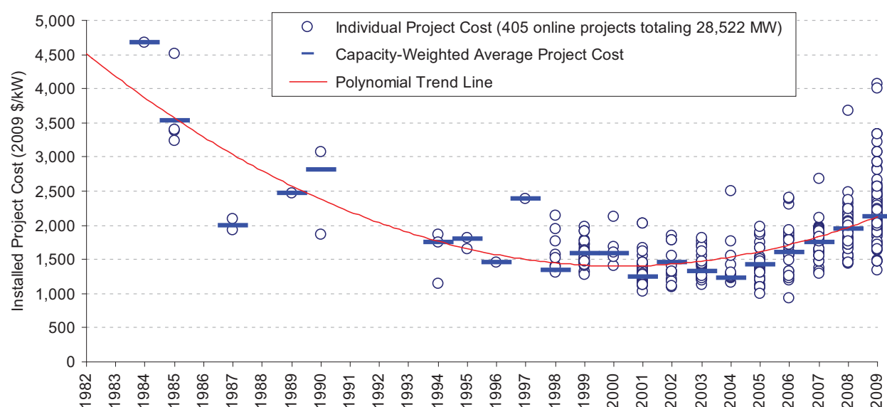
Figure 27. Installed Wind Power Project Costs Over Time
