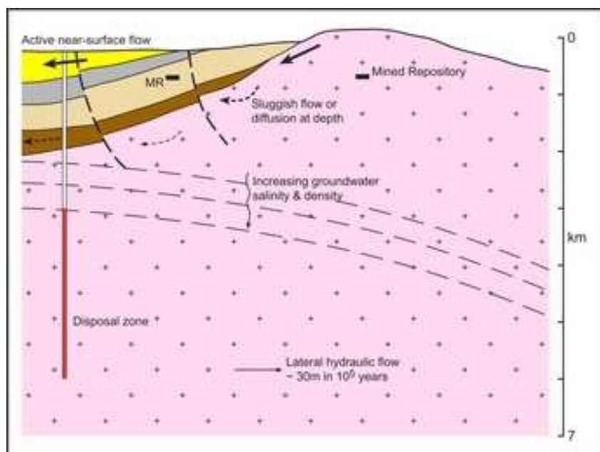
Figure 13. Deep Borehole Disposal Concept 46
