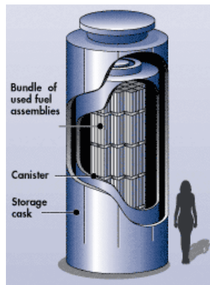
Figure 4. Dry Storage System
