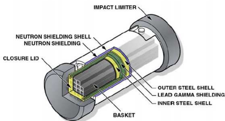
Generic Rail Cask for Spent Fuel
