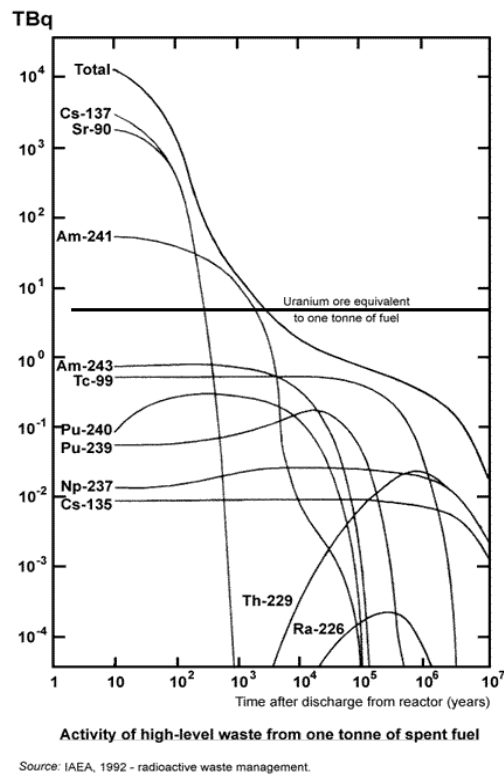
Figure 8. Radioactive Decay of Typical Spent Fuel
