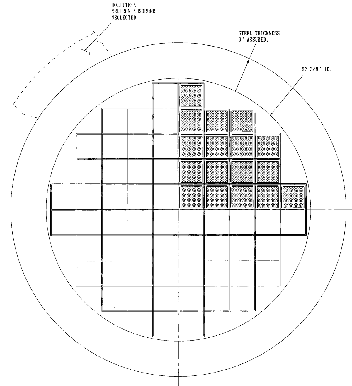
FIGURE 6.3.6; CALCULATION MODEL (PLANAR CROSS-SECTION) WITH FUEL ILLUSTRATED IN ONE QUADRANT OF THE MPC-68
