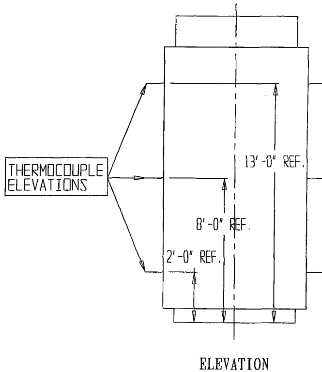
FIGURE 9.1.2; THERMOCOUPLE LOCATIONS
