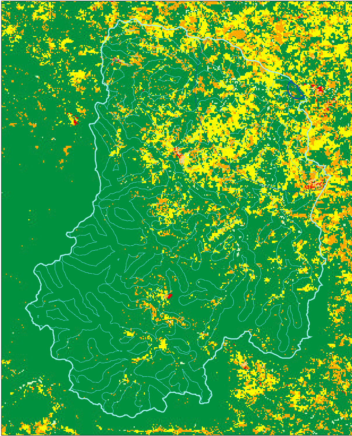
FIGURE 5: LAND USE RATING CLEVELAND COUNTY WATER PWS ID: 0123055, 1ST BROAD RIVER
