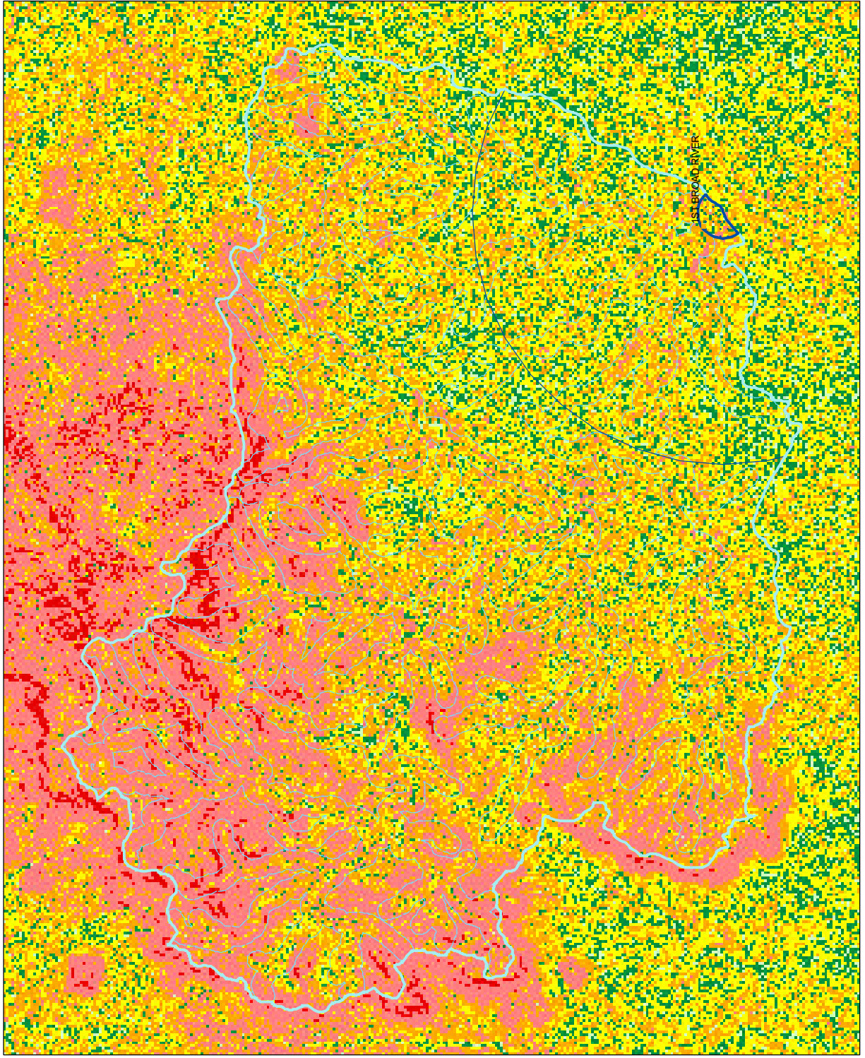
FIGURE 4: LAND SURFACE SLOPE RATING CLEVELAND COUNTY WATER PWS ID: 0123055, 1ST BROAD RIVER
