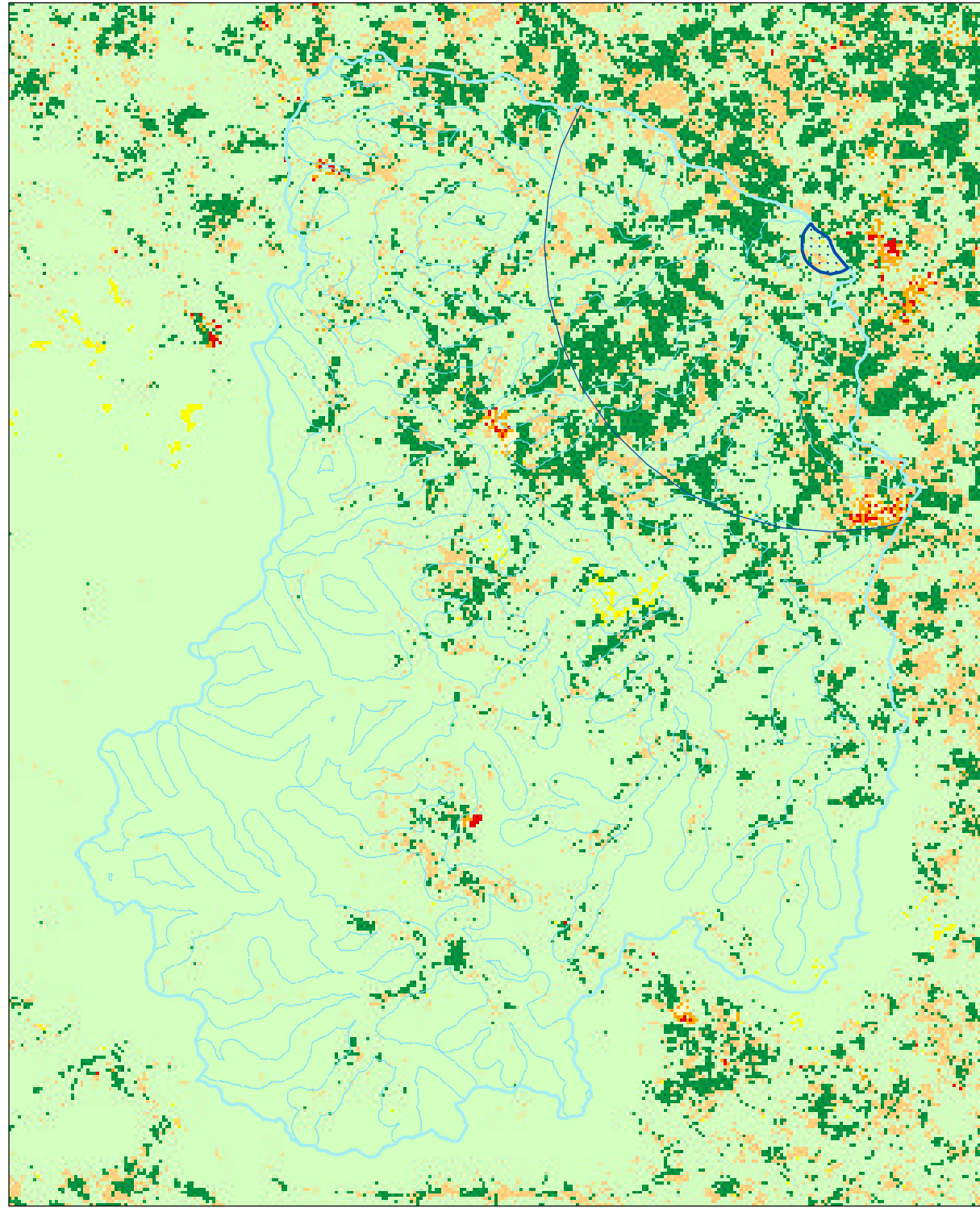
FIGURE 6: LAND COVER RATING CLEVELAND COUNTY WATER PWS ID: 0123055, 1ST BROAD RIVER
