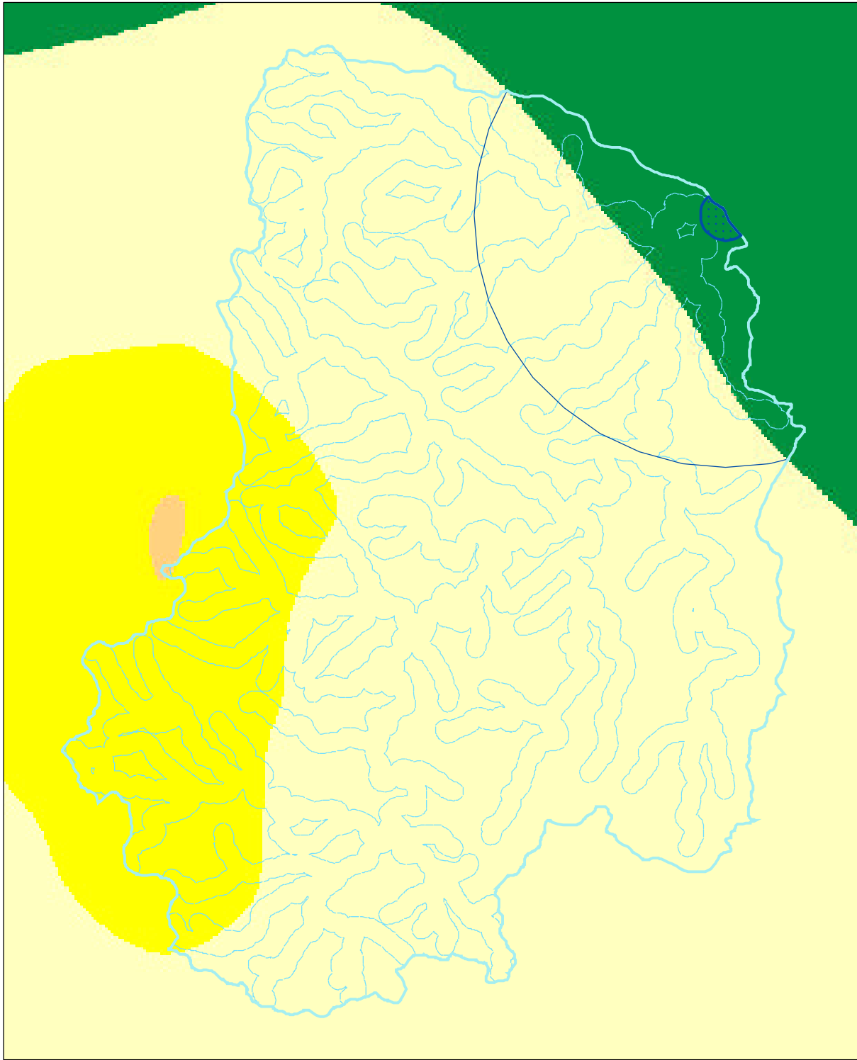
FIGURE 3. AVERAGE ANNUAL PRECIPITATION RATING CLEVELAND COUNTY WATER PWS ID: 0123055, 1ST BROAD RIVER
