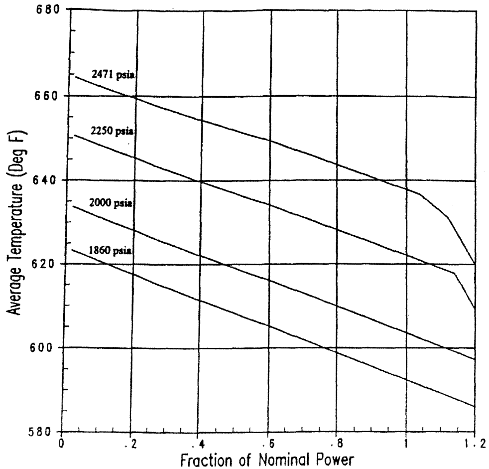
Figure 2.1.1: Reactor Core Limits
