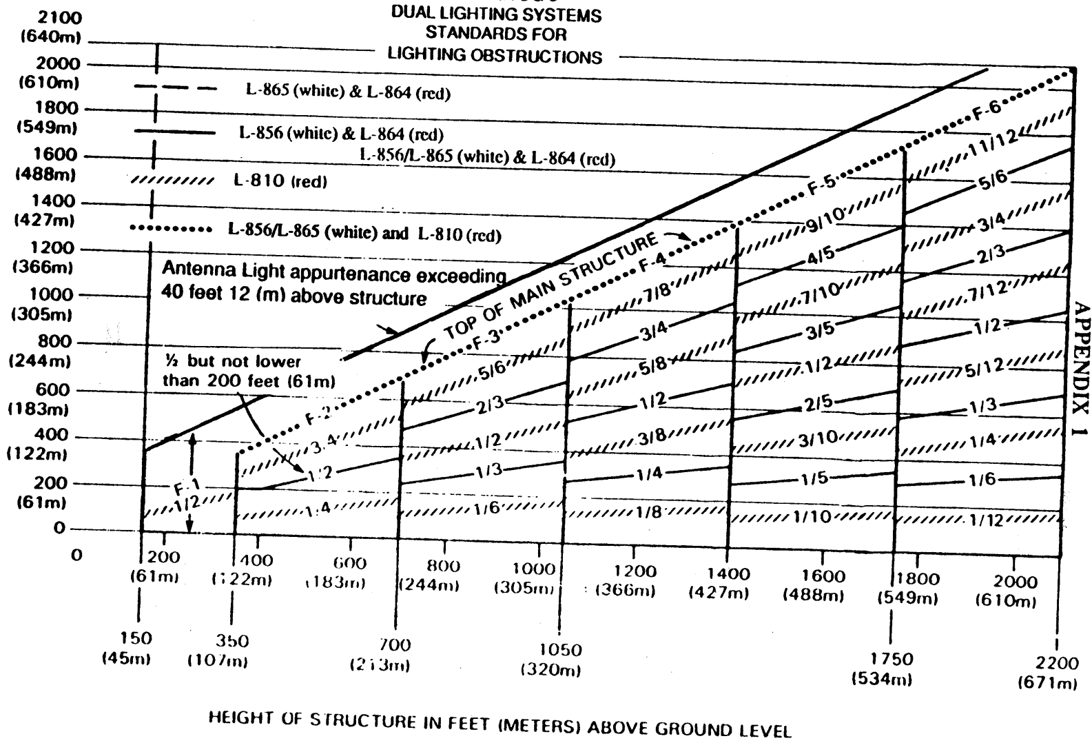
HEIGHT OF LIGHTS ON STRUCTURE IN FEET (METERS) ABOVE GROUND LEVEL
