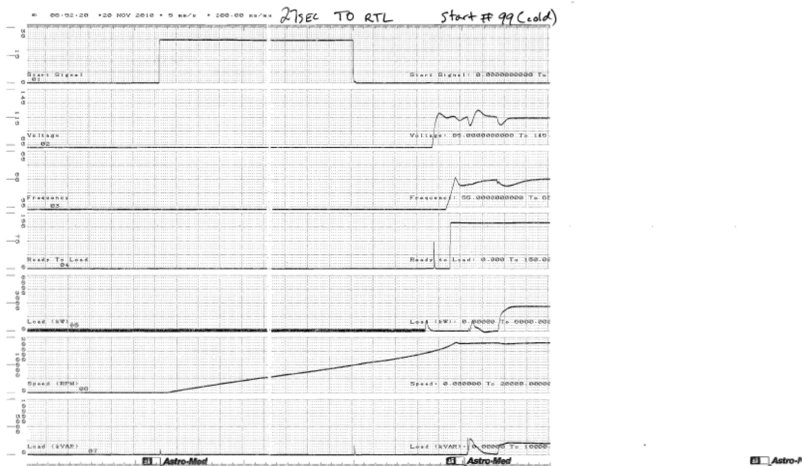
Figure C.1.0-100 Parameter Chart of Start and Load Acceptance Test, No.99, Cold
