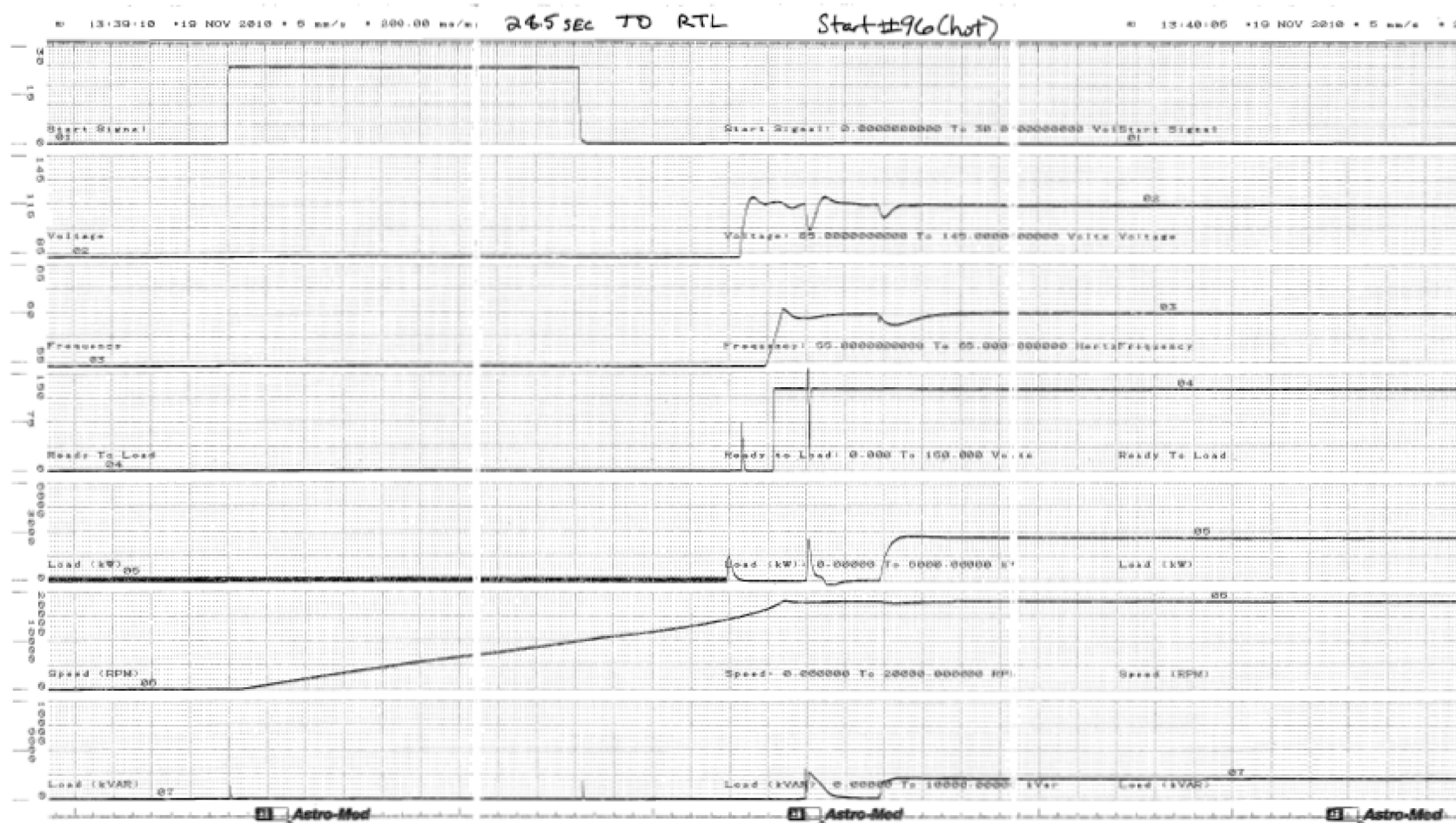
Figure C.1.0-97 Parameter Chart of Start and Load Acceptance Test, No.96, Hot
