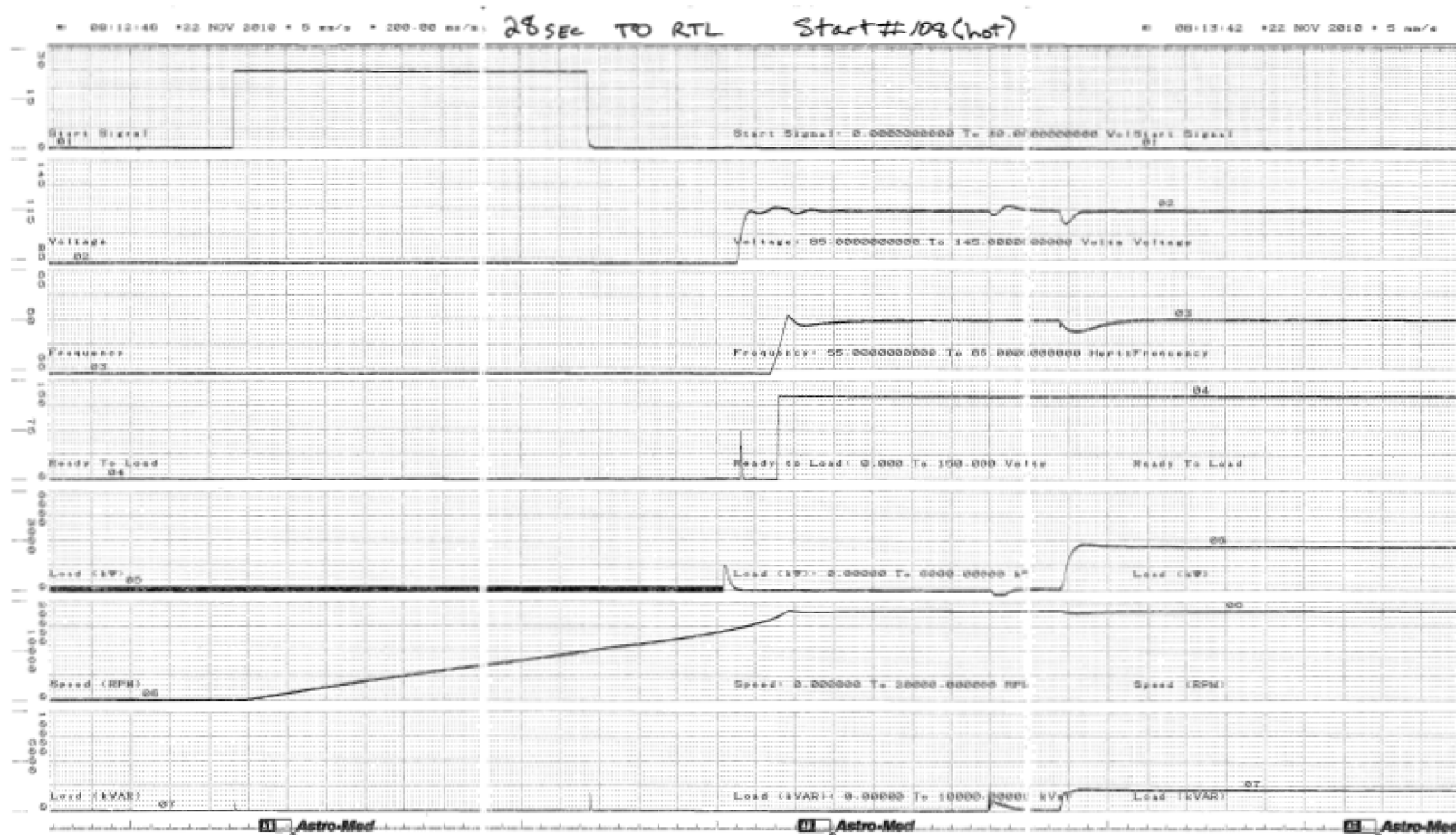
Figure C.1.0-109 Parameter Chart of Start and Load Acceptance Test, No.108, Hot
