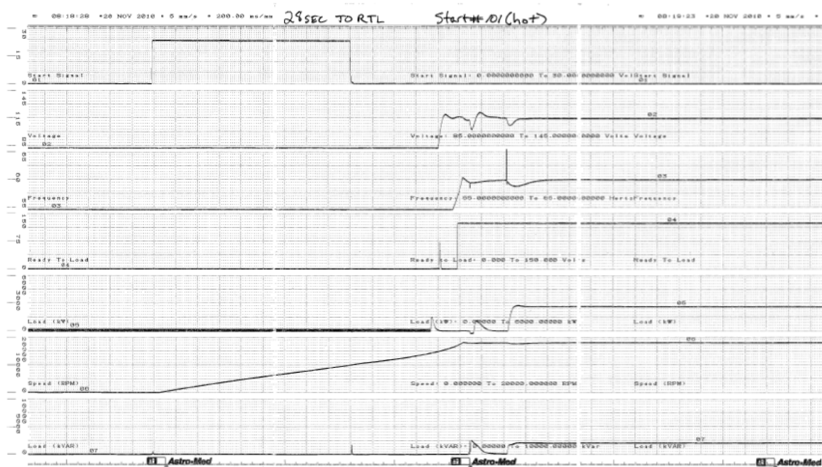
Figure C.1.0-102 Parameter Chart of Start and Load Acceptance Test, No.101, Hot
