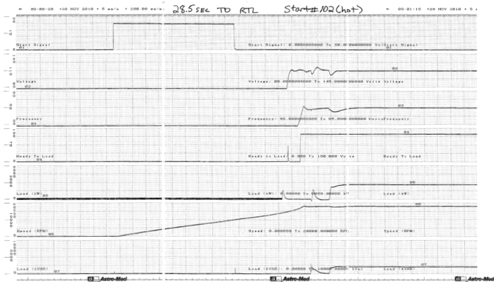
Figure C.1.0-103 Parameter Chart of Start and Load Acceptance Test, No.102, Hot
