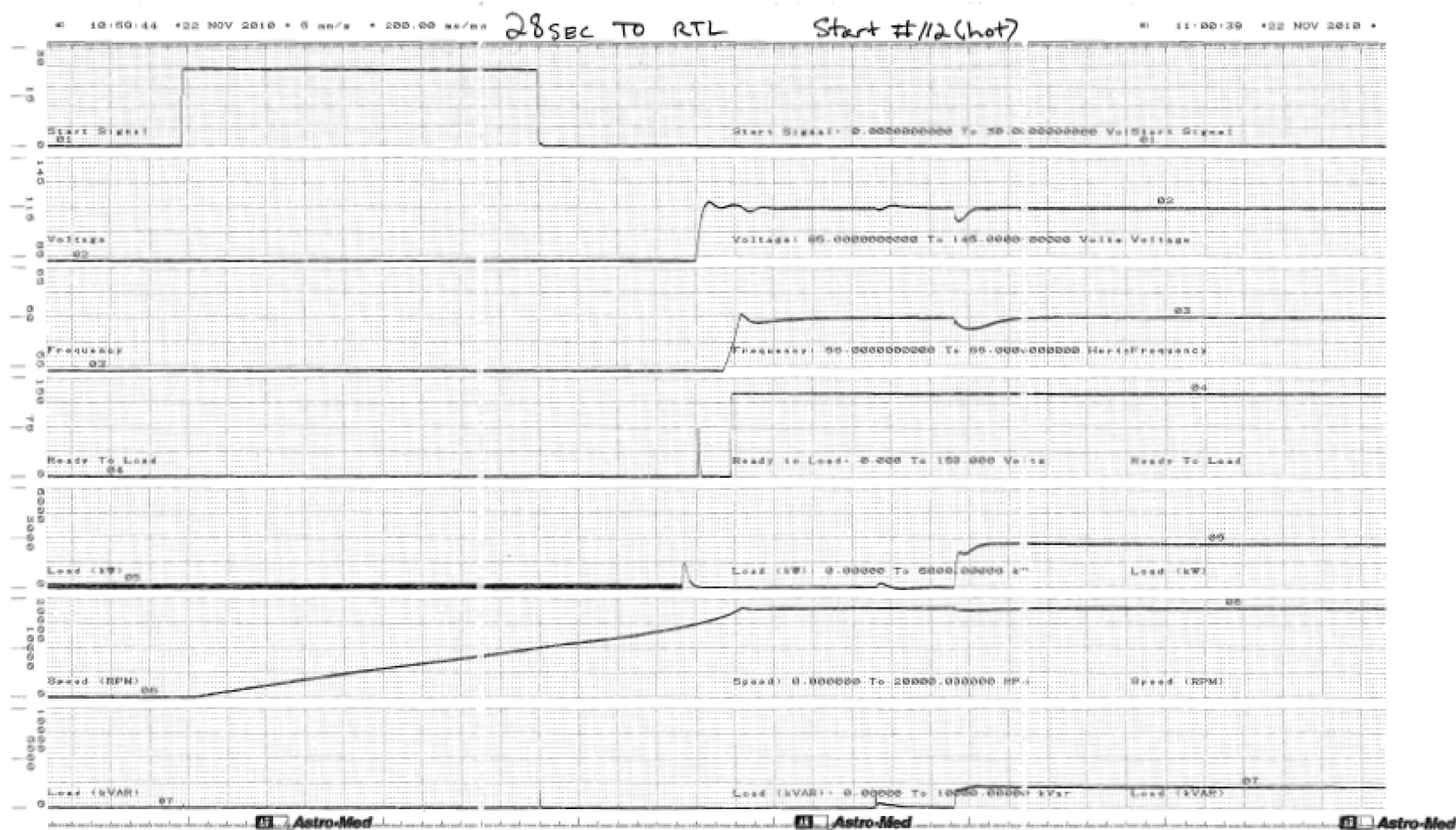
Figure C.1.0-113 Parameter Chart of Start and Load Acceptance Test, No.112, Hot
