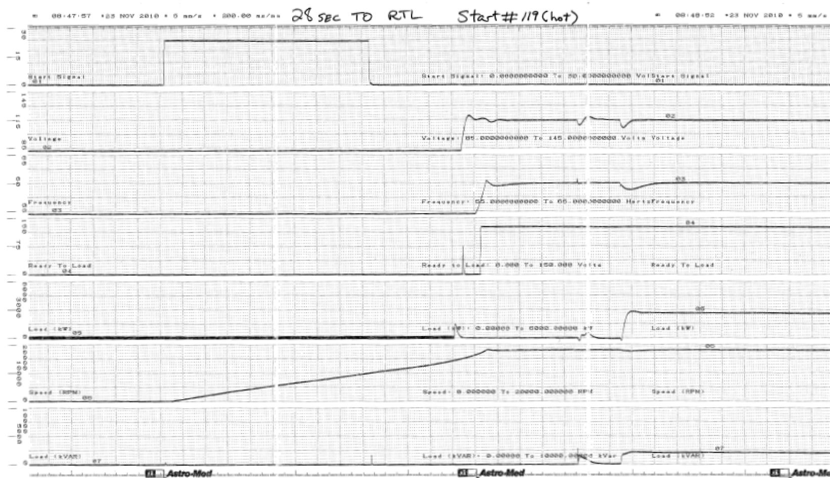
Figure C.1.0-120 Parameter Chart of Start and Load Acceptance Test, No.119, Hot
