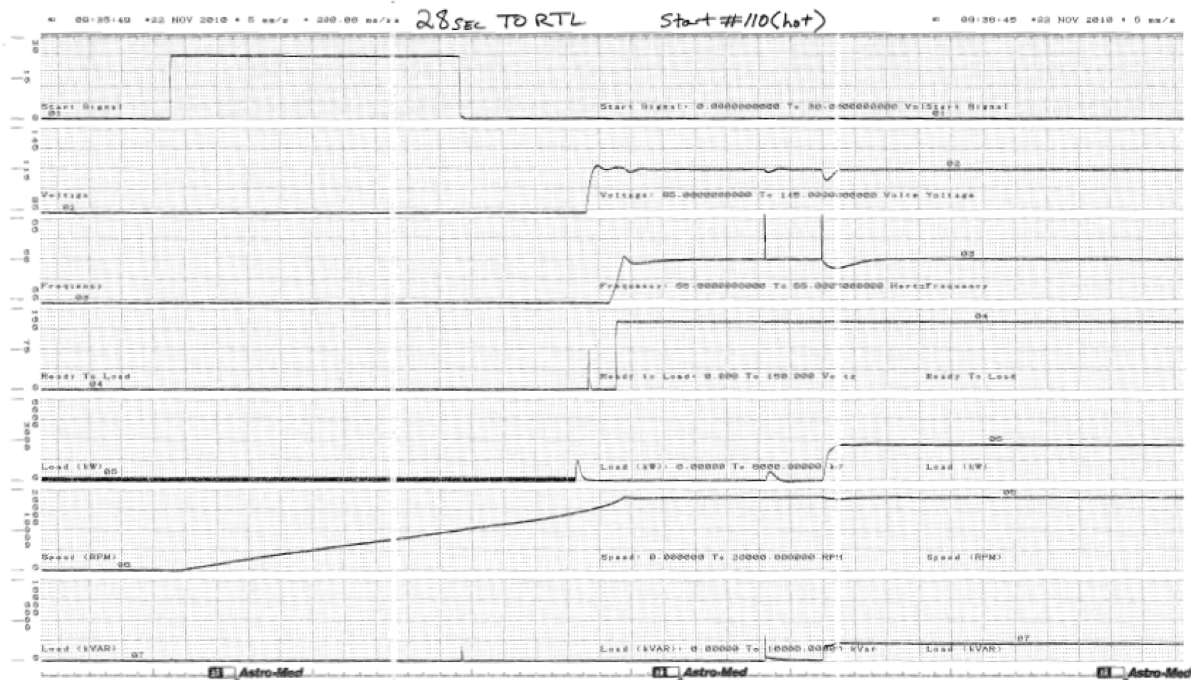
Figure C.1.0-111 Parameter Chart of Start and Load Acceptance Test, No.110, Hot
