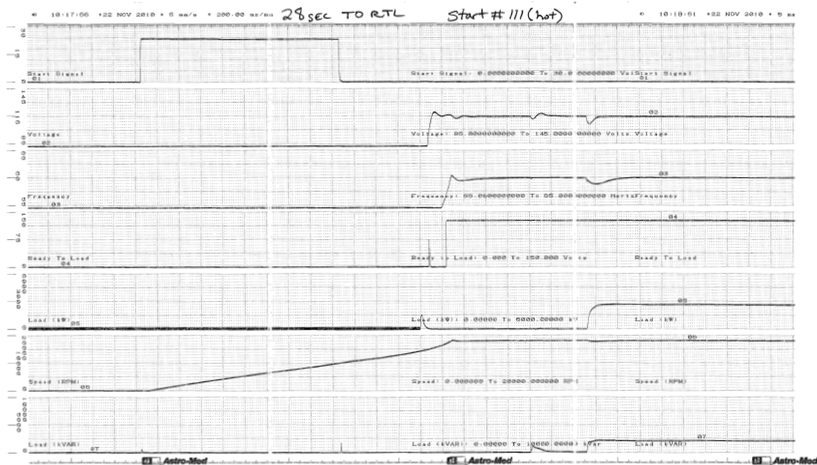
Figure C.1.0-112 Parameter Chart of Start and Load Acceptance Test, No.111, Hot
