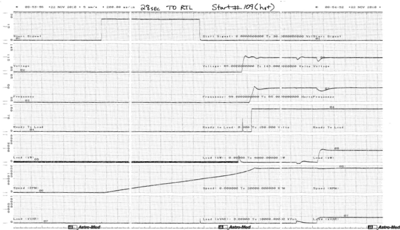
Figure C.1.0-110 Parameter Chart of Start and Load Acceptance Test, No.109, Hot
