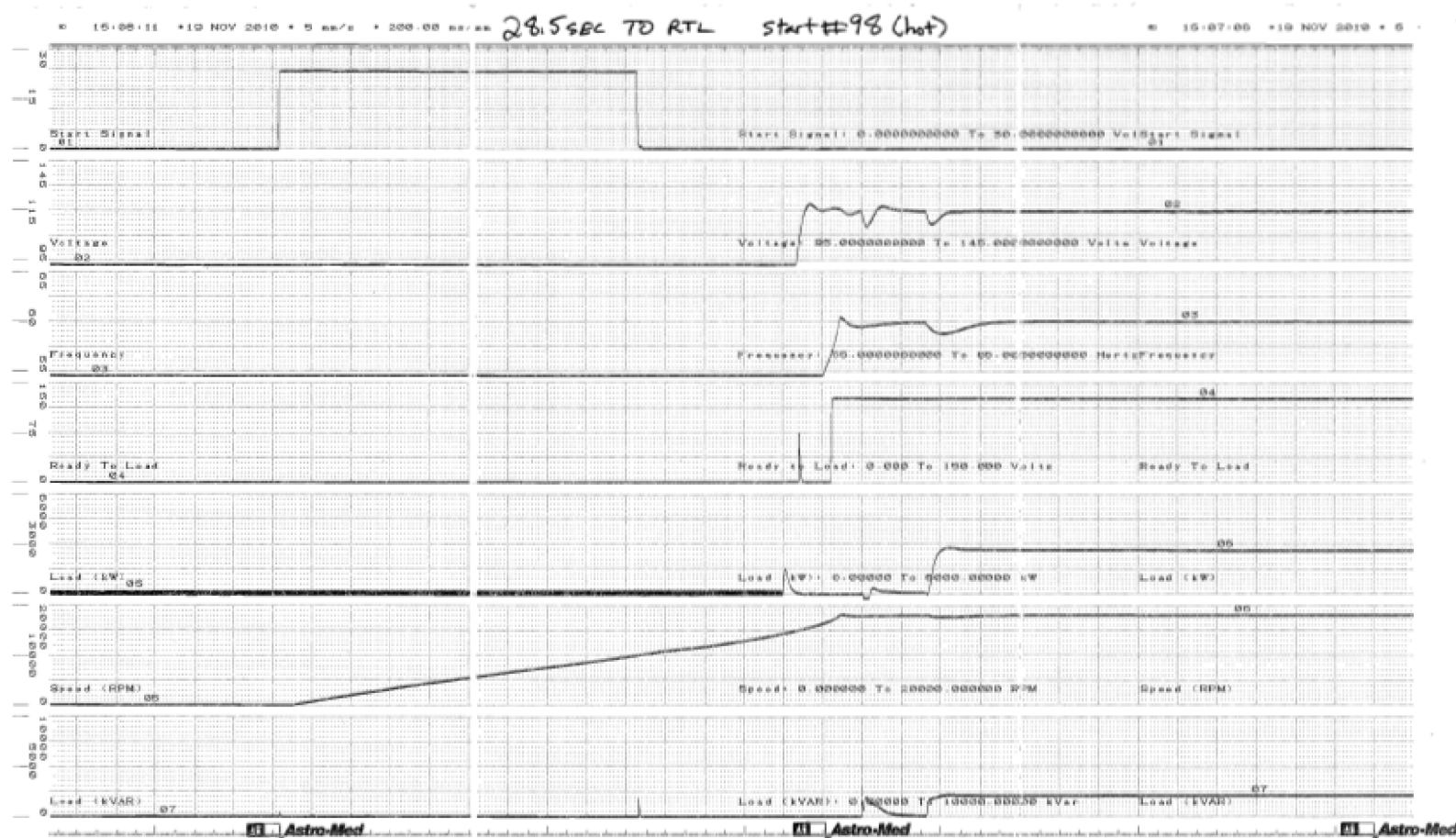
Figure C.1.0-99 Parameter Chart of Start and Load Acceptance Test, No.98, Hot
