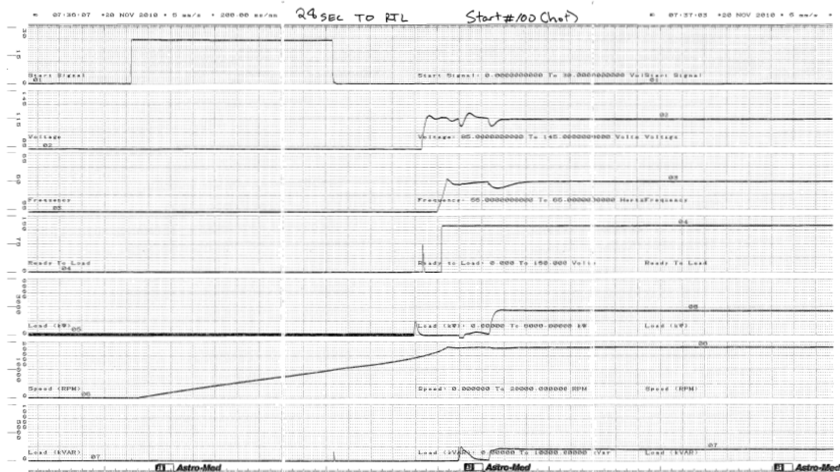
Figure C.1.0-101 Parameter Chart of Start and Load Acceptance Test, No.100, Hot
