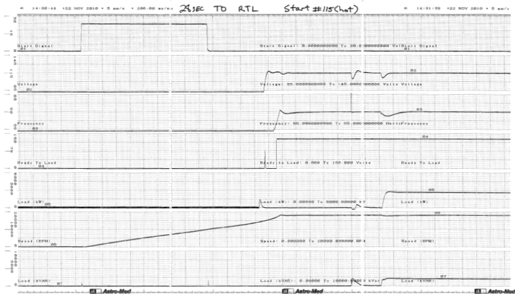
Figure C.1.0-116 Parameter Chart of Start and Load Acceptance Test, No.115, Hot
