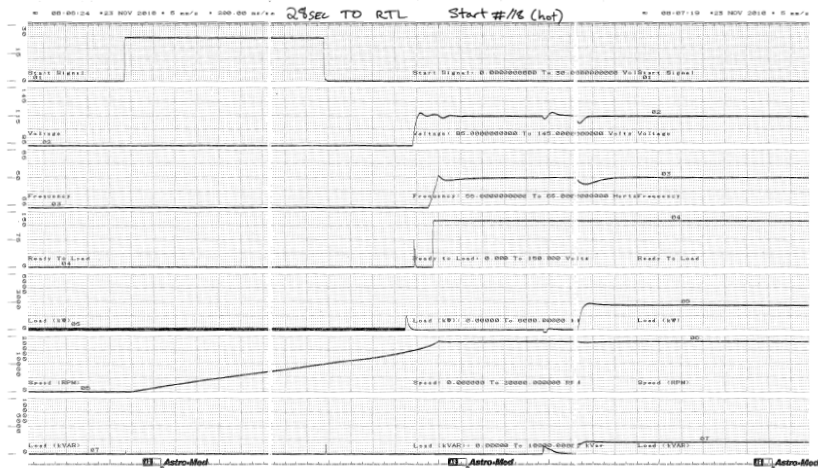
Figure C.1.0-119 Parameter Chart of Start and Load Acceptance Test, No.118, Hot
