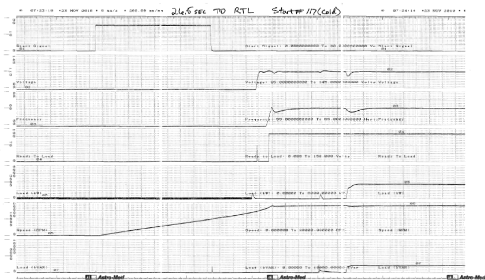
Figure C.1.0-118 Parameter Chart of Start and Load Acceptance Test, No.117, Cold
