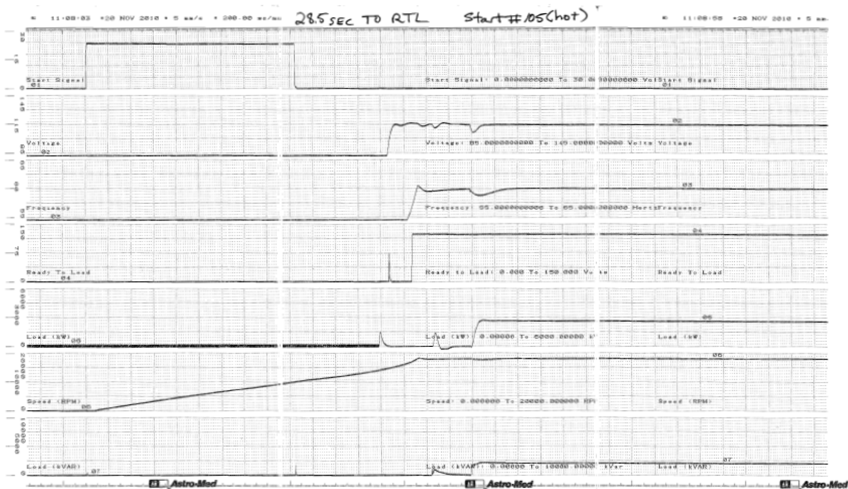
Figure C.1.0-106 Parameter Chart of Start and Load Acceptance Test, No.105, Hot
