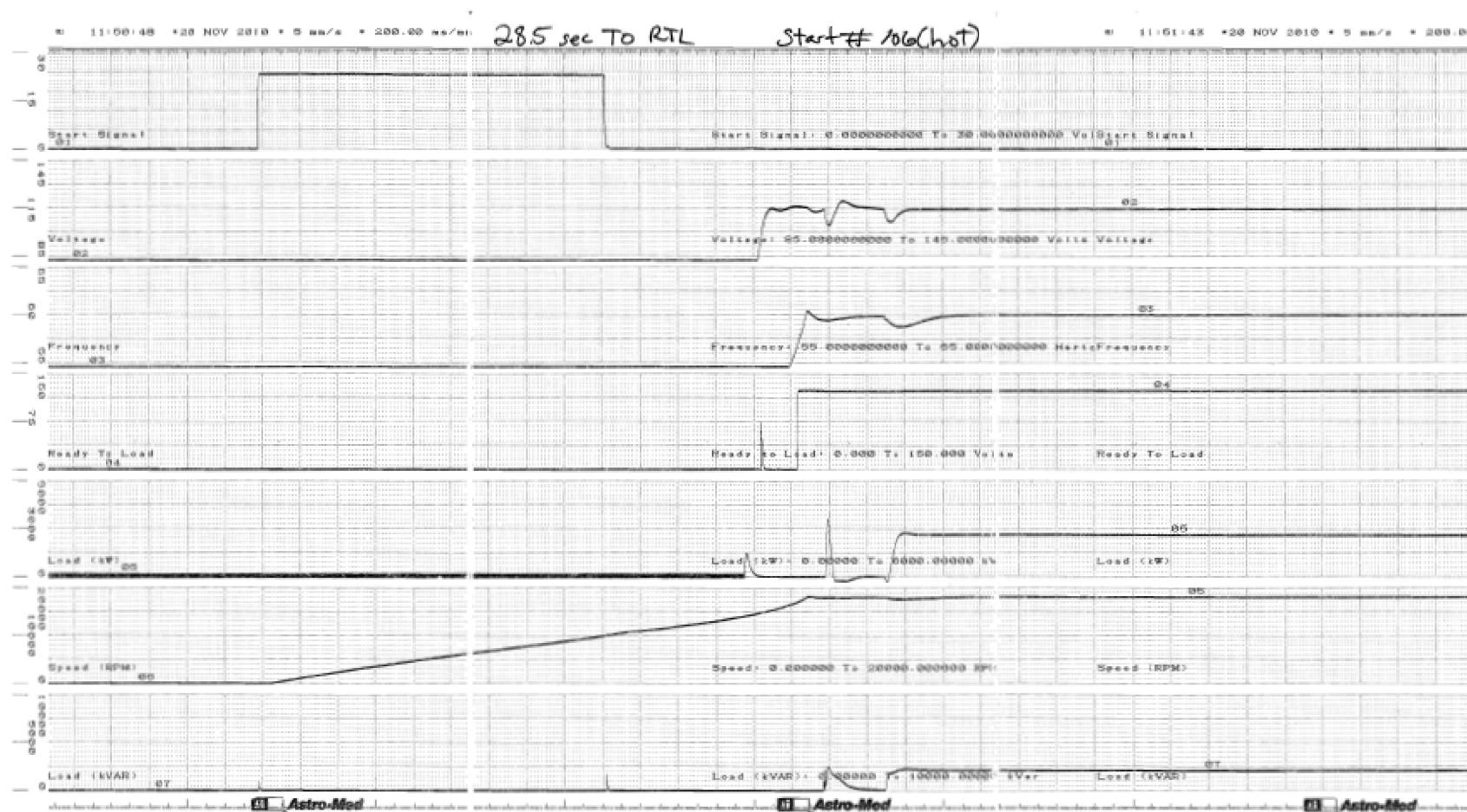
Figure C.1.0-107 Parameter Chart of Start and Load Acceptance Test, No.106, Hot
