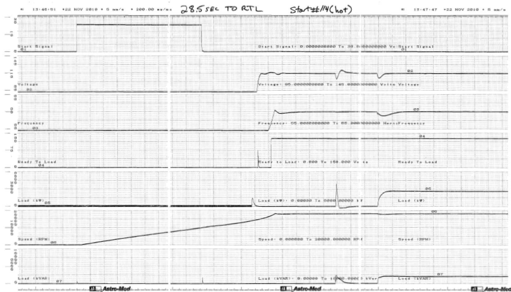
Figure C.1.0-115 Parameter Chart of Start and Load Acceptance Test, No.114, Hot
