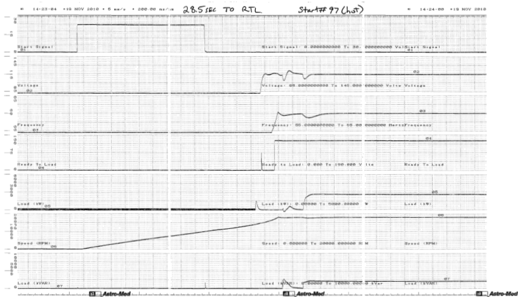
Figure C.1.0-98 Parameter Chart of Start and Load Acceptance Test, No.97, Hot
