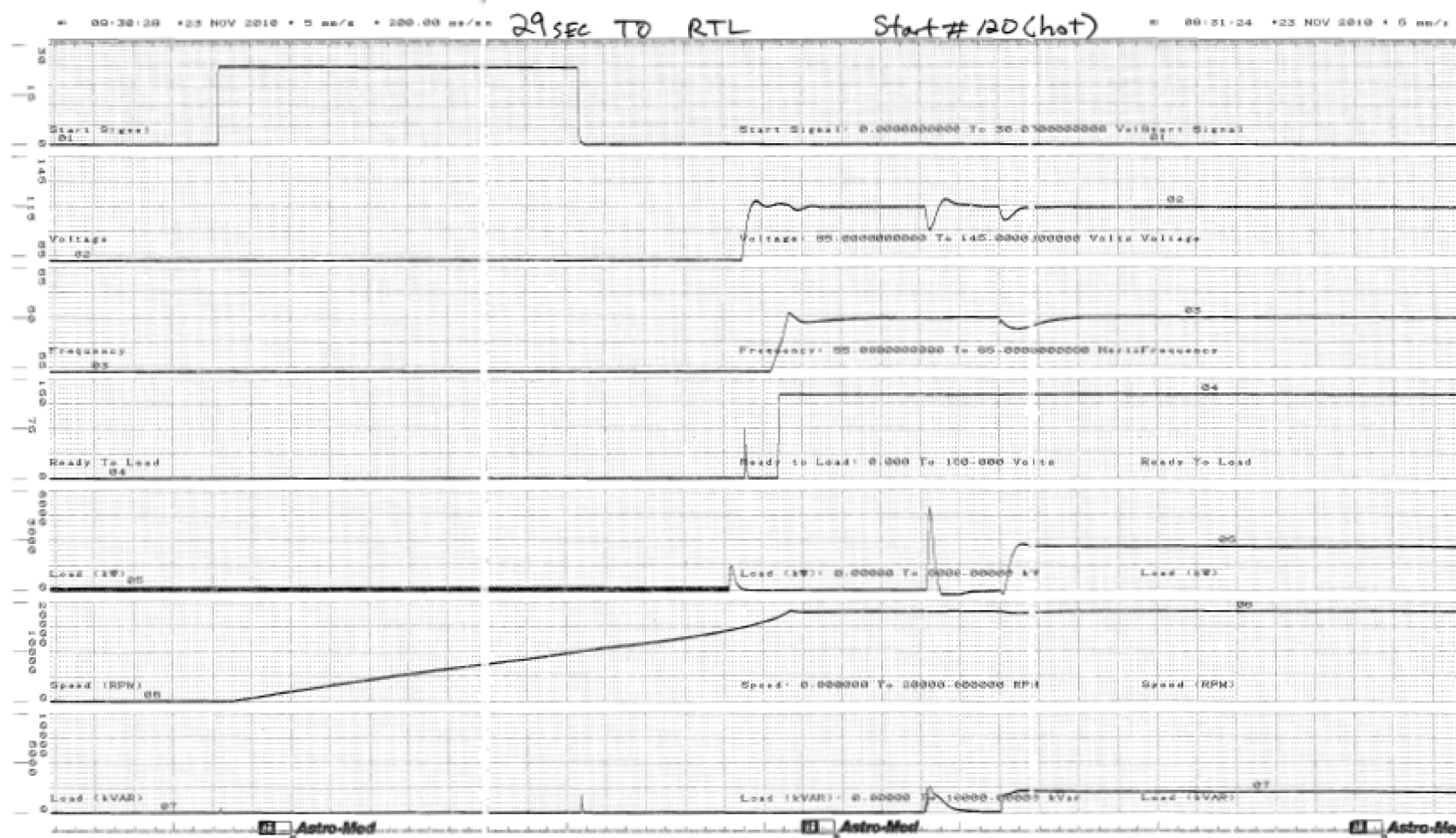
Figure C.1.0-121 Parameter Chart of Start and Load Acceptance Test, No.120, Hot
