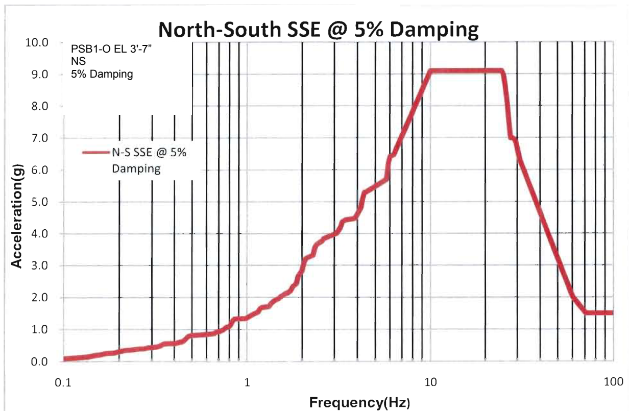
Figure 8.2-7 North-South RRS for Lube Oil Cooler Fan Assembly
