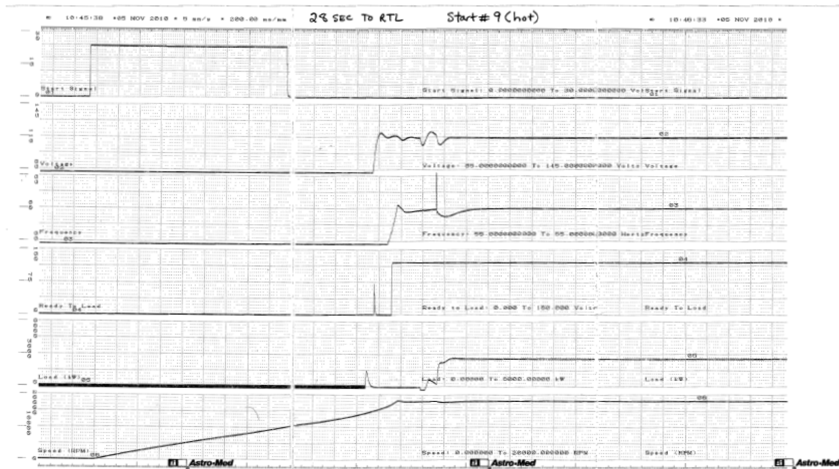
Figure C.1.0-10 Parameter Chart of Start and Load Acceptance Test, No.9, Hot
