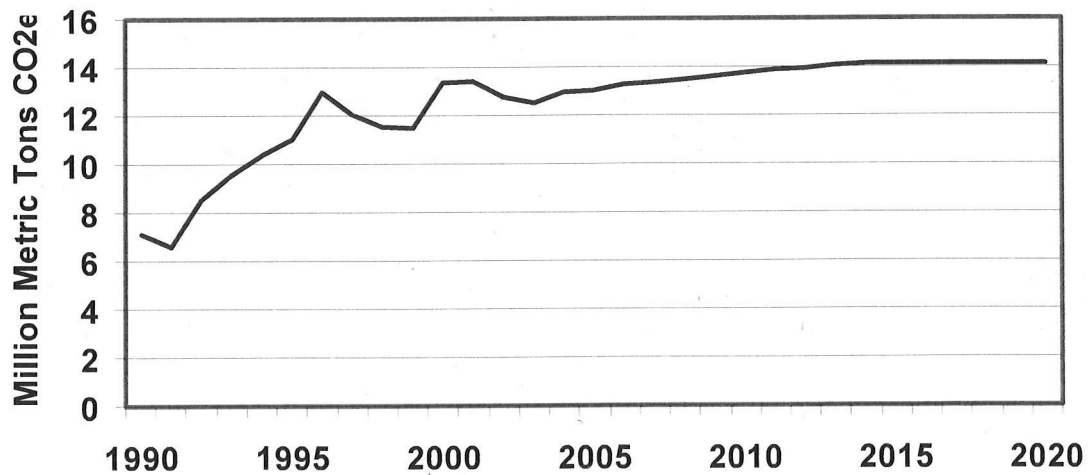
Figure D-6. GHG Emissions from Natural Gas Production and Processing
