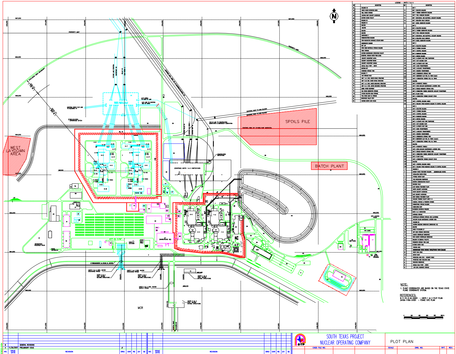
Figure 1.1-1 Site Layout
