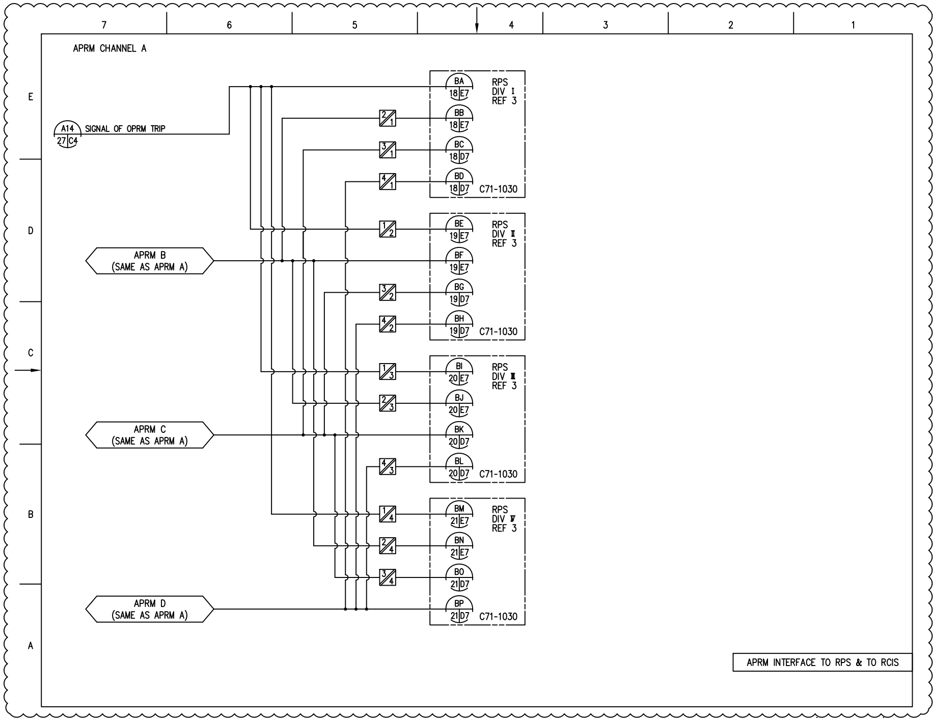
Figure 7.6-2 – Neutron Monitoring System IBD (Sheet 9b of 28)
