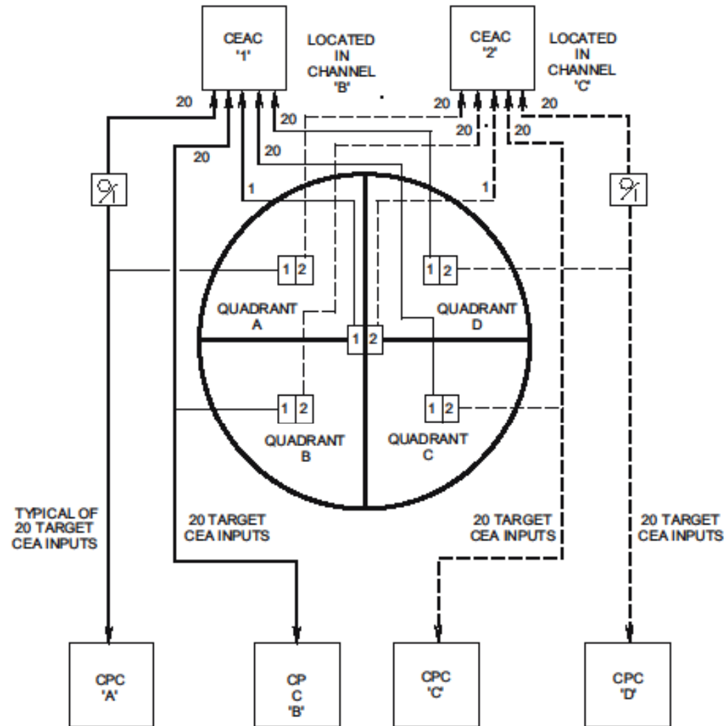
Figure 12.2-1 CEAC Inputs
