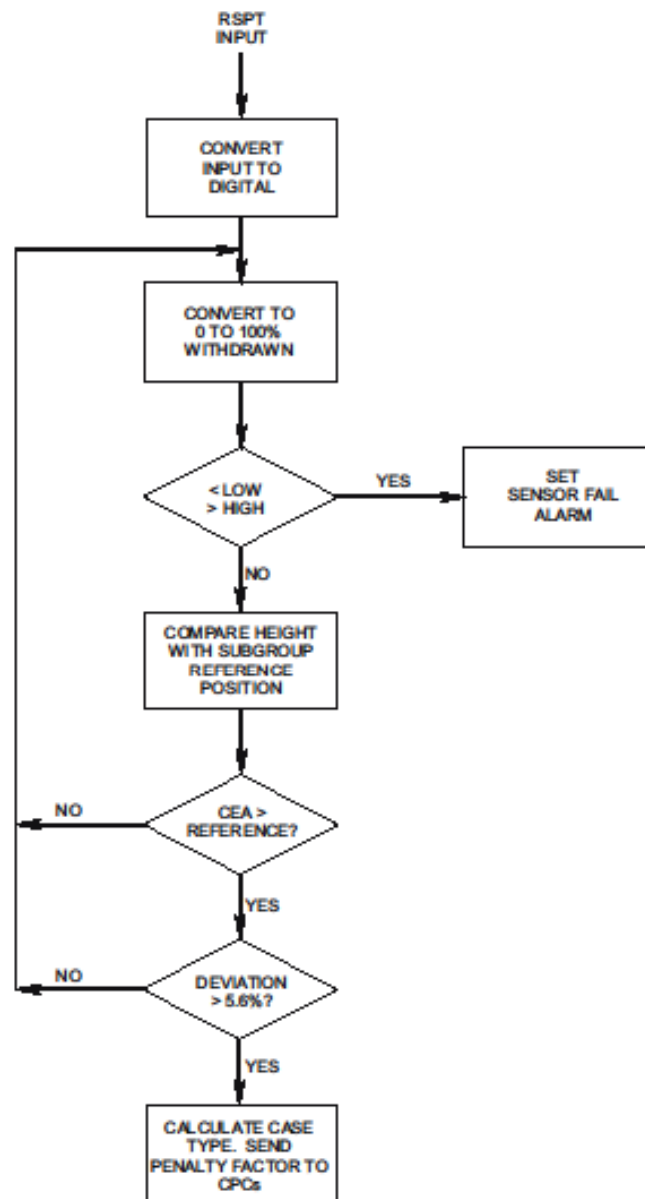
Figure 12.2-2 CEAC Software
