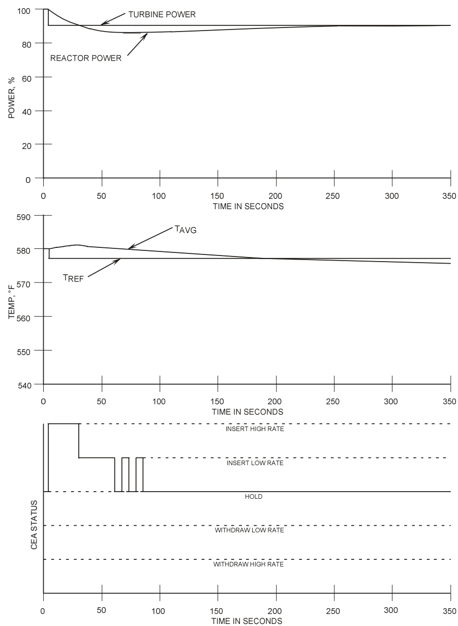
Figure 4-4 Step Load Reduction
