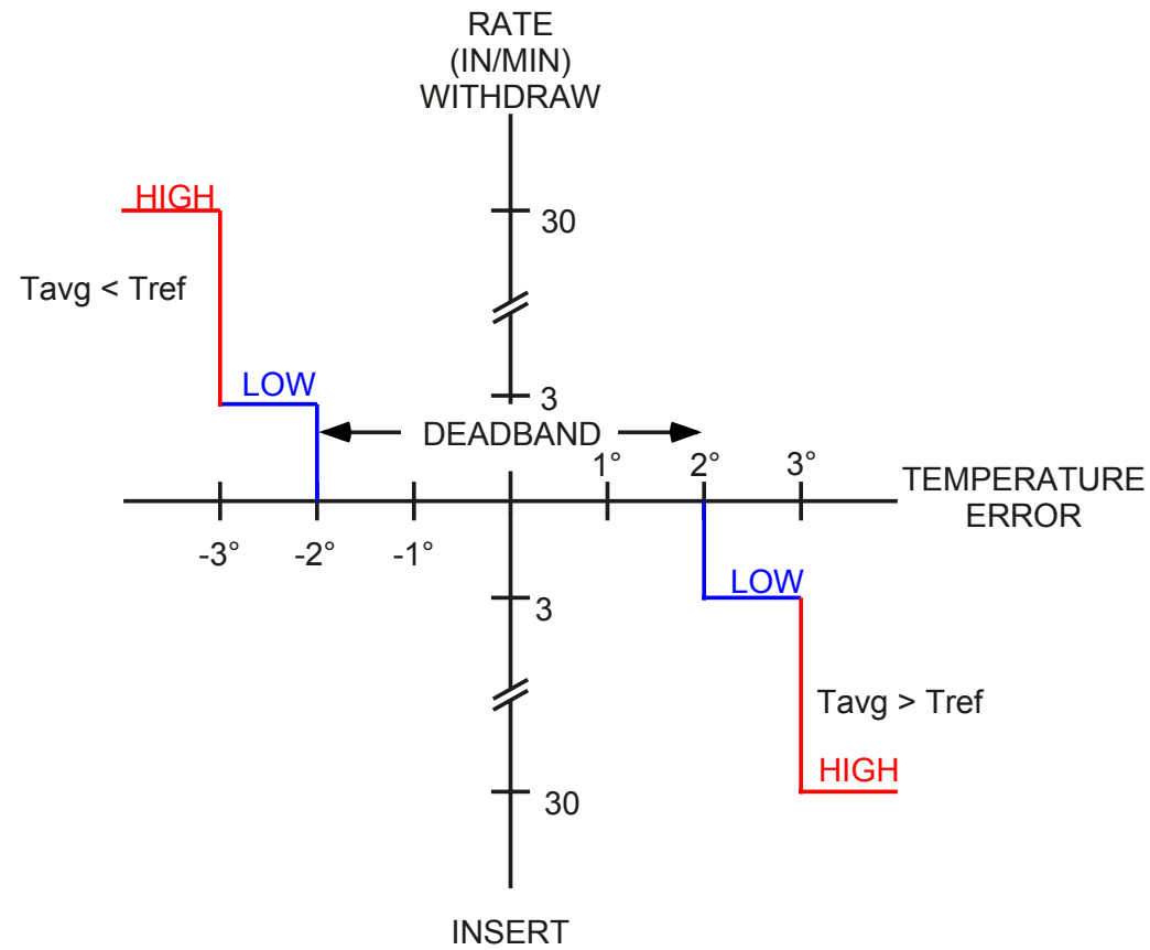
Figure 4-2 CEA Rates and Direction
