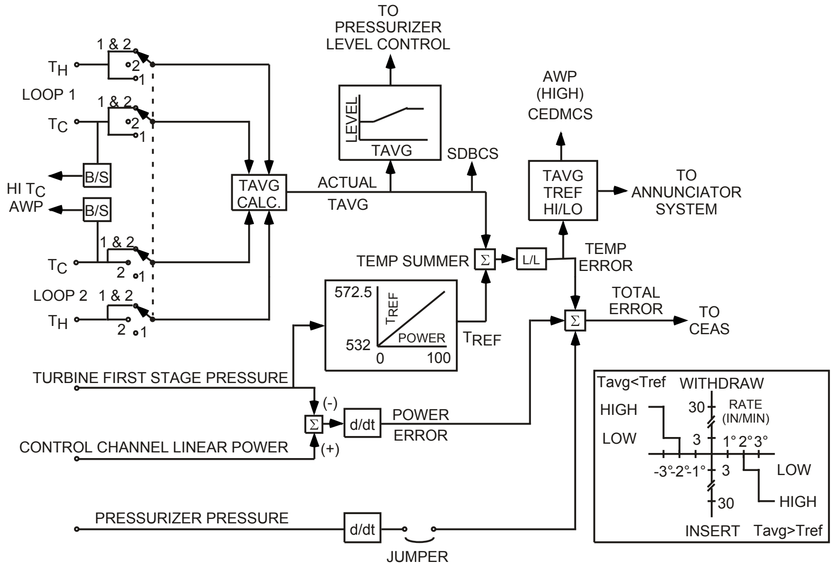
Figure 4-1 Reactor Regulating System
