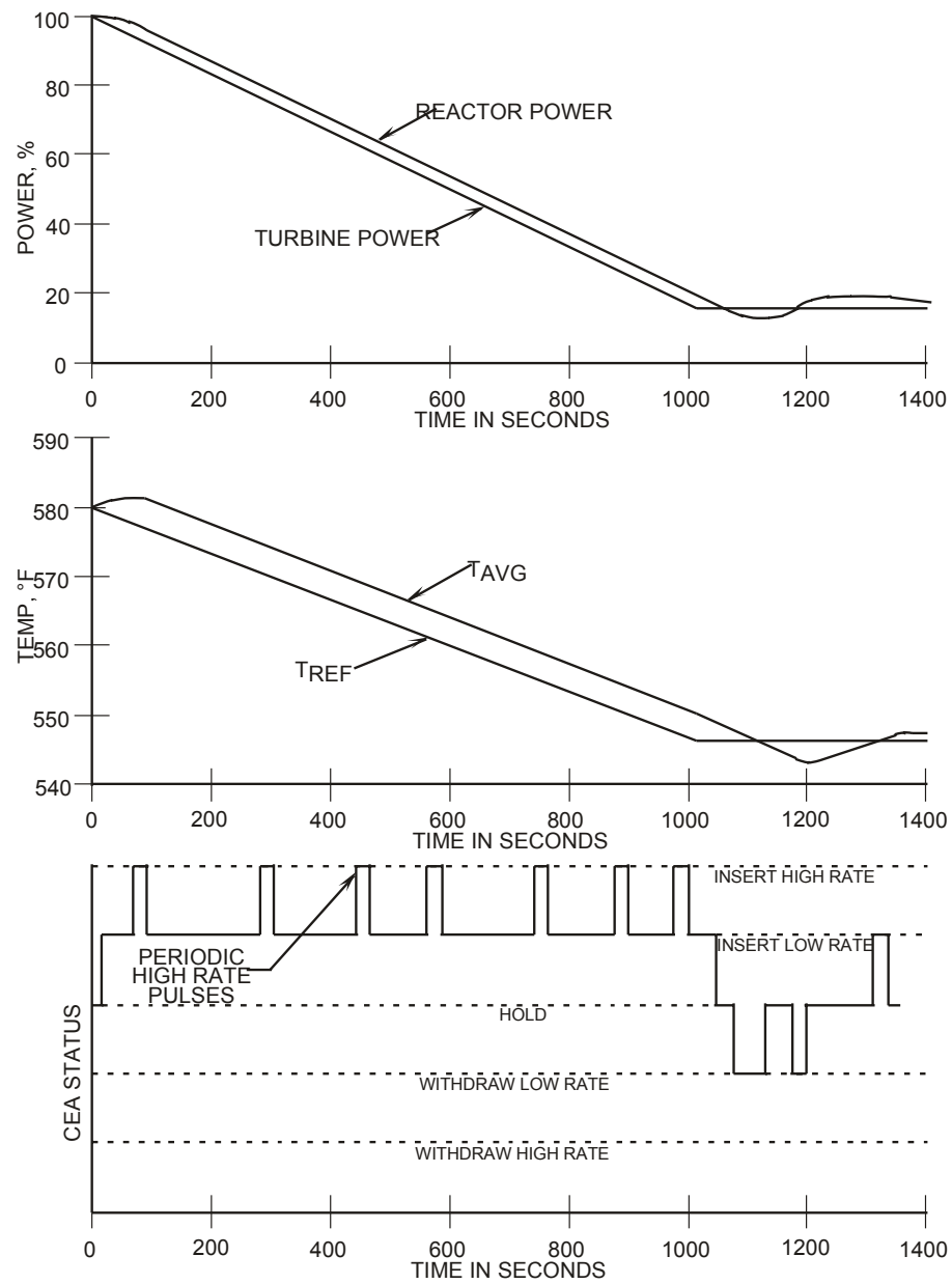
Figure 4-3 Ramp Load Reduction
