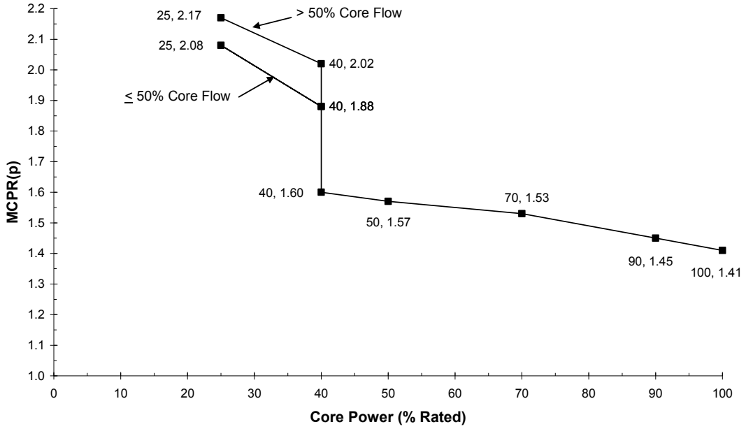
Figure 2-4a Cycle 18 Power-Dependent MCPR Limits for GNF2 MOC to EOC with EOC-RPT Inoperable
