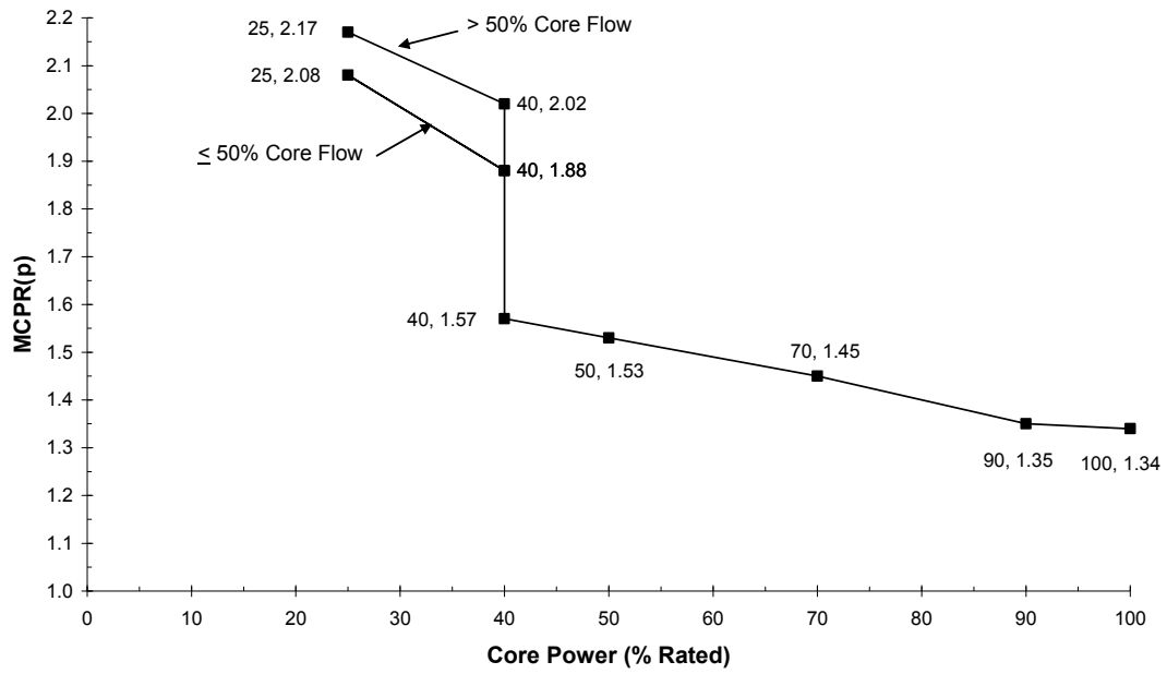
Figure 2-3c Cycle 18 Power-Dependent MCPR Limits for ATRIUM-10 MOC to EOC
