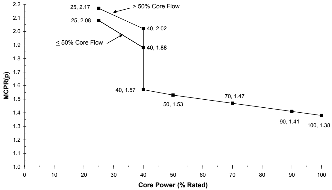
Figure 2-4c Cycle 18 Power-Dependent MCPR Limits for ATRIUM-10 MOC to EOC with EOC-RPT Inoperable
