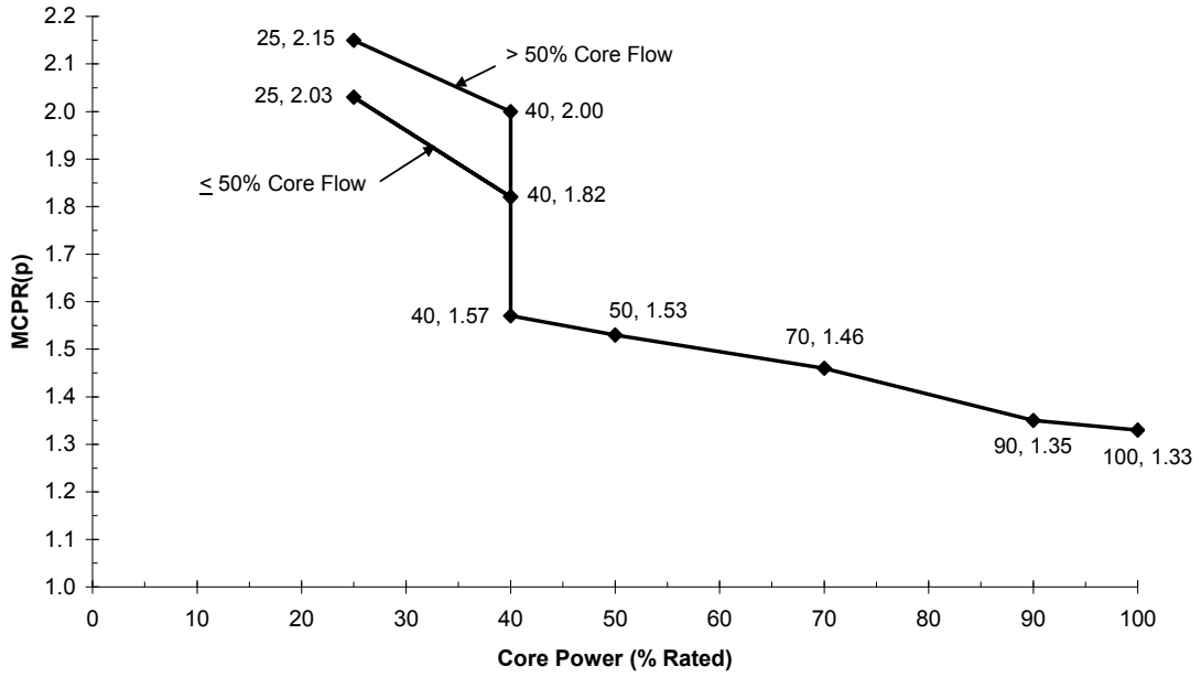
Figure 2-1a Cycle 18 Power-Dependent MCPR Limits for GNF2 BOC to MOC
