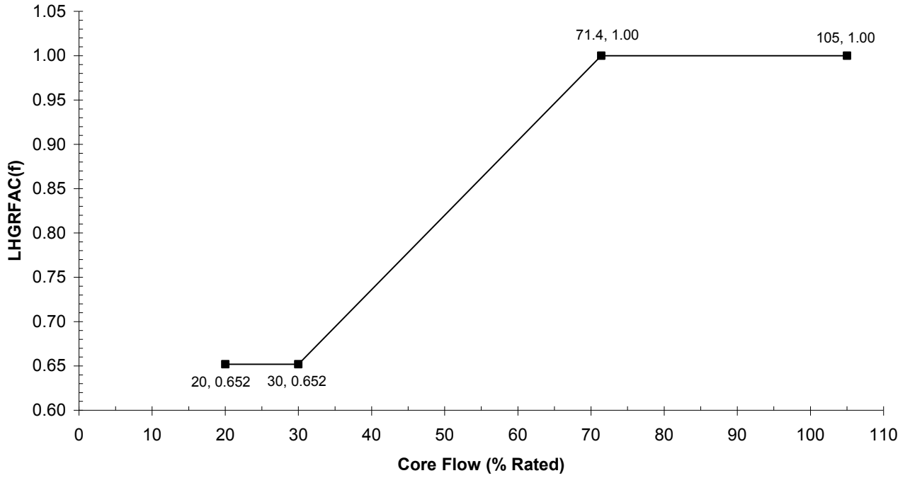
Figure 3-3 Cycle 18 Flow-Dependent LHGR Factor for GNF2, GE14, and ATRIUM-10 Note: These factors to be applied to the exposure-dependent limits as described in Section 5.3
