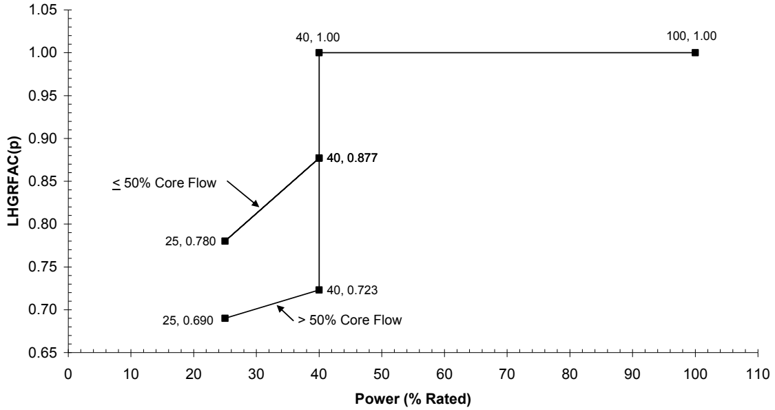
Figure 3-2a Cycle 18 Power-Dependent LHGR Factor BOC-MOC for GNF2, GE14, and ATRIUM-10 Note: These factors to be applied to the exposure-dependent limits as described in Section 5.3
