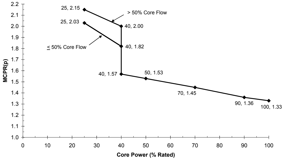
Figure 2-2c Cycle 18 Power-Dependent MCPR Limits for ATRIUM-10 BOC to MOC with EOC-RPT Inoperable
