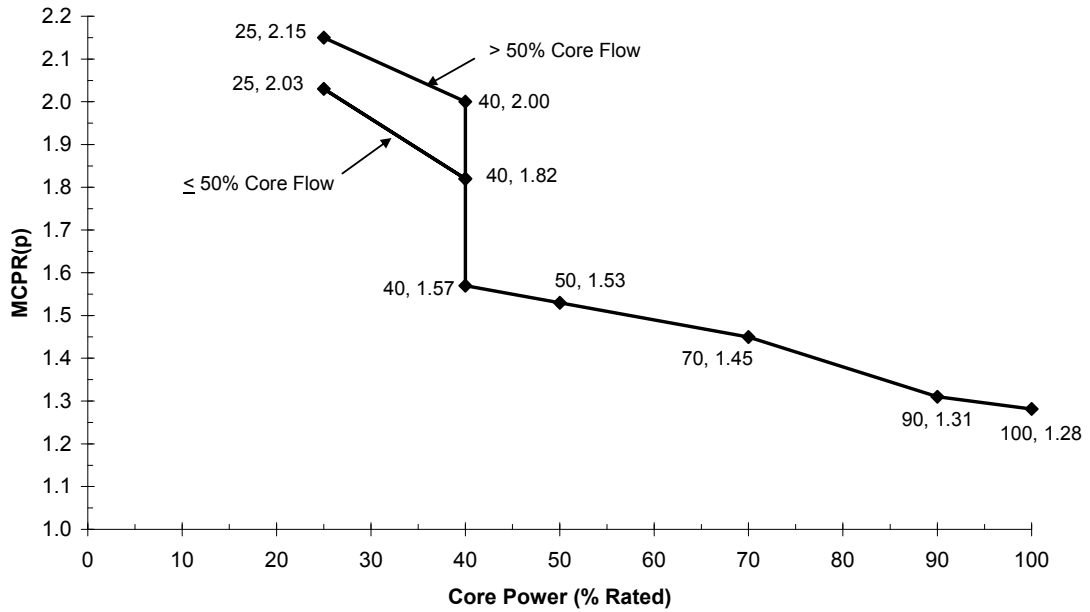
Figure 2-1b Cycle 18 Power-Dependent MCPR Limits for GE14 BOC to MOC
