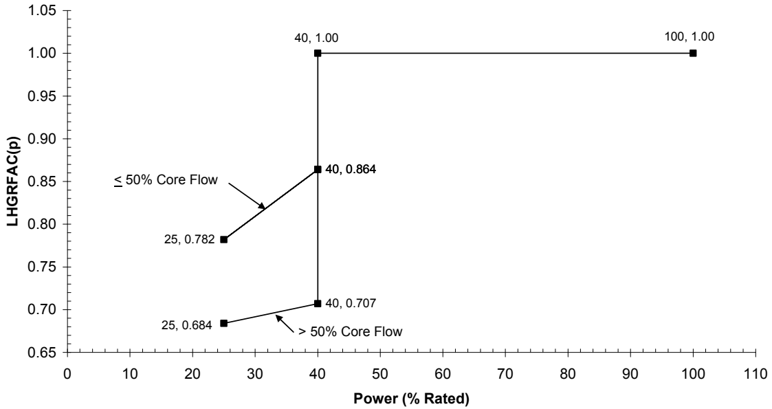
Figure 3-2b Cycle 18 Power-Dependent LHGR Factor MOC-EOC for GNF2, GE14, and ATRIUM-10 Note: These factors to be applied to the exposure-dependent limits as described in Section 5.3
