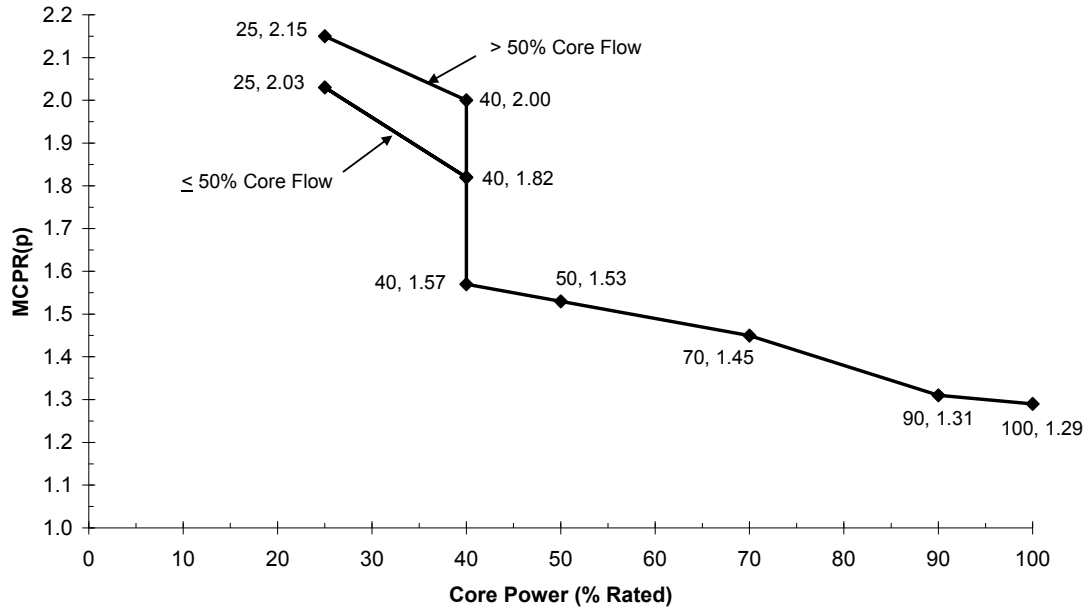
Figure 2-1c Cycle 18 Power-Dependent MCPR Limits for ATRIUM-10 BOC to MOC
