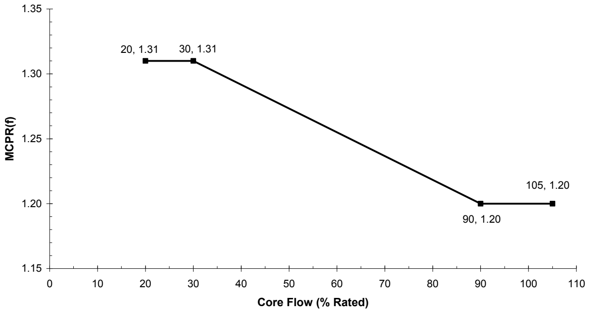
Figure 2-5 Cycle 18 Flow-Dependent MCPR Limits for GNF2, GE14 and ATRIUM-10
