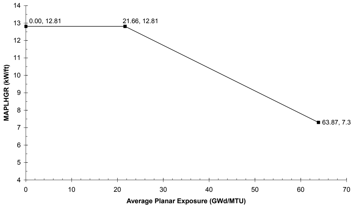
Figure 1-3 Maximum Average Planar Linear Heat generation Rate for ATRIUM-10 Note: Actual Limits described in Sections 5.1 and 5.5
