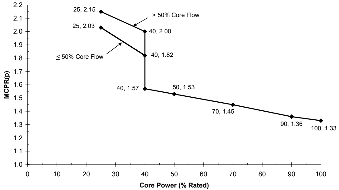
Figure 2-2b Cycle 18 Power-Dependent MCPR Limits for GE14 BOC to MOC with EOC-RPT Inoperable
