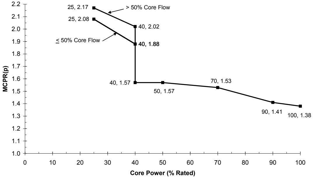
Figure 2-3a Cycle 18 Power-Dependent MCPR Limits for GNF2 MOC to EOC
