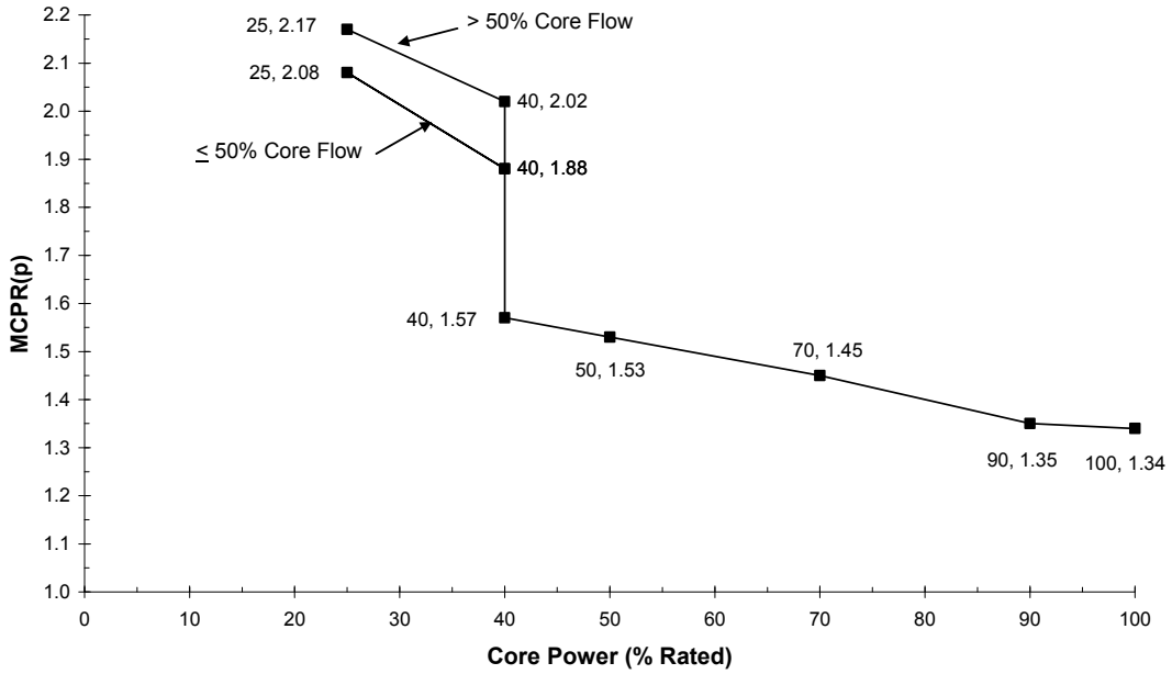
Figure 2-3b Cycle 18 Power-Dependent MCPR Limits for GE14 MOC to EOC
