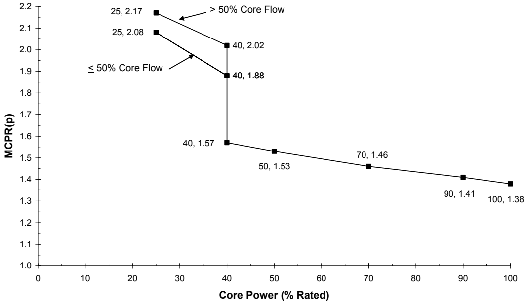
Figure 2-4b Cycle 18 Power-Dependent MCPR Limits for GE14 MOC to EOC with EOC-RPT Inoperable
