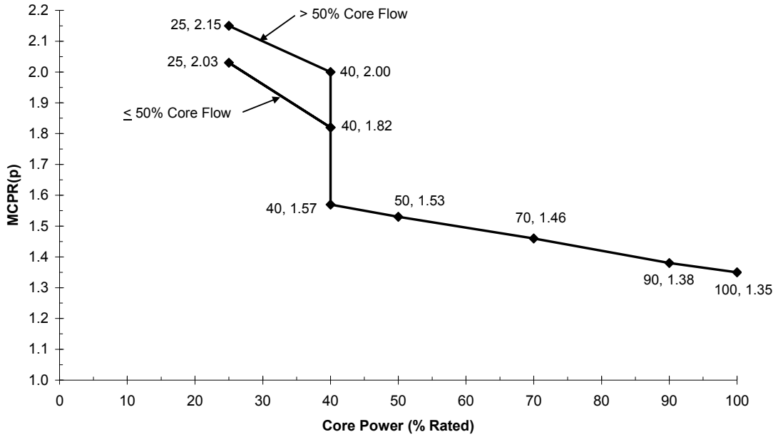
Figure 2-2a Cycle 18 Power-Dependent MCPR Limits for GNF2 BOC to MOC with EOC-RPT Inoperable
