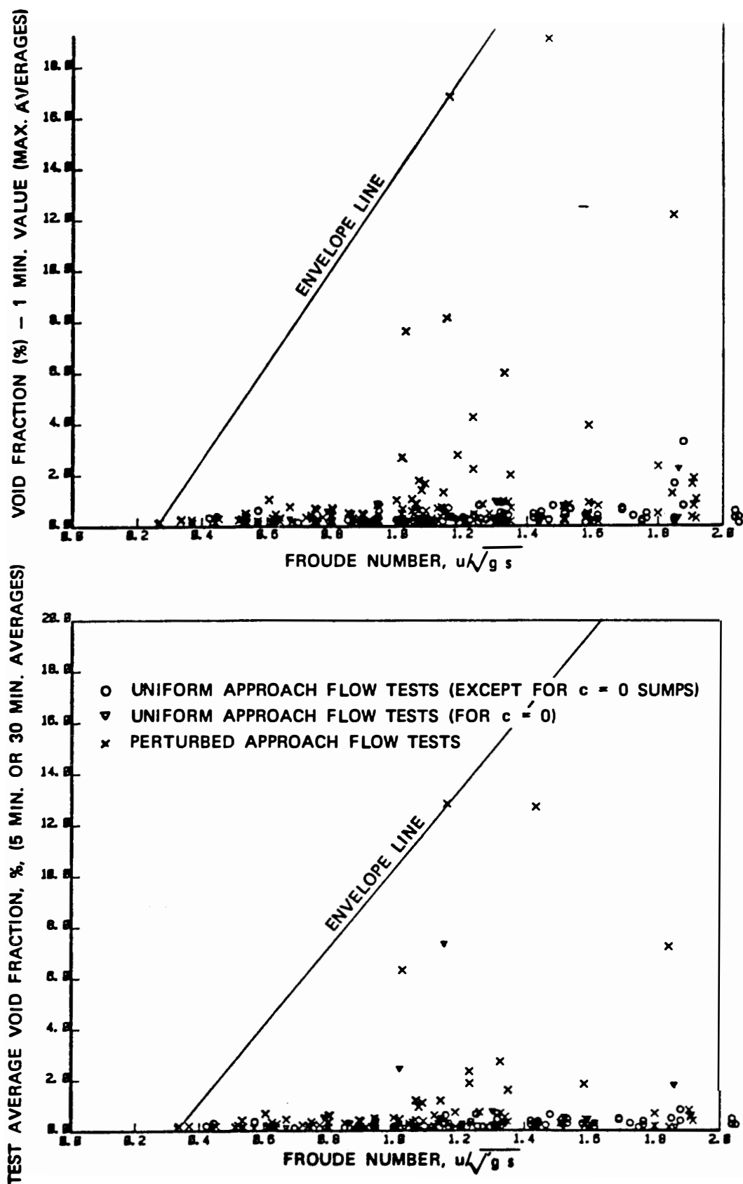
Figure 3.37 Void fraction data for various Froude numbers; vertical intake configuration; only data for nonzero void fraction plotted
