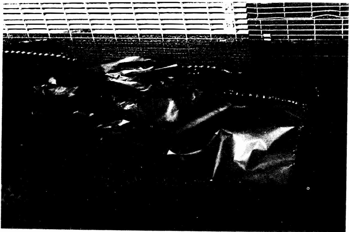
Figure 3.31 Several foil sheets on screen (flow velocity = 0.7 ft/sec)
