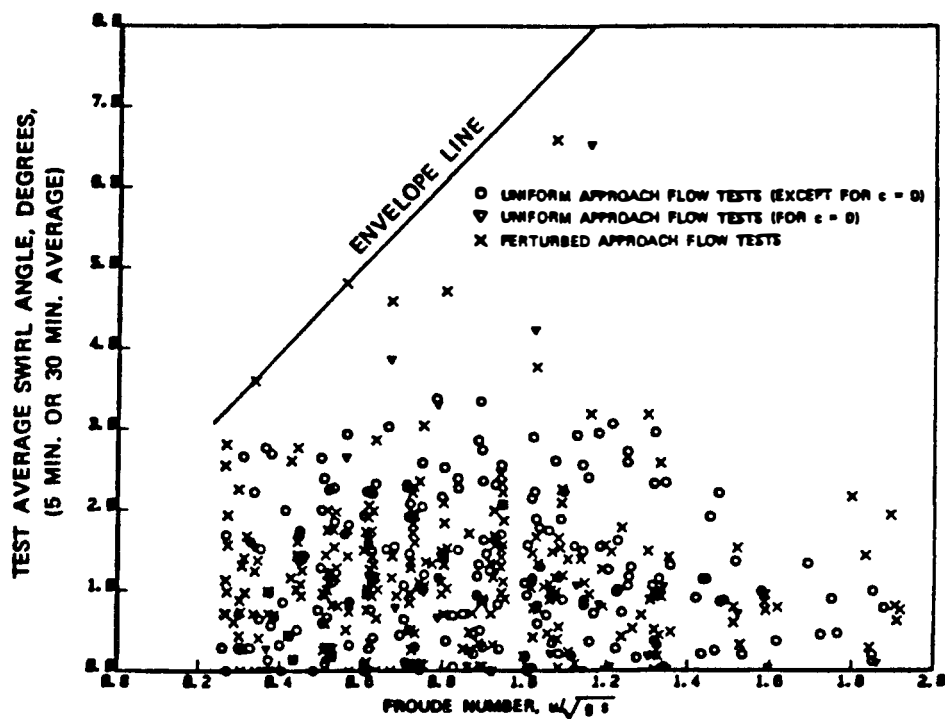
Figure 3.39 Swirl as a function of Froude number, vertical intake configuration
