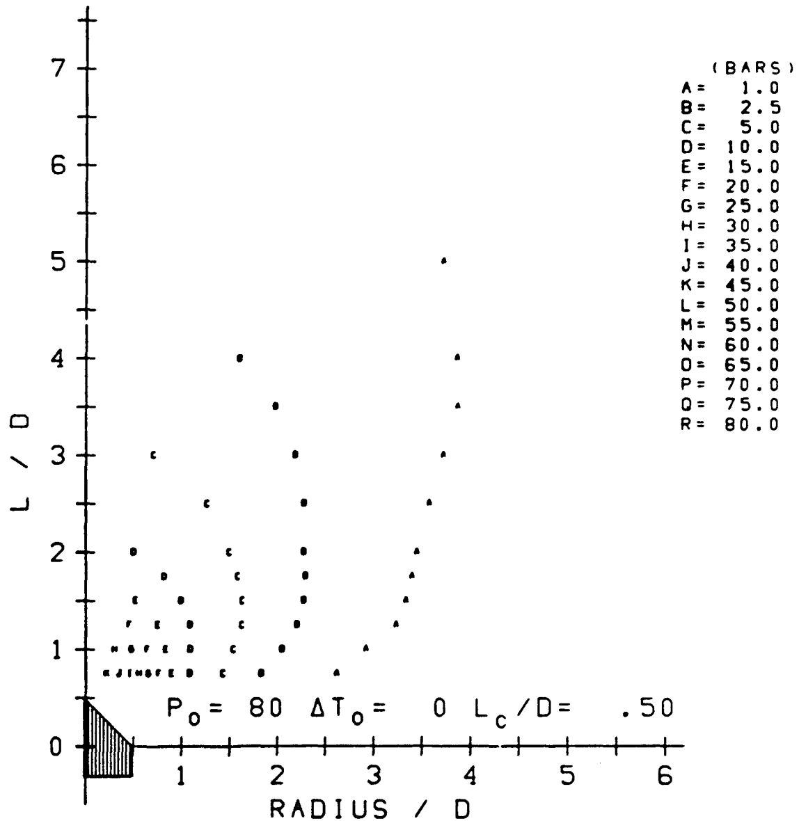
Figure 3.23 Composite target pressure contours as a function of target length/jet diameter ( L/D ) and target radius/jet diameter ( RADIUS/D ) for stagnation conditions of P_o = 80 bars and saturated liquid. Smooth lines connecting like alphabetic letters form an approximate pressure contour corresponding, in bars, to the pressure versus alphabetic letter key. This contour is approximate and is only informational.
