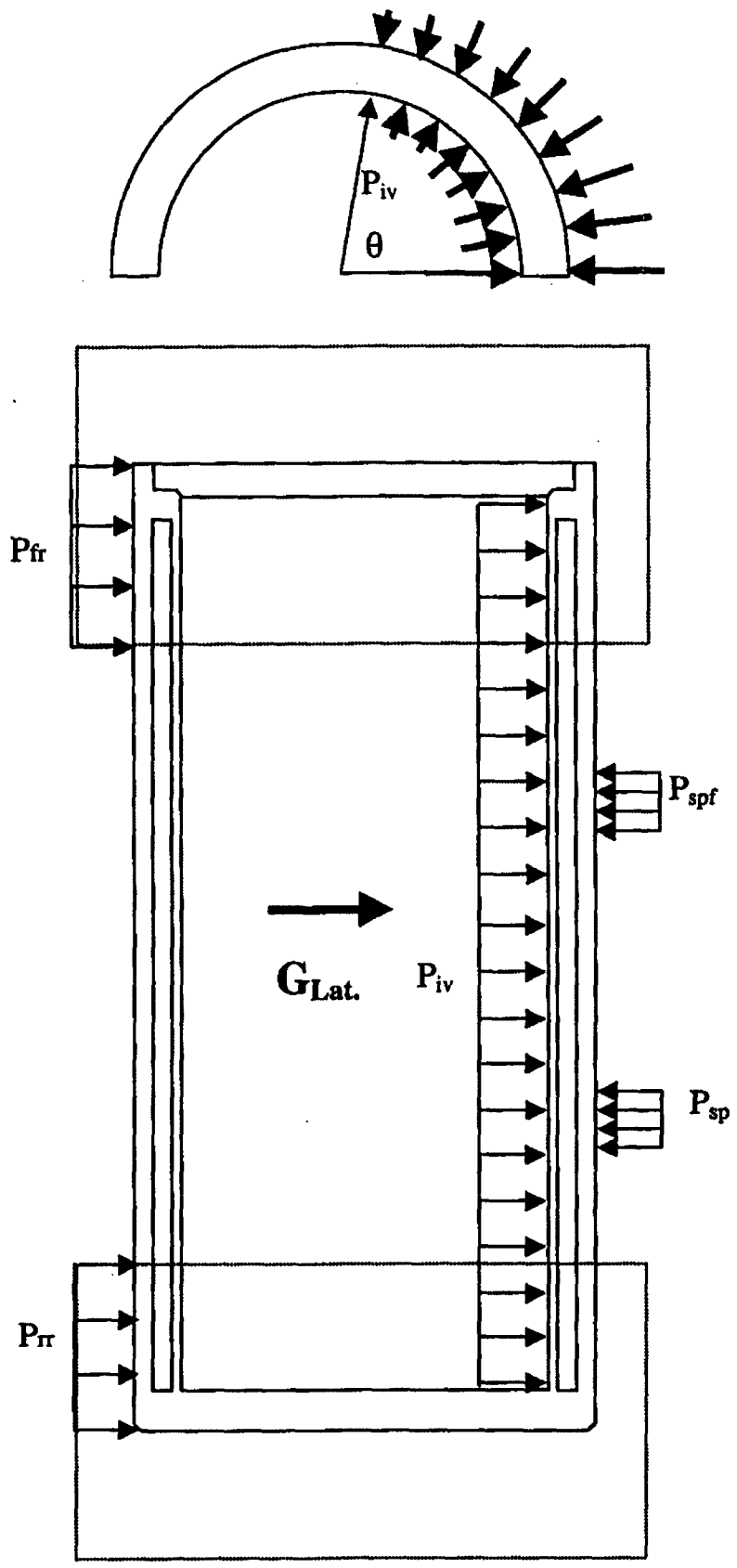
Figure 2.10.1-10: 1G Loading
