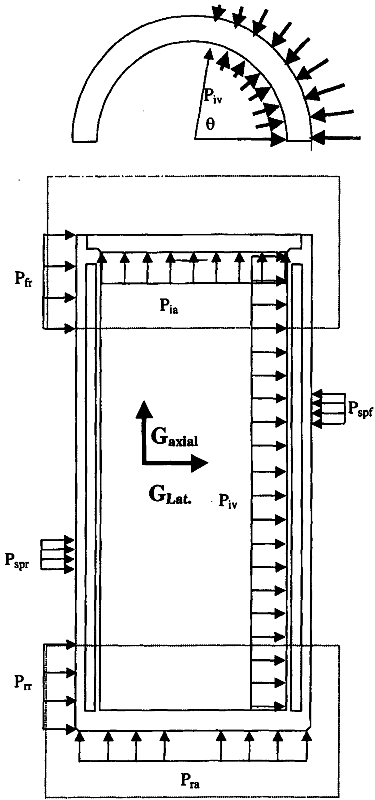
Figure 2.10.1-18: Tie-Down Loading
