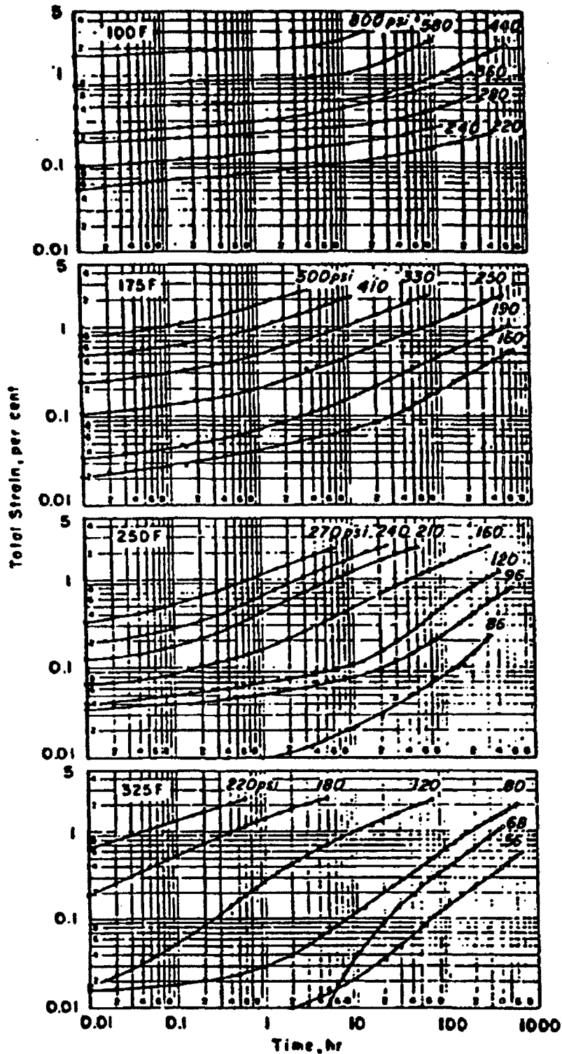
—Total Strain versus Creep Time for High-Purity Lead.
