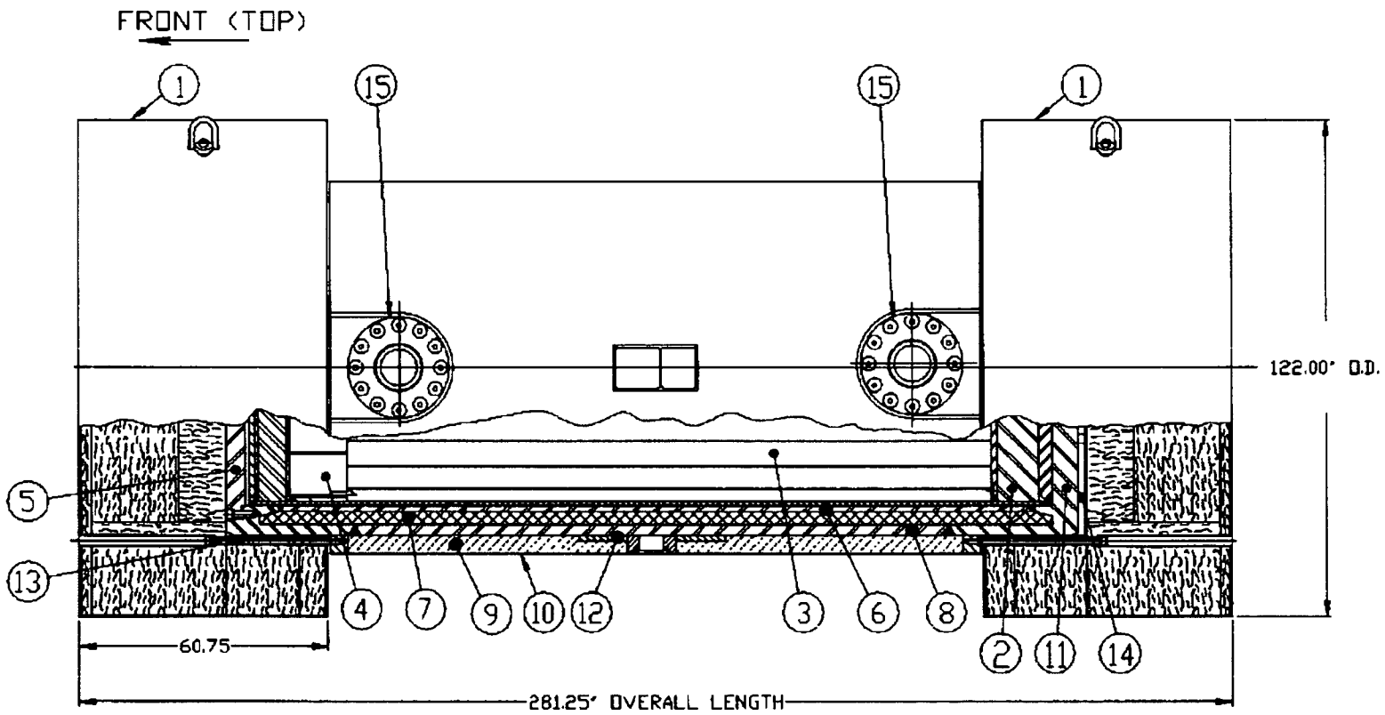
General Arrangement NUHOMS-MP197 Packaging
