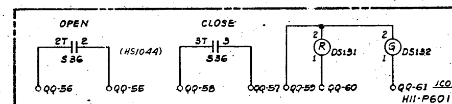
MAIN STEAM LINE DRAIN VALVE B21-F021 (MO/044) SH.2, FIG. 1 BECHTEL SCHEME B2209 (REF) (SEE DWG E-122, SH. 8)
