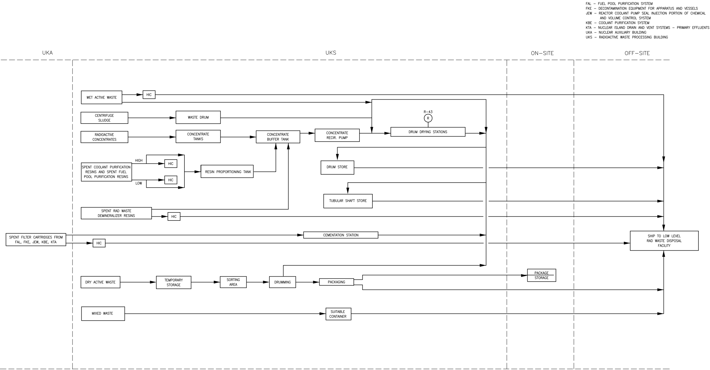
Figure 11.4-1—Solid Waste Management Flow Diagram
