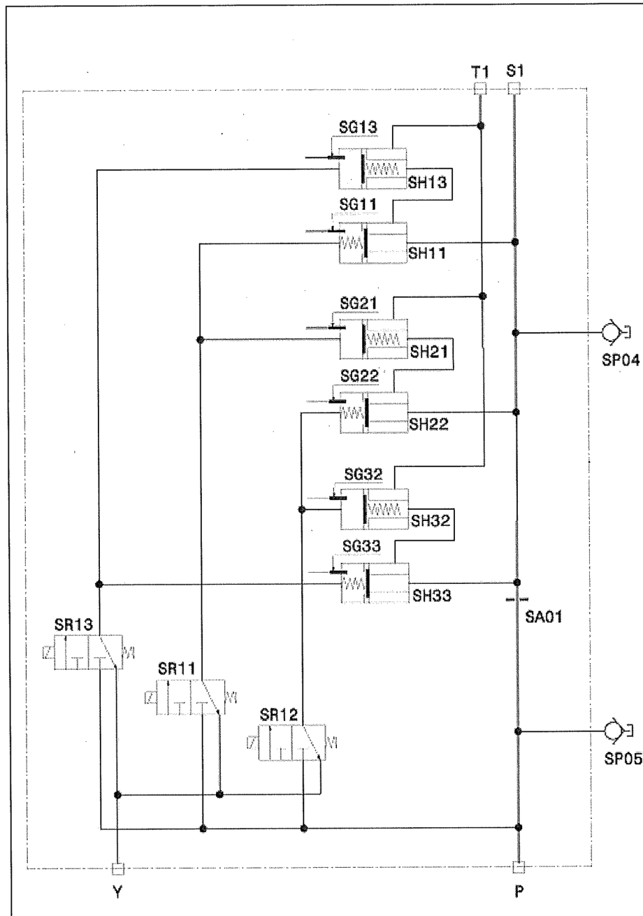
Figure 10.2-3—Turbine Trip Block Schematic
