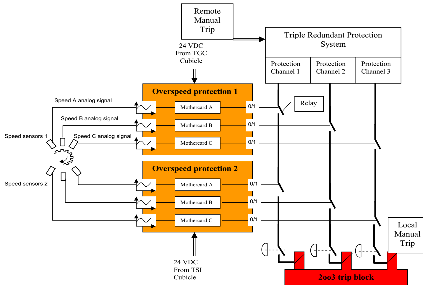
Figure 10.2-2—Overspeed Protection System Schematic
