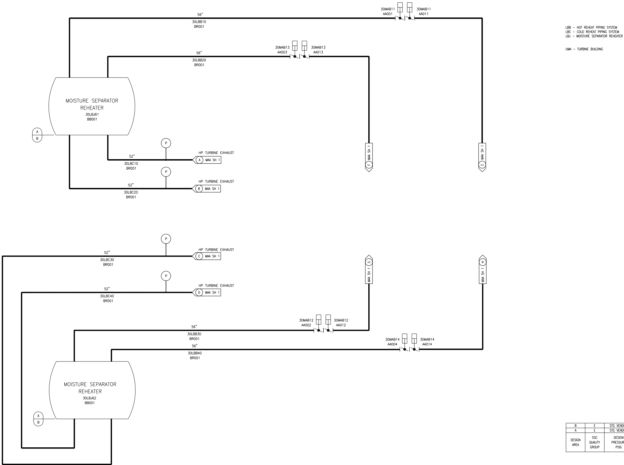
Figure 10.2-1—Turbine Generator System Sheet 2 of 2
