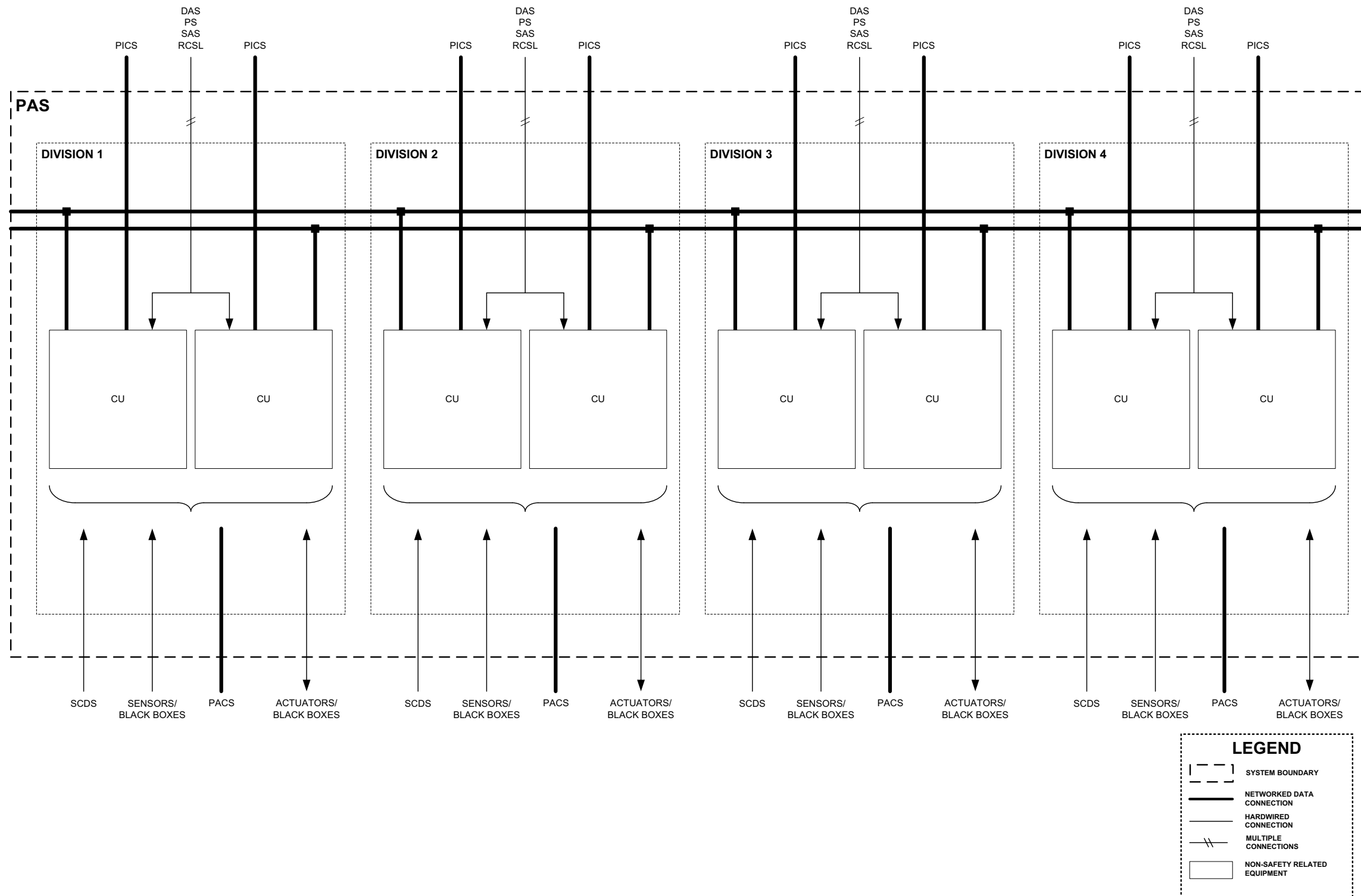
Figure 7.1-11—Process Automation System Architecture (Nuclear Island)
