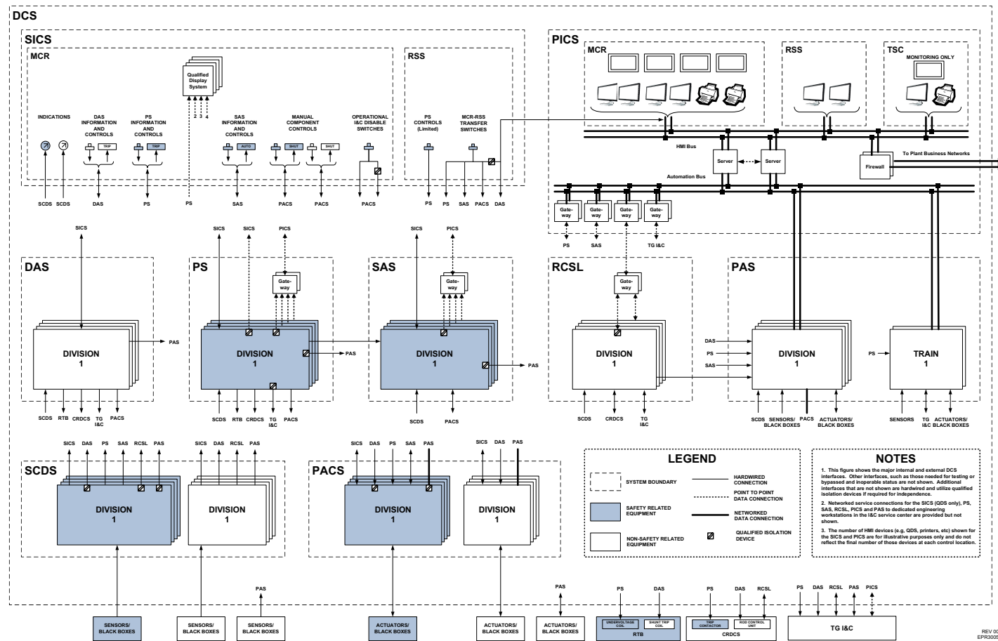
Figure 7.1-2—Distributed Control System Functional Architecture
