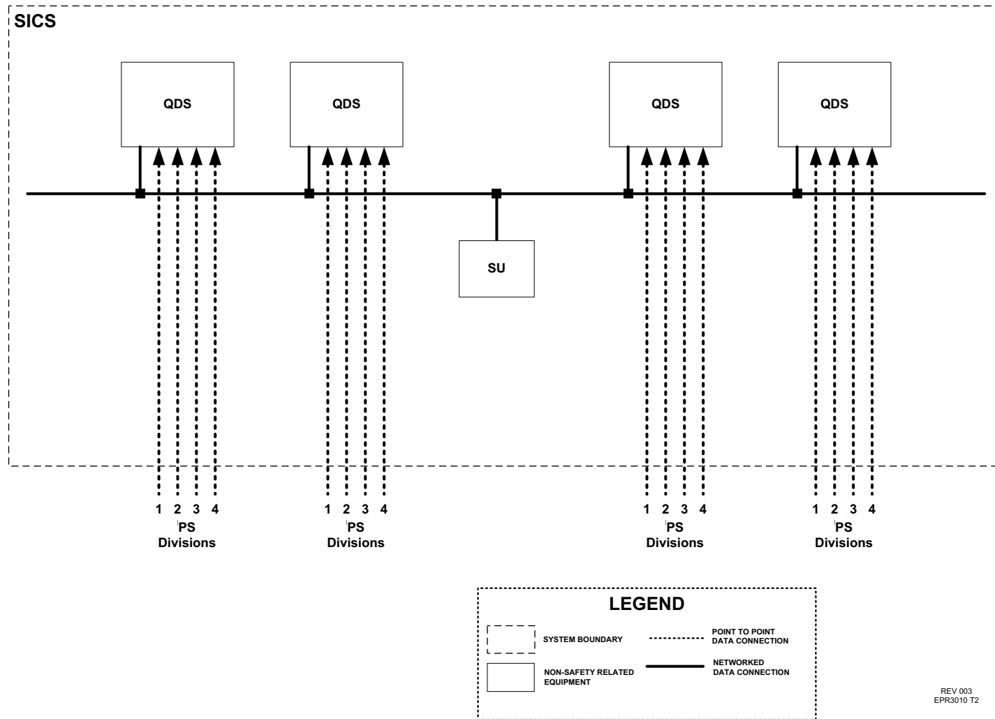
Figure 7.1-3—Safety Information and Control System Architecture (QDS Portion)
