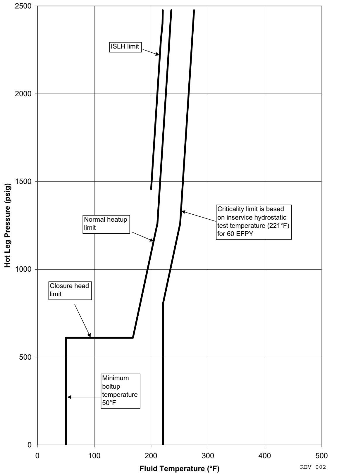
Figure 5.3-1—Reactor Coolant System Heatup Pressure-Temperature Curve
