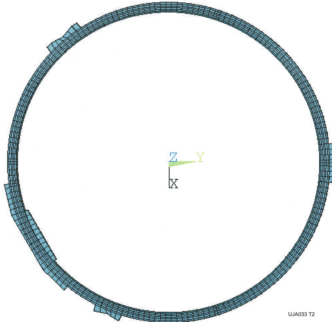
Figure 3E.1-19—Plan View Cut Through Critical Section
