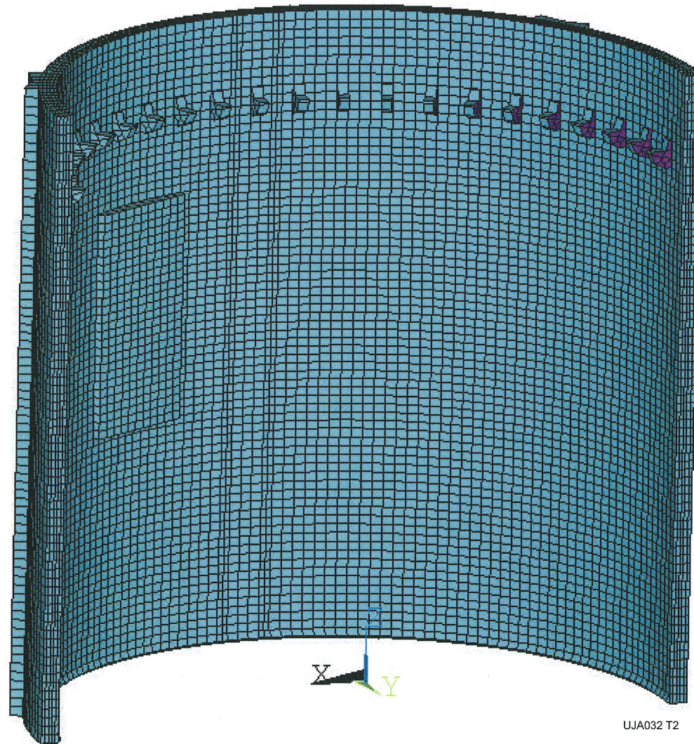
Figure 3E.1-18—Section View Cut Through Critical Section
