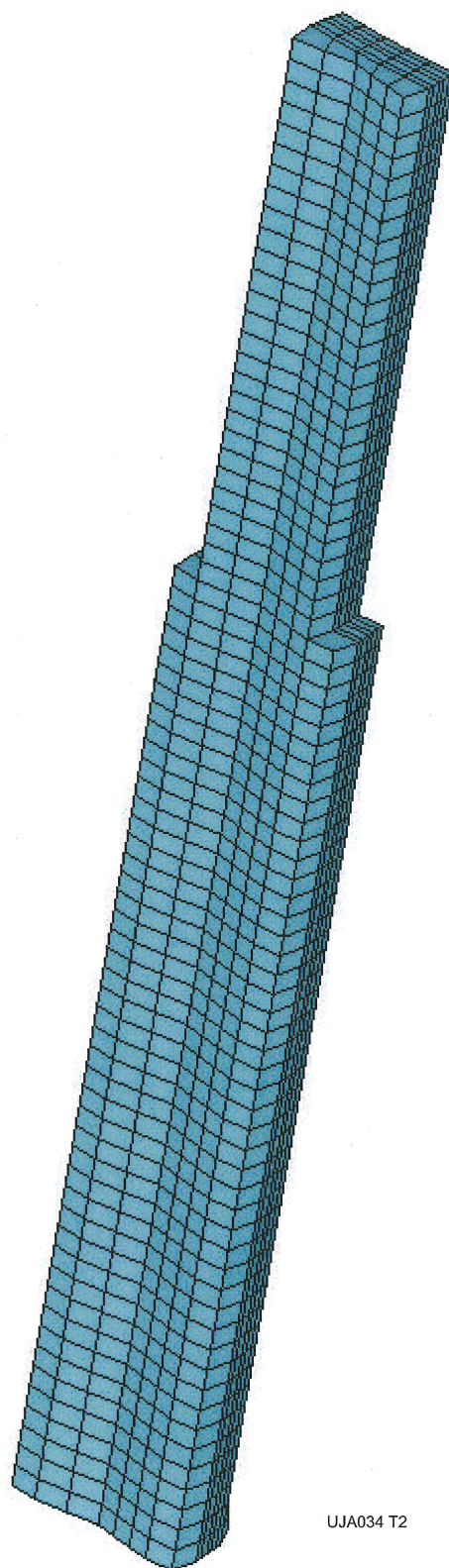
Figure 3E.1-20—Elevation View of Buttress 3
