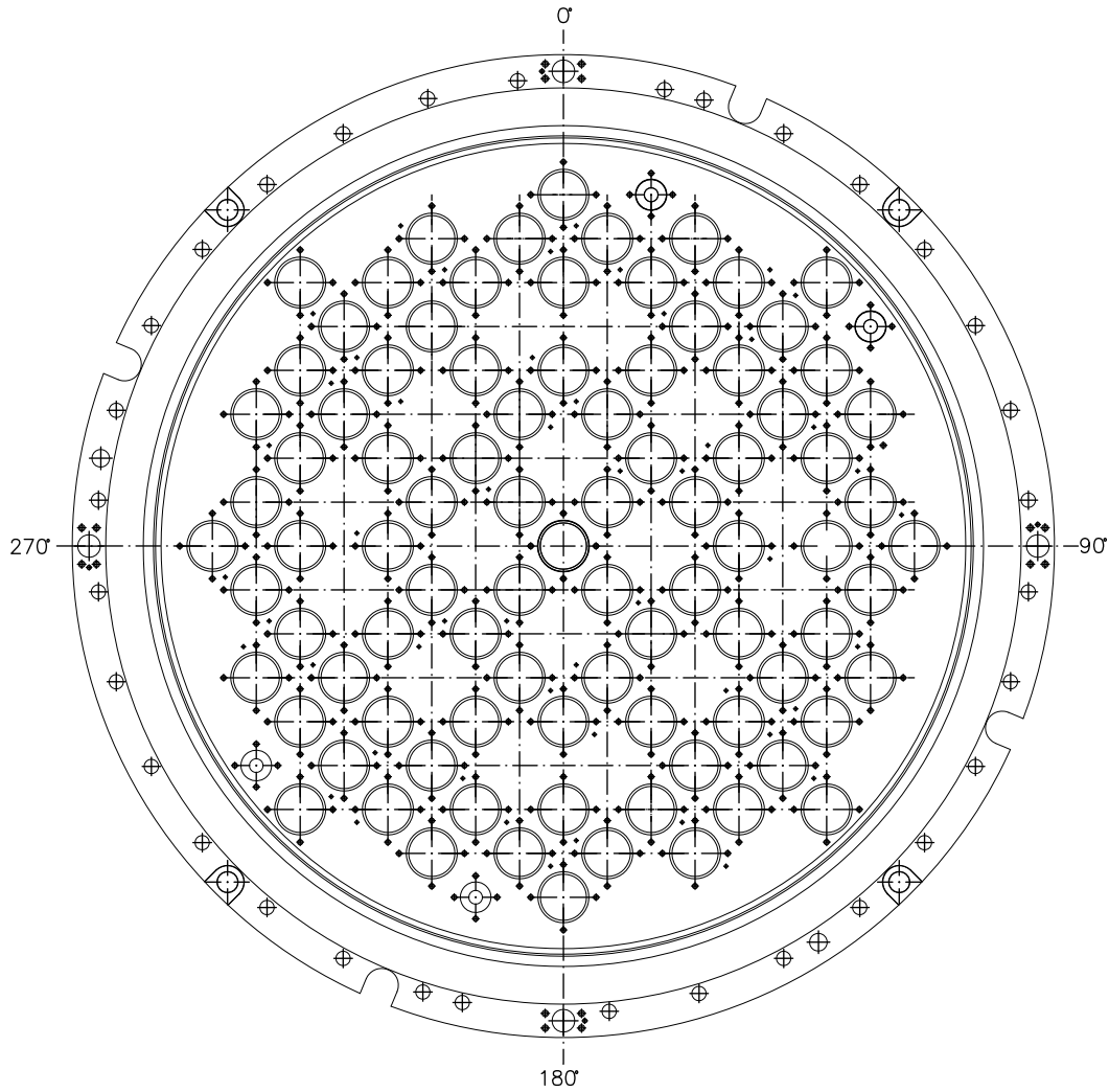
SECTION B-B UPPER SUPPORT PLATE
