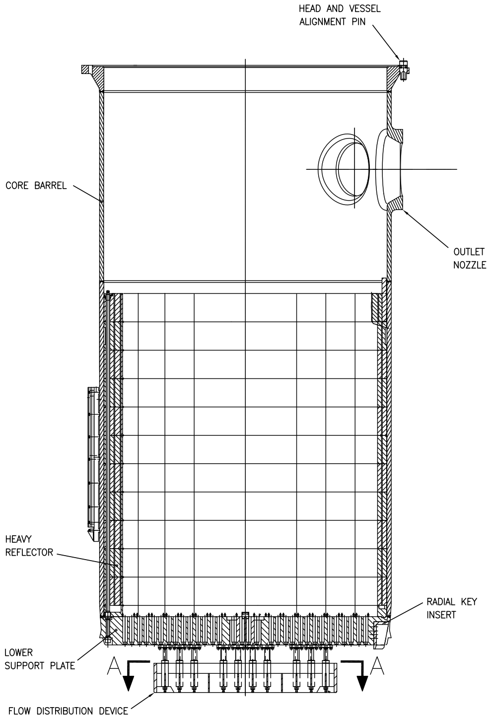
Figure 3.9.5-2—Lower Reactor Internals
