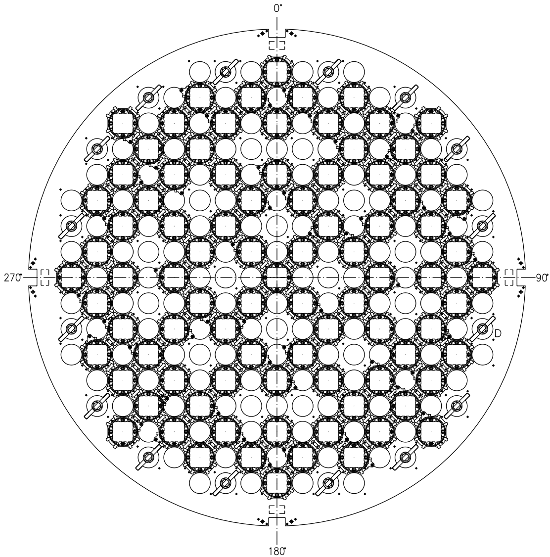
SECTION C-C UPPER CORE PLATE
