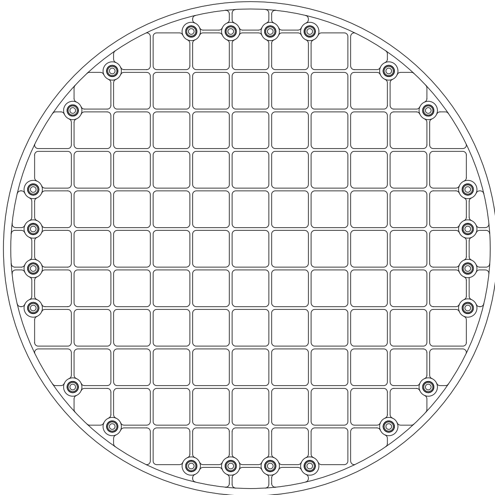
SECTION A-A FLOW DISTRIBUTION DEVICE
