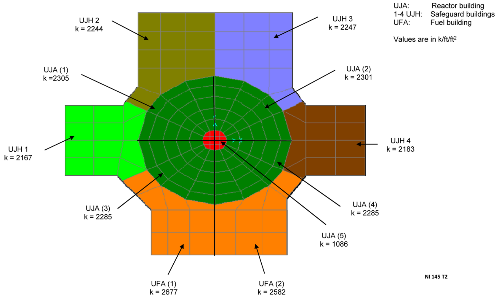
Figure 3.8-145—Foundation Modulus for High Frequency Soil Cases
