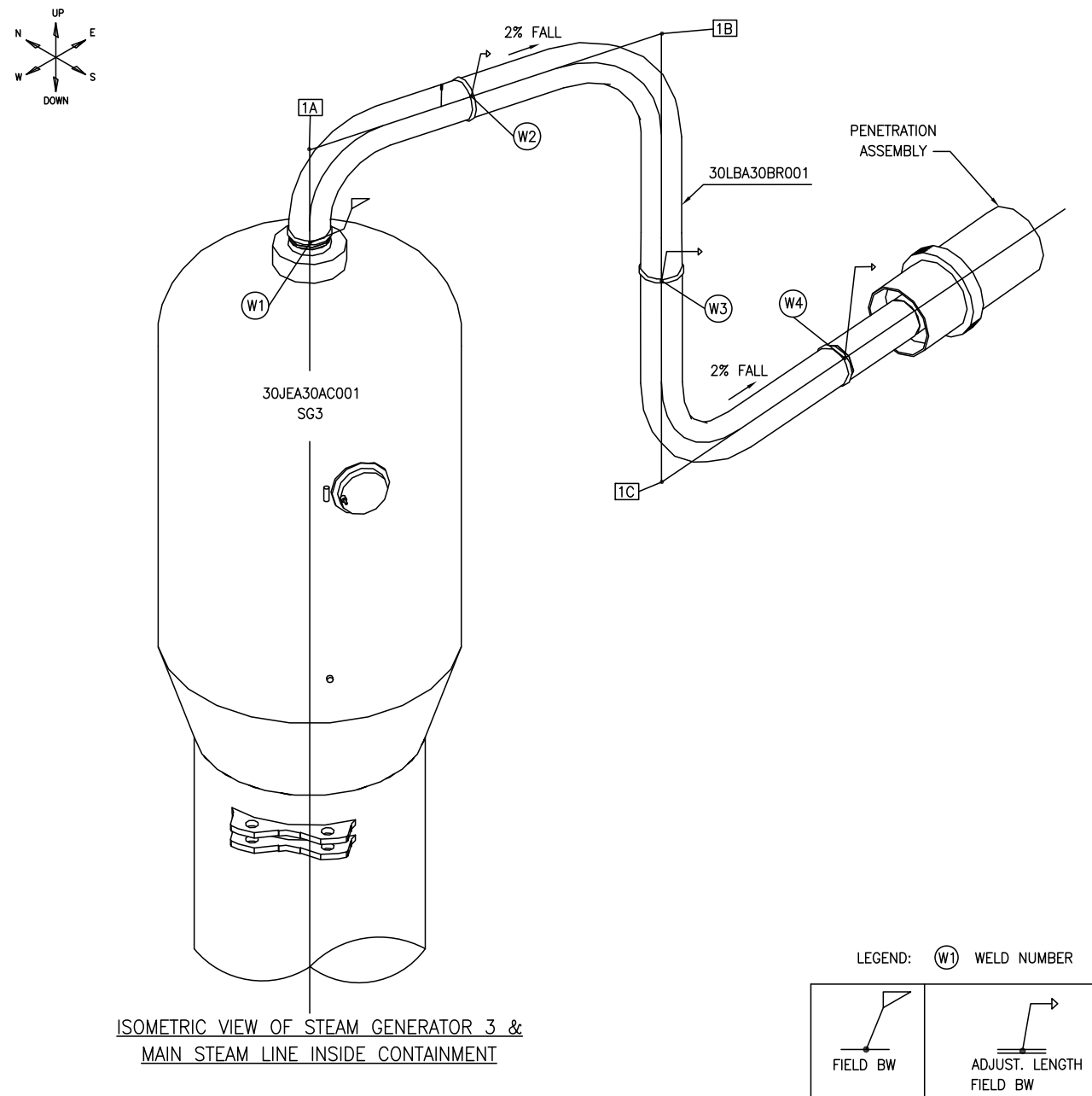
Figure 3.6.3-4—Isometric View of the Main Steam Line
