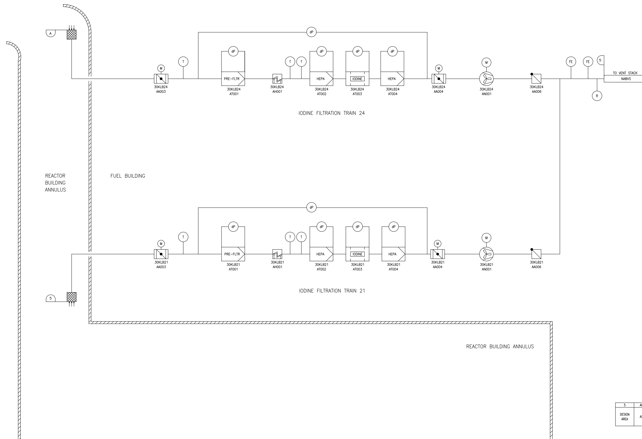
Figure 2.6.3-2—Annulus Ventilation System Accident Filtration Train Functional Arrangement
