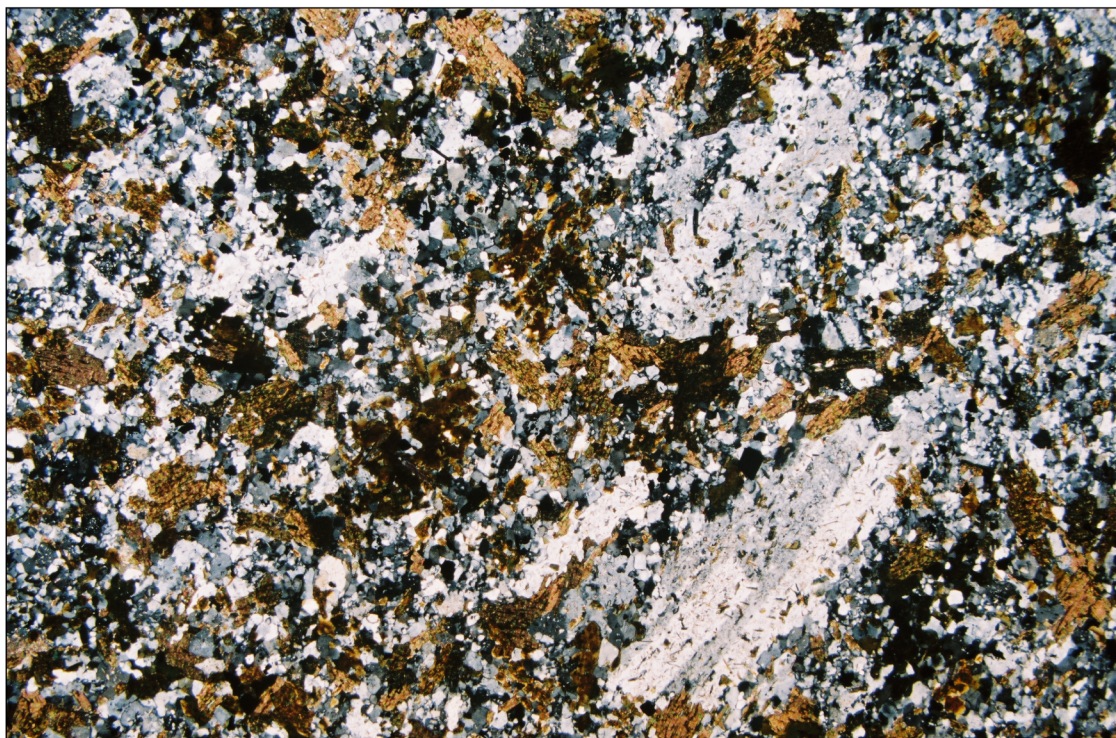
Meta-dacite Porphyry showing typical appearance of porphyritic texture in thin section
