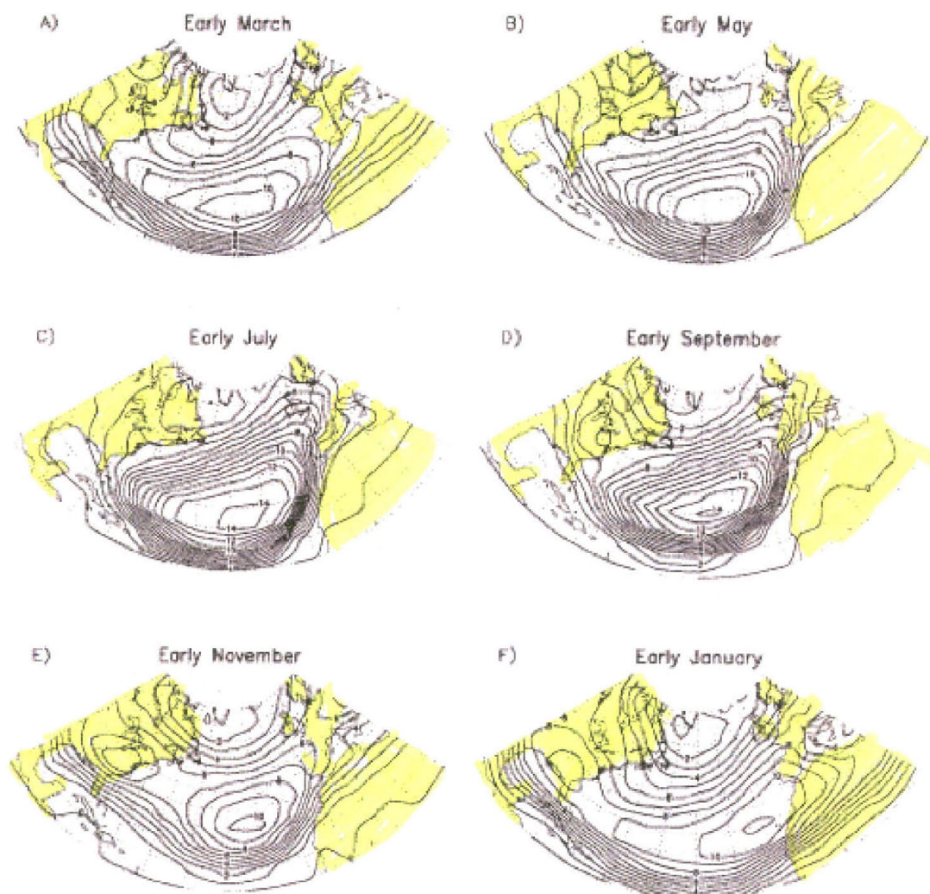
FIG. 2. Average number of days with sea level pressure \leq 1010 mb in the first half of (a) March, (b) May, (c) July, (d) September, (e) November, and (f) January.
