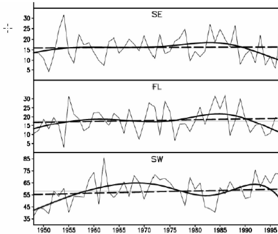
Air Stagnation Trend (Positive)
