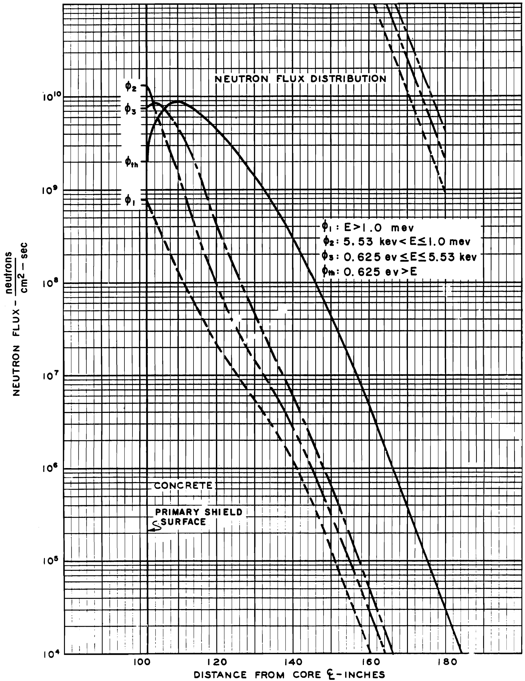
NEUTRON FLUX DISTRIBUTION
