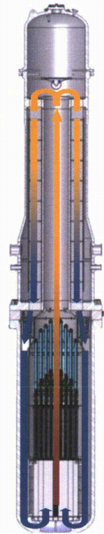
Primary Loop
