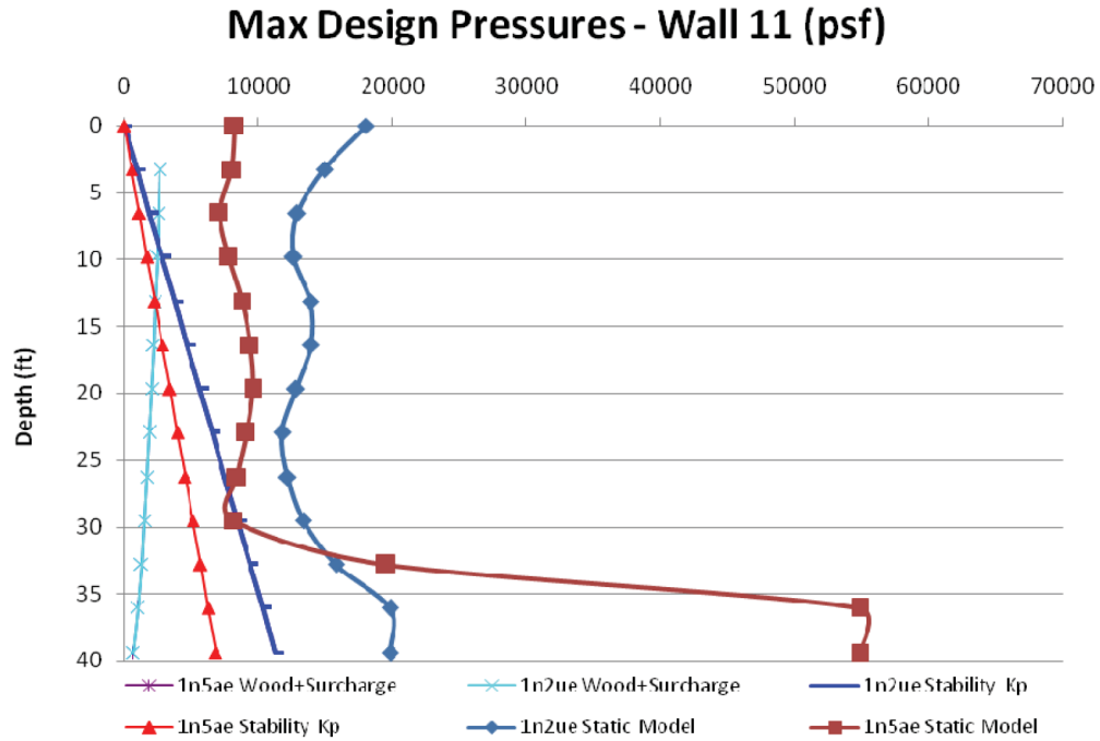
Figure 03.08.05-28-29—Wall 11 - Soil 1n2ue and 1n5ae (Cracked Concrete)
