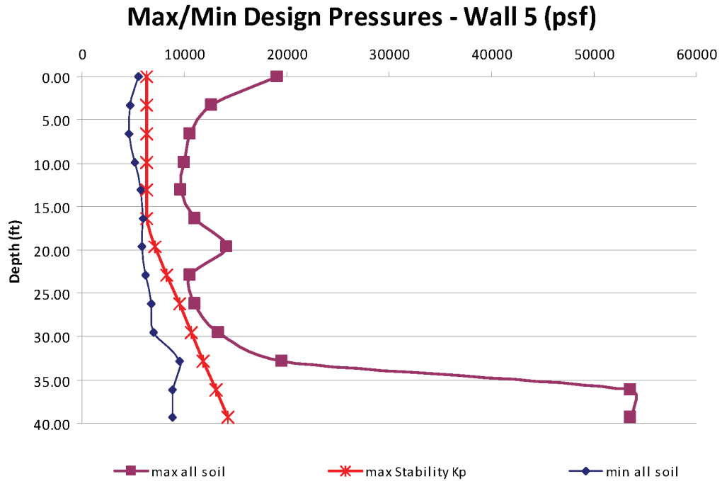
Figure 03.08.05-28-35—Wall 5 – Upper/Lower Bound of all Soil Cases (Cracked Concrete)
