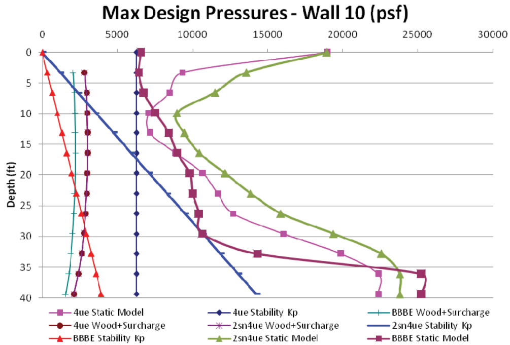
Figure 03.08.05-28-27—Wall 10 - Soil 2sn4ue, 4ue and hfbe (Cracked Concrete)
