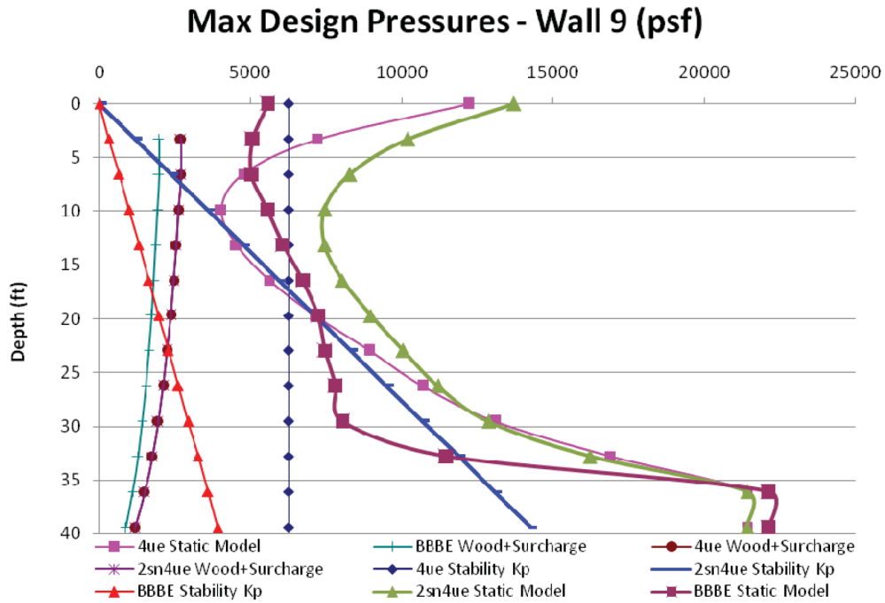
Figure 03.08.05-28-24—Wall 9 - Soil 2sn4ue, 4ue and hfbe (Cracked Concrete)
