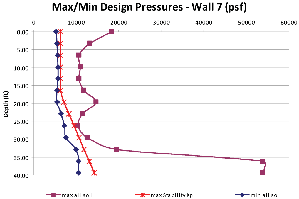
Figure 03.08.05-28-37—Wall 7 – Upper/Lower Bound of all Soil Cases (Cracked Concrete)
