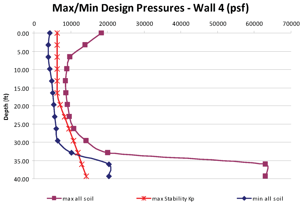
Figure 03.08.05-28-34—Wall 4 – Upper/Lower Bound of all Soil Cases (Cracked Concrete)
