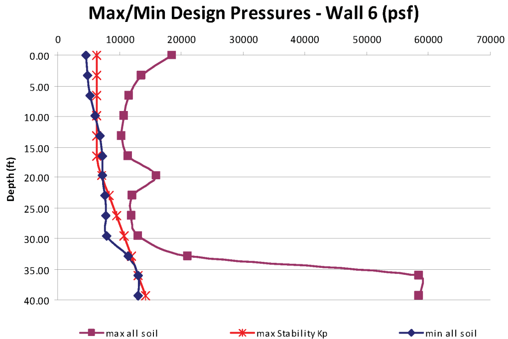
Figure 03.08.05-28-36—Wall 6 – Upper/Lower Bound of all Soil Cases (Cracked Concrete)
