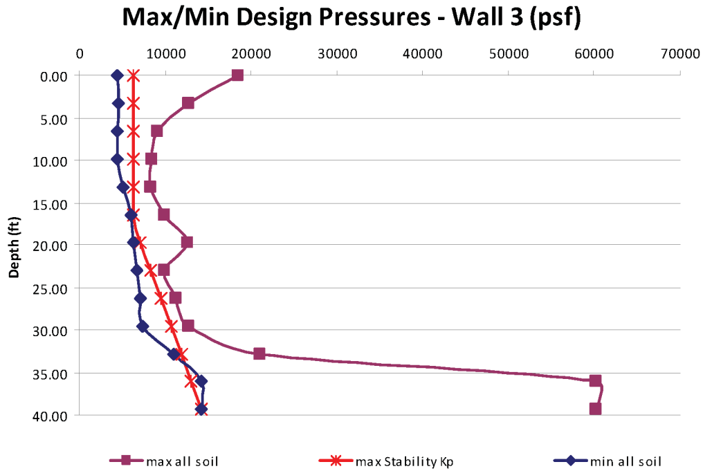
Figure 03.08.05-28-33—Wall 3 – Upper/Lower Bound of all Soil Cases (Cracked Concrete)
