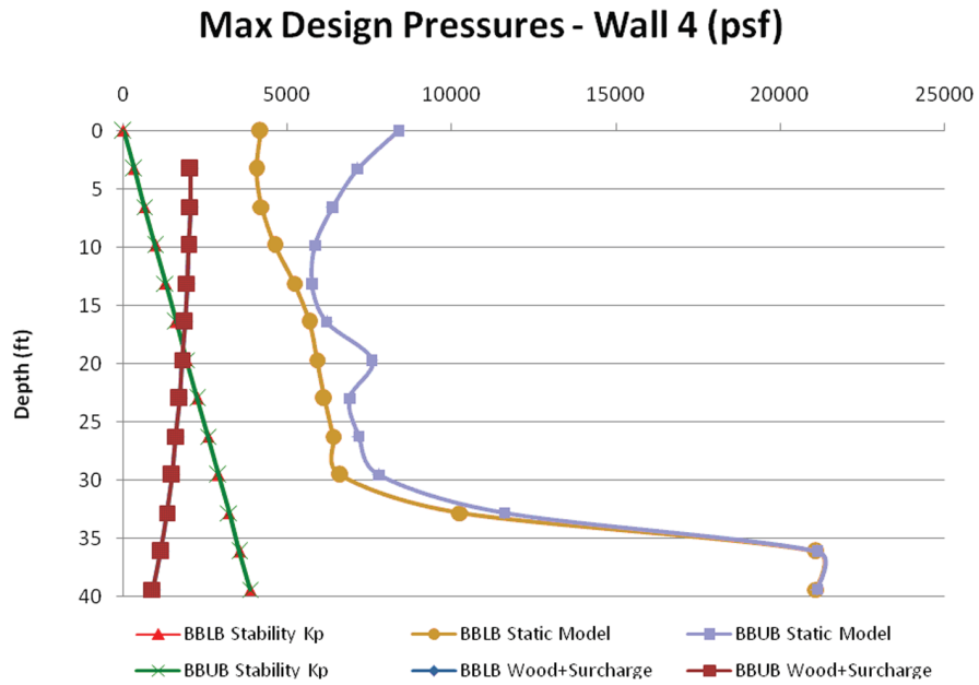
Figure 03.08.05-28-51—Wall 4 - Soil hflb and hfub (Uncracked Concrete)
