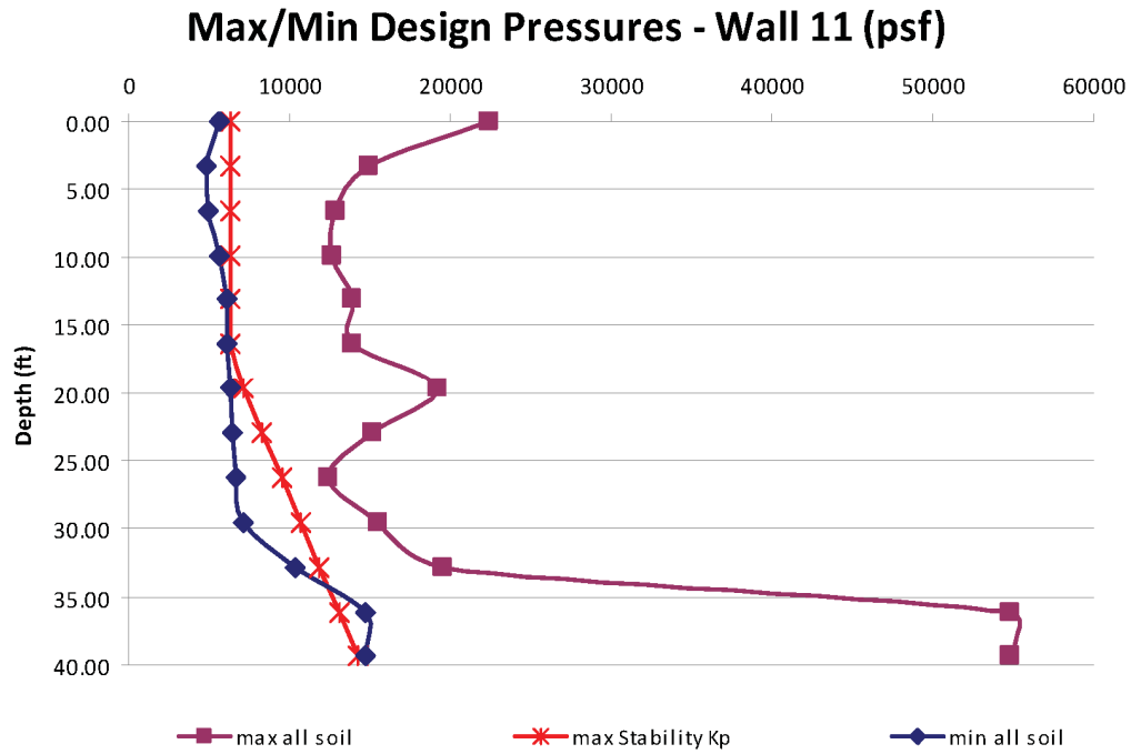
Figure 03.08.05-28-41—Wall 11 – Upper/Lower Bound of all Soil Cases (Cracked Concrete)
