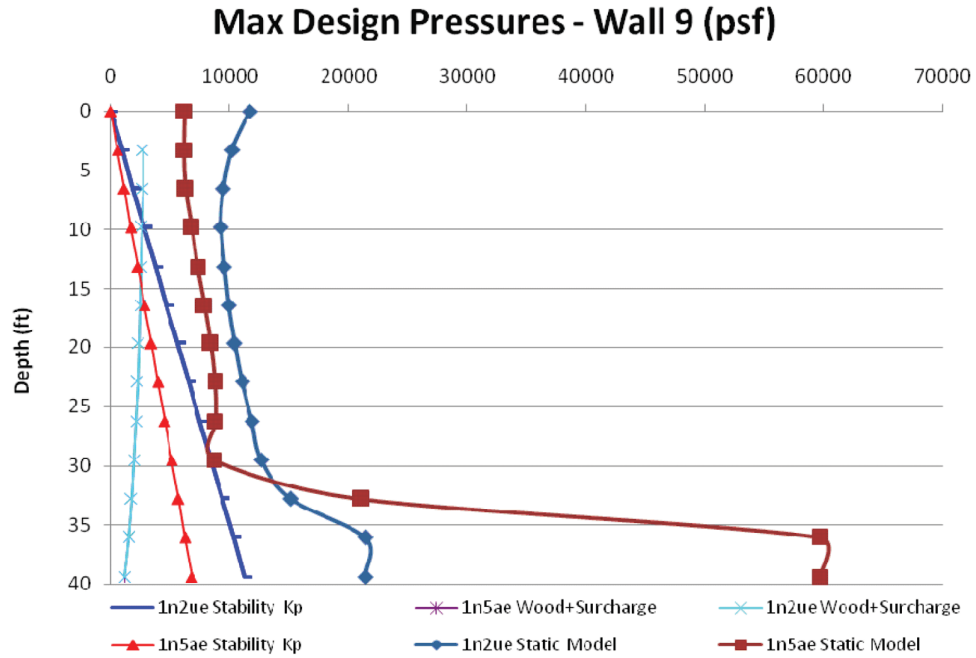
Figure 03.08.05-28-23—Wall 9 - Soil 1n2ue and 1n5ae (Cracked Concrete)
