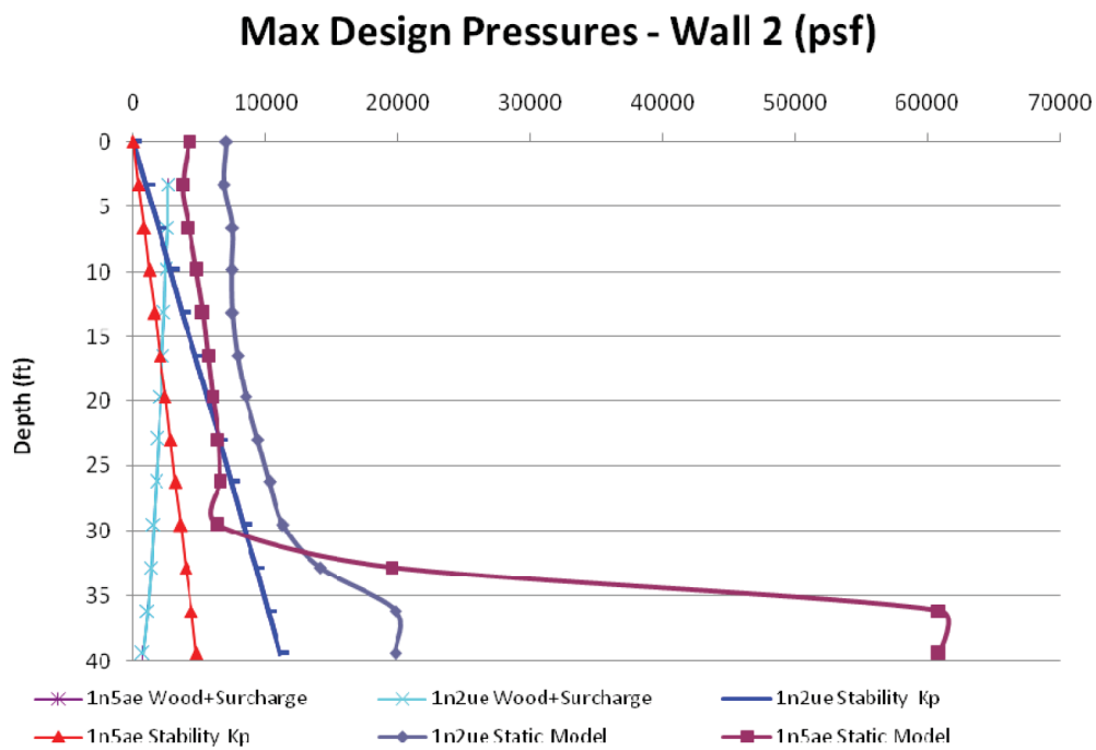
Figure 03.08.05-28-43—Wall 2 - Soil 1n2ue and 1n5ae (Uncracked Concrete)
