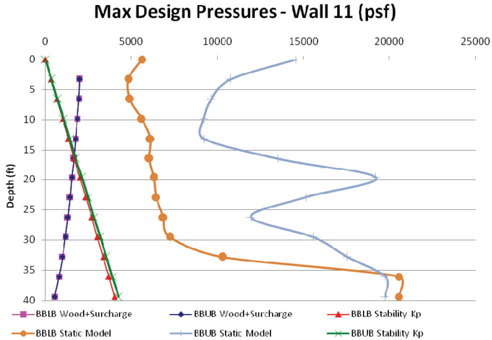
Figure 03.08.05-28-31—Wall 11 - Soil hflb and hfub (Cracked Concrete)
