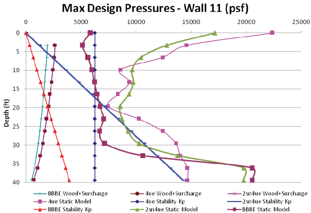
Figure 03.08.05-28-30—Wall 11 - Soil 2sn4ue, 4ue and hfbe (Cracked Concrete)
