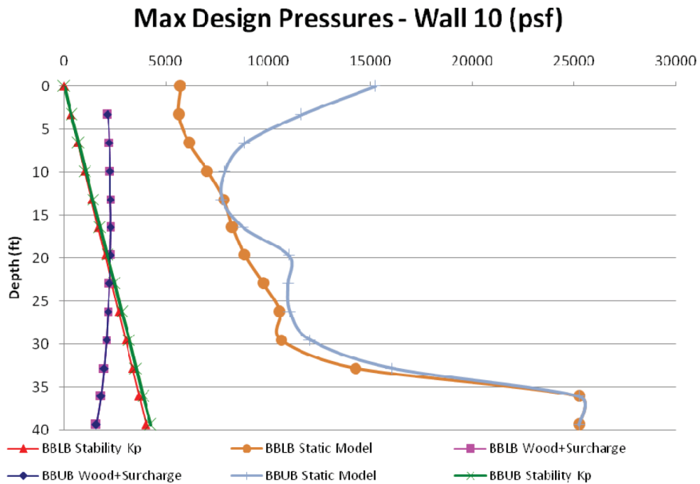
Figure 03.08.05-28-28—Wall 10 - Soil hf1b and hfub (Cracked Concrete)
