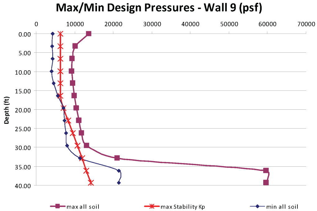
Figure 03.08.05-28-39—Wall 9 – Upper/Lower Bound of all Soil Cases (Cracked Concrete)
