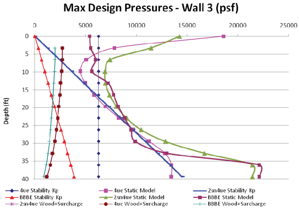
Figure 03.08.05-28-47—Wall 3 - Soil 2sn4ue, 4ue and hfbe (Uncracked Concrete)
