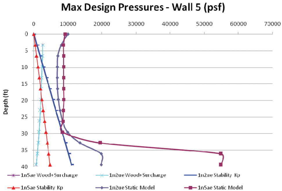
Figure 03.08.05-28-52—Wall 5 - Soil 1n2ue and 1n5ae (Uncracked Concrete)
