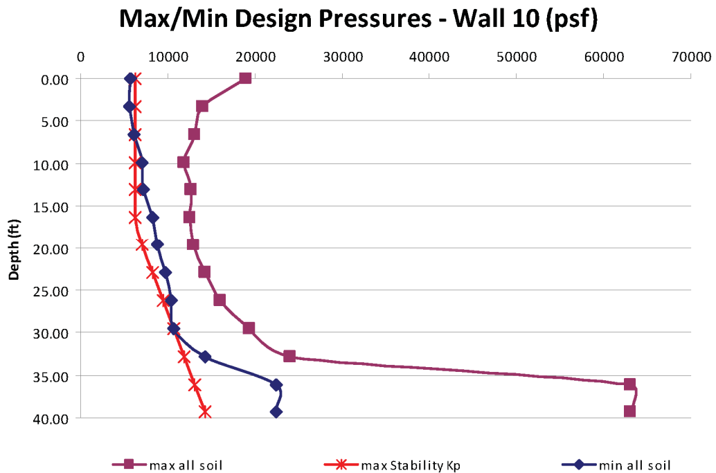
Figure 03.08.05-28-40—Wall 10 – Upper/Lower Bound of all Soil Cases (Cracked Concrete)
