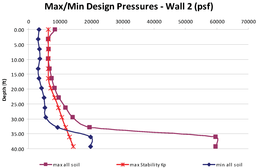
Figure 03.08.05-28-32—Wall 2 – Upper/Lower Bound of all Soil Cases (Cracked Concrete)
