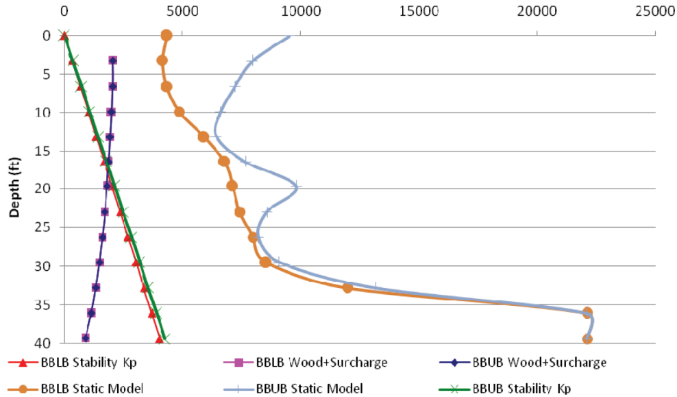
Figure 03.08.05-28-25—Wall 9 - Soil hflb and hfub (Cracked Concrete) Max Design Pressures - Wall 9 (psf)
