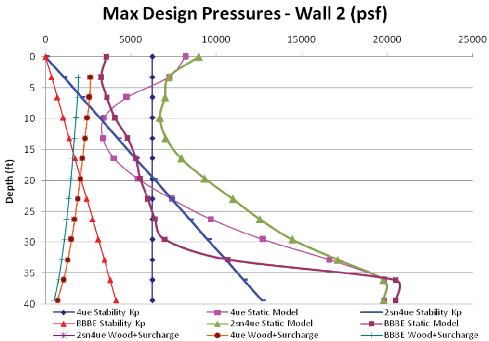
Figure 03.08.05-28-44—Wall 2 - Soil 2sn4ue, 4ue and hfbe (Uncracked Concrete)
