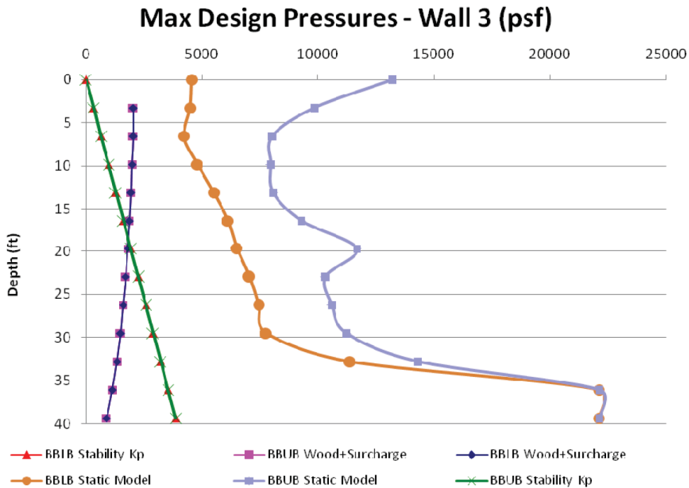
Figure 03.08.05-28-48—Wall 3 - Soil hf1b and hfub (Uncracked Concrete)
