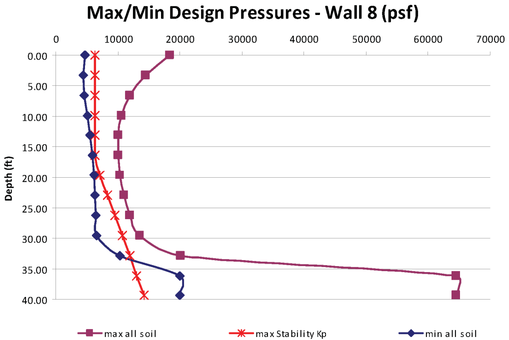
Figure 03.08.05-28-38—Wall 8 – Upper/Lower Bound of all Soil Cases (Cracked Concrete)
