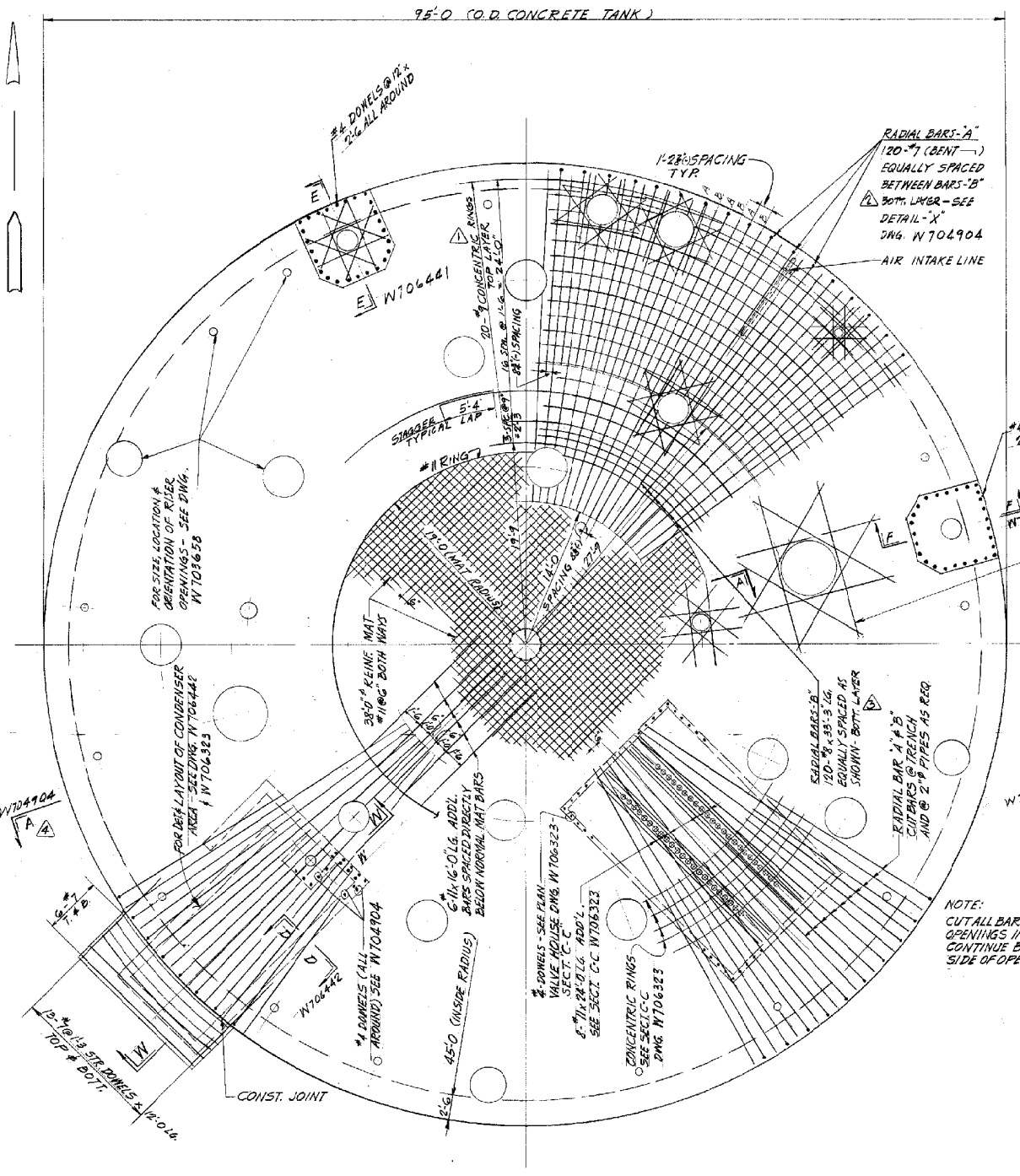
PLAN - TOP FACE REINFORCEMENT - TOP SLAB
