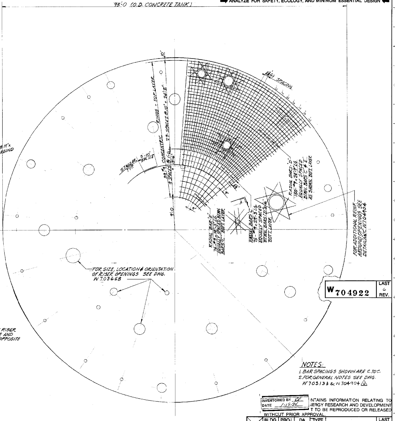
PLAN - BOT. FACE REINFORCEMENT - TOP SLAB
