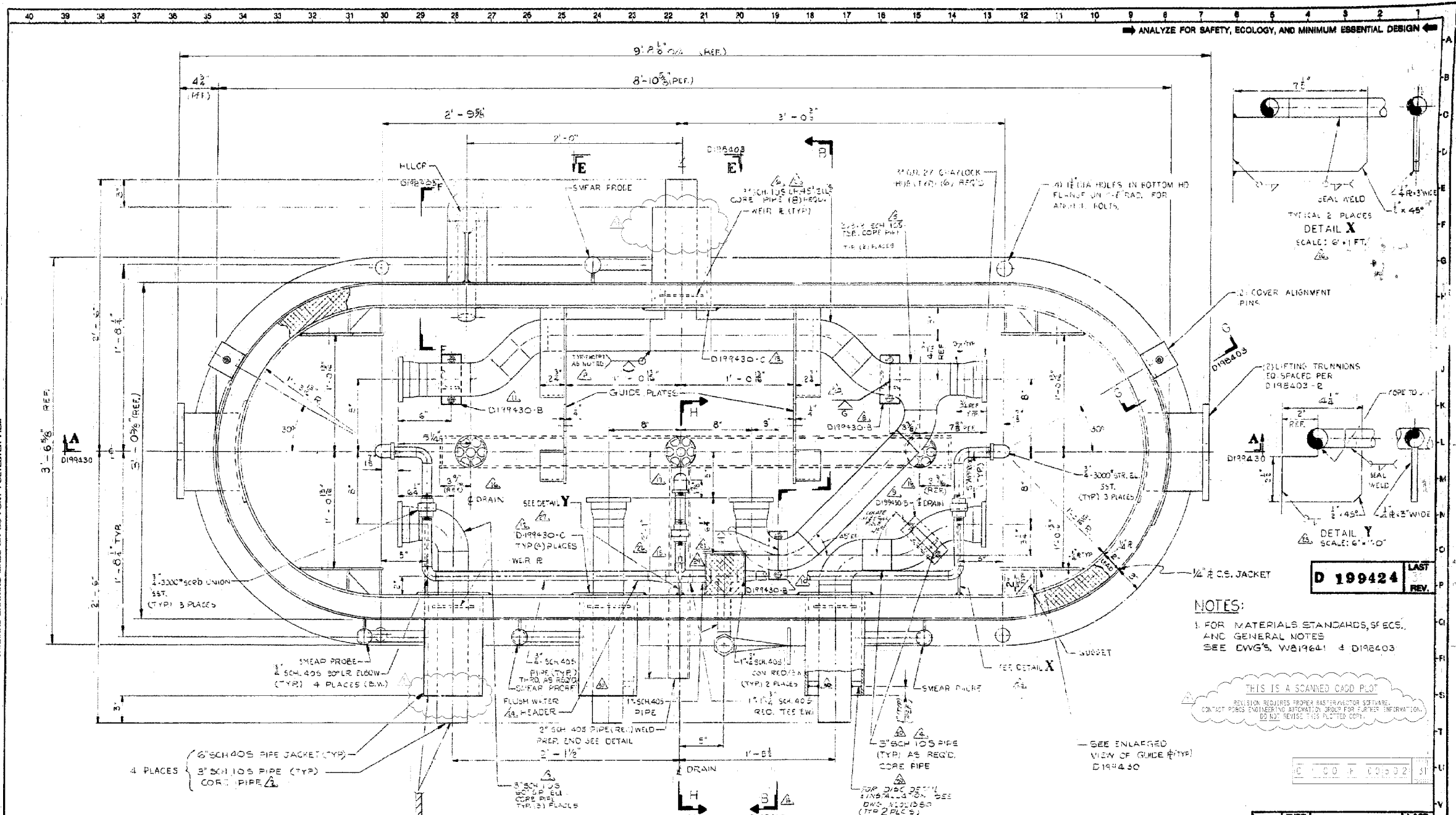
PLAN COVER & PLUGS NOT SHOWN D199424-A WT OF BOX APPROX. 9500 LBS.
