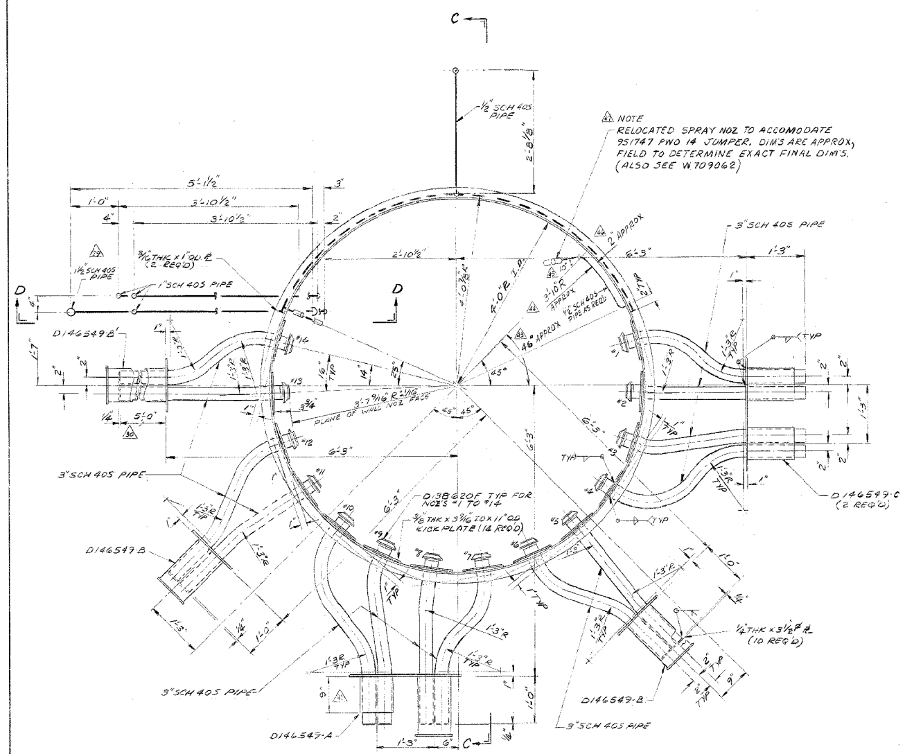
PLAN A-A MATERIAL: ST 304L (unless noted) 146352A
